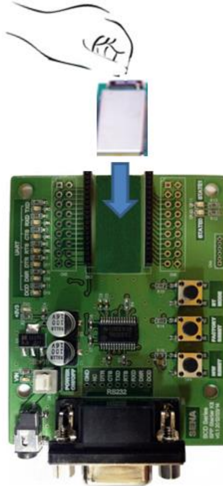
Figure 2-2 Connecting IW05 to Development Board
