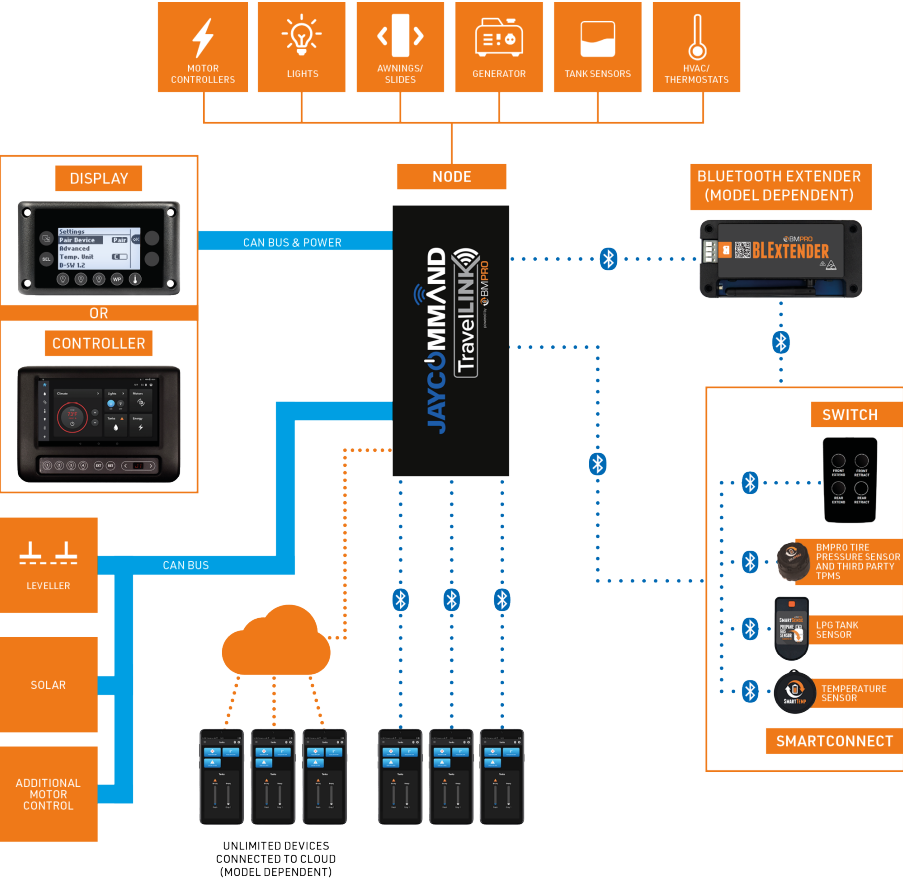
FIGURE 1: System Diagram
