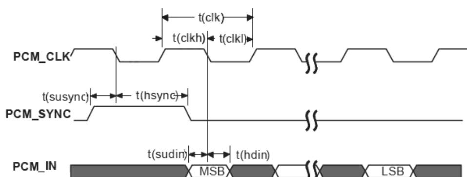
Figure 235: PCM_SYNC timing
