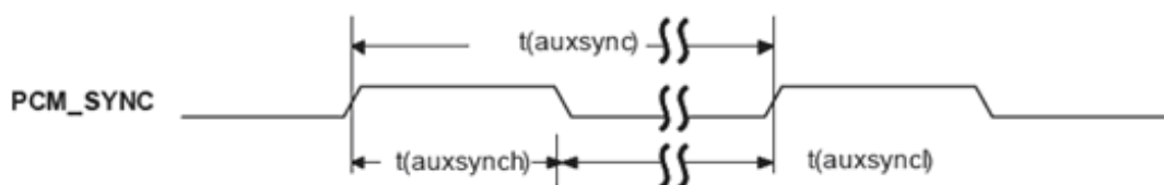
Figure 235: PCM_SYNC timing
