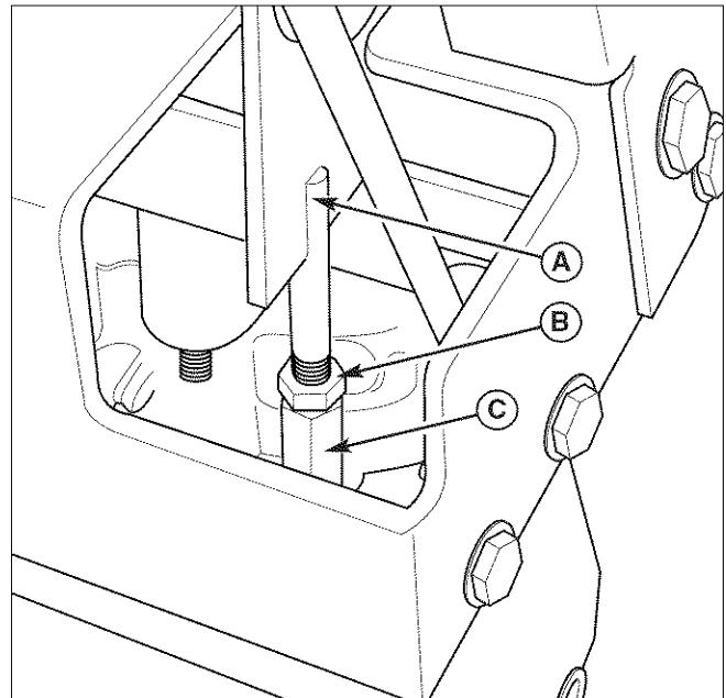
Figure 30. Adjusting the Speed of the Faster Wheel (RH side shown)
