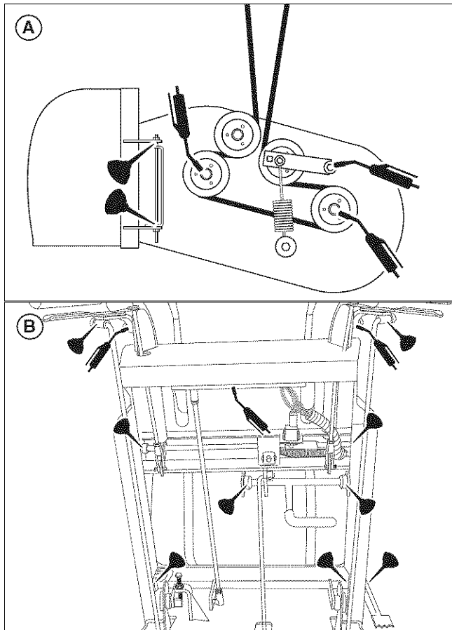
Figure 19. Lubrication Points
