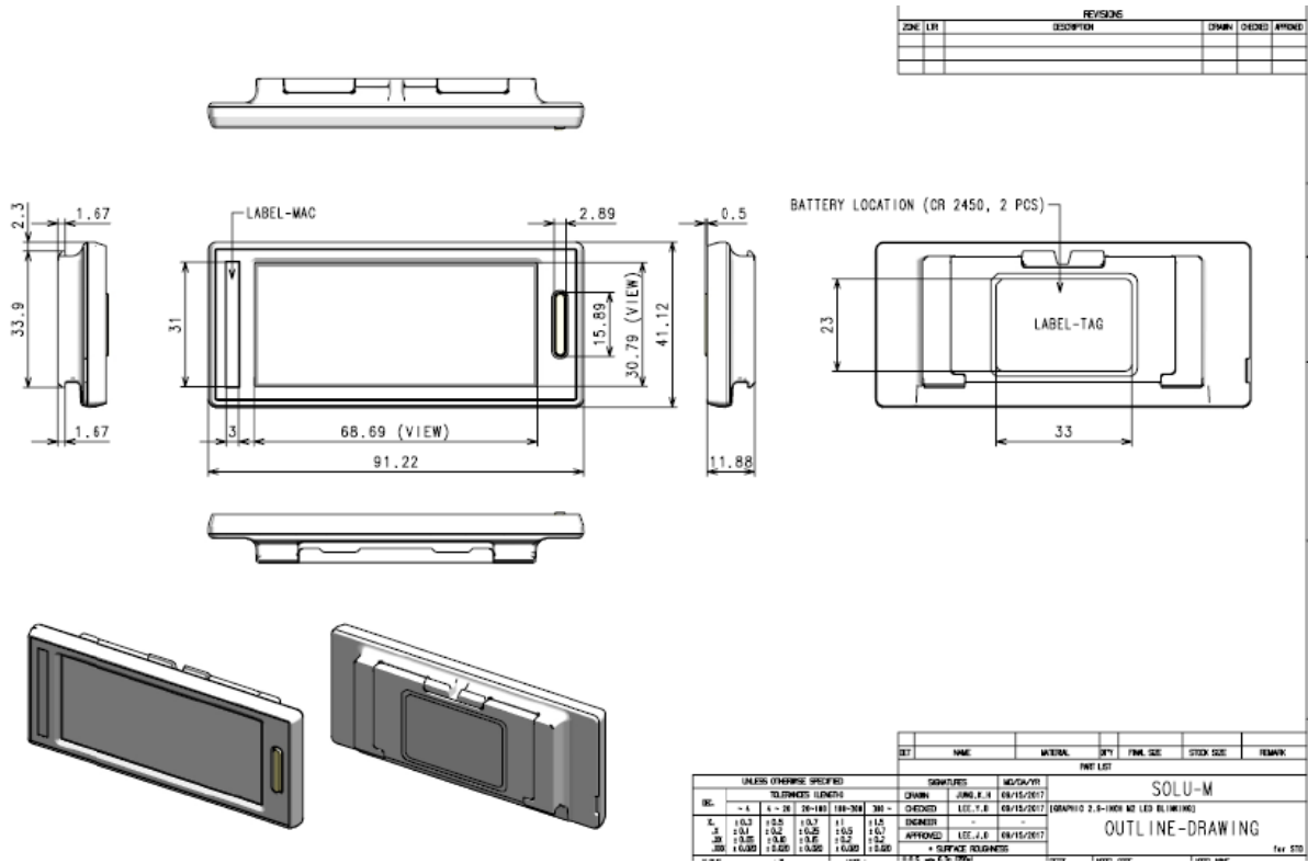
Figure 5. 2.9"Mechanical Dimension
