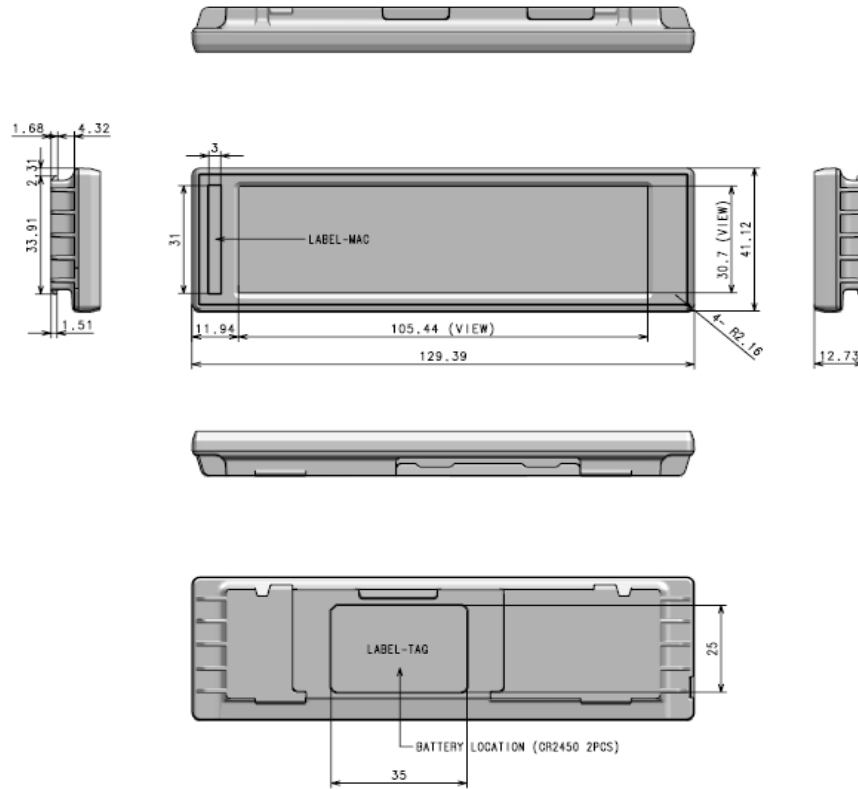
Figure 3 Mechanical Dimension
