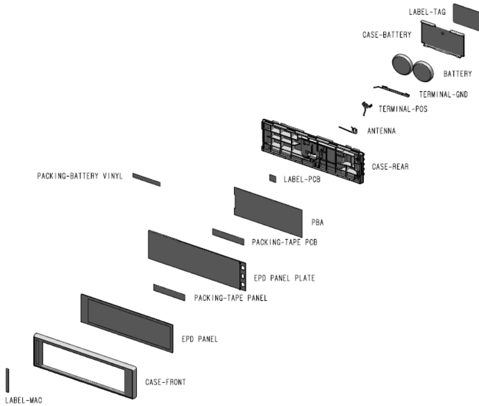
Figure 4 Exploded View
