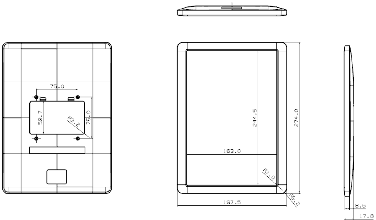
Figure 3. Mechanical Dimension
