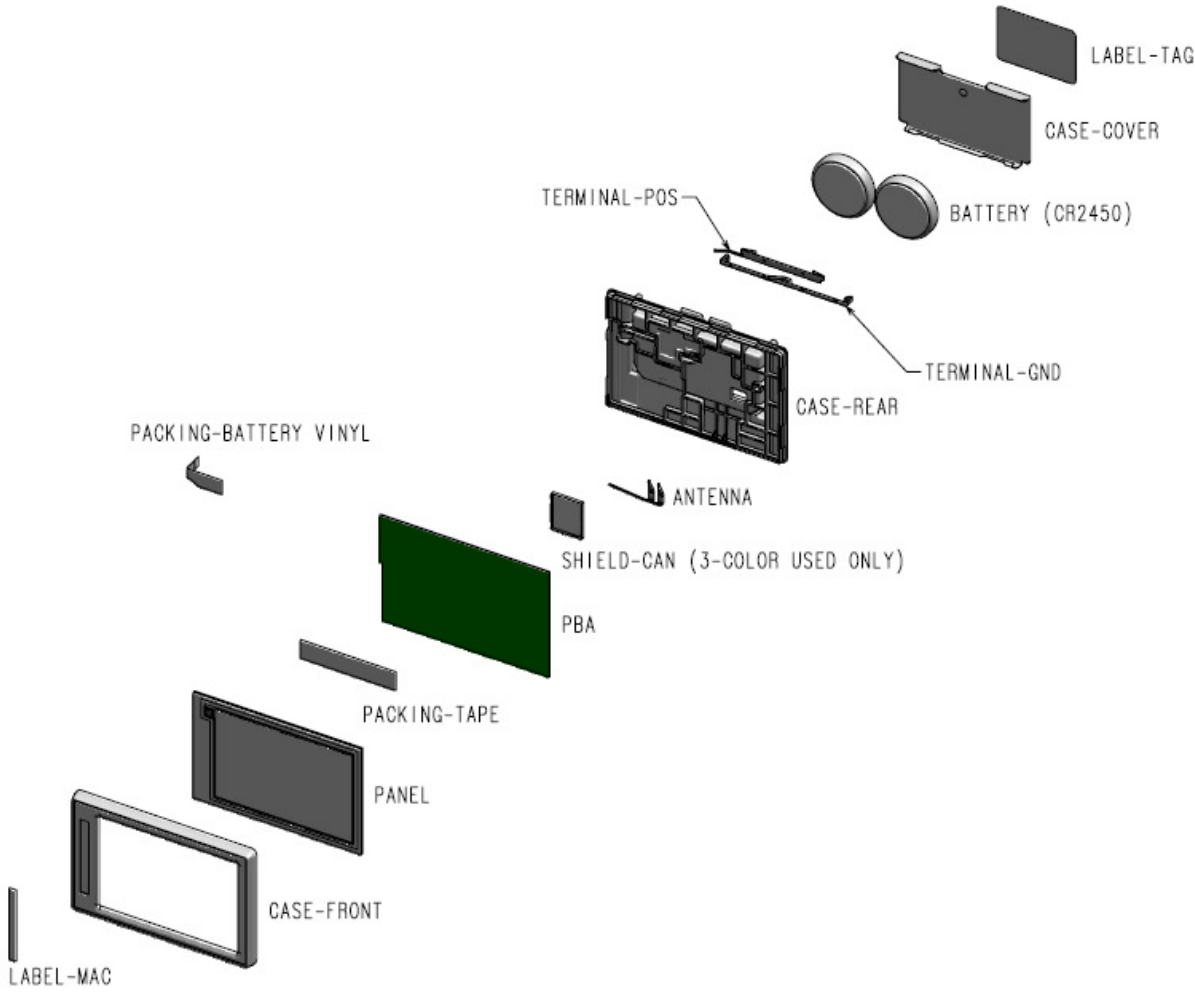
Figure 4 Exploded View
