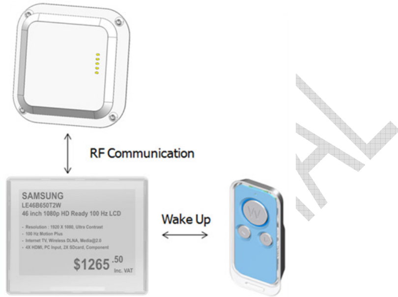
Figure 6 Operation Test
