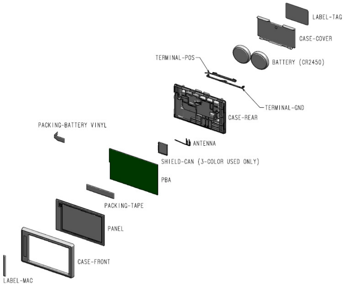
Figure 4 Exploded View
