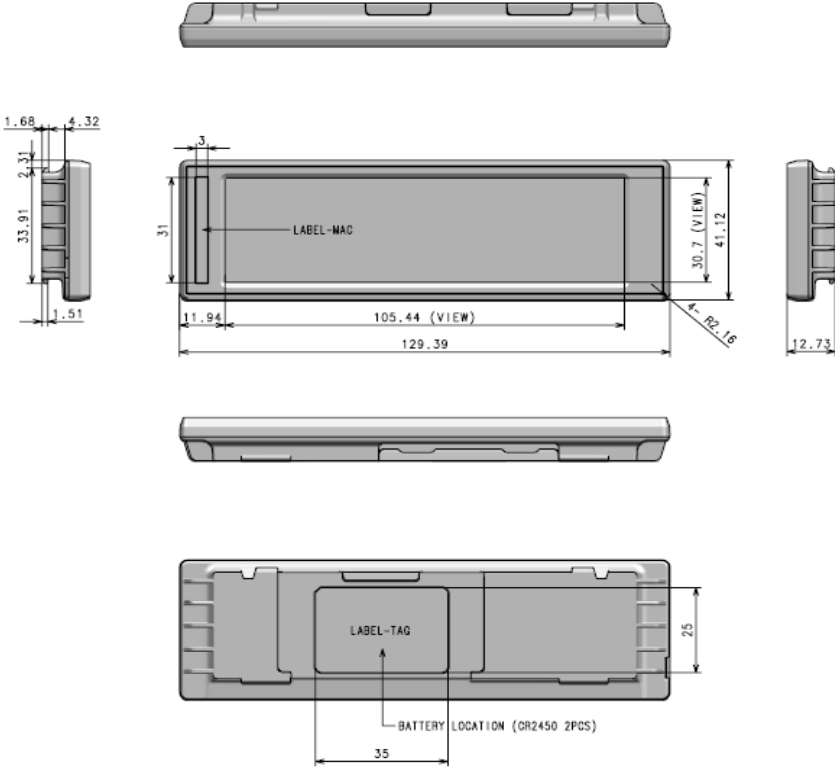
Figure 3 Mechanical Dimension
