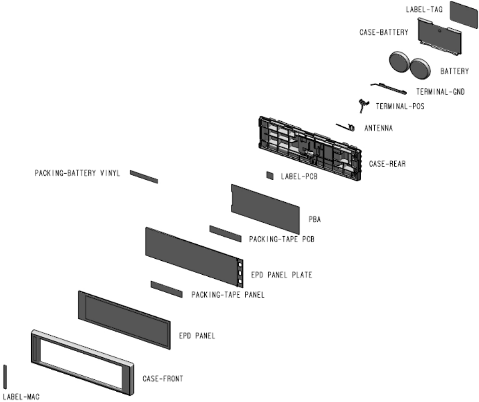
Figure 4 Exploded View
