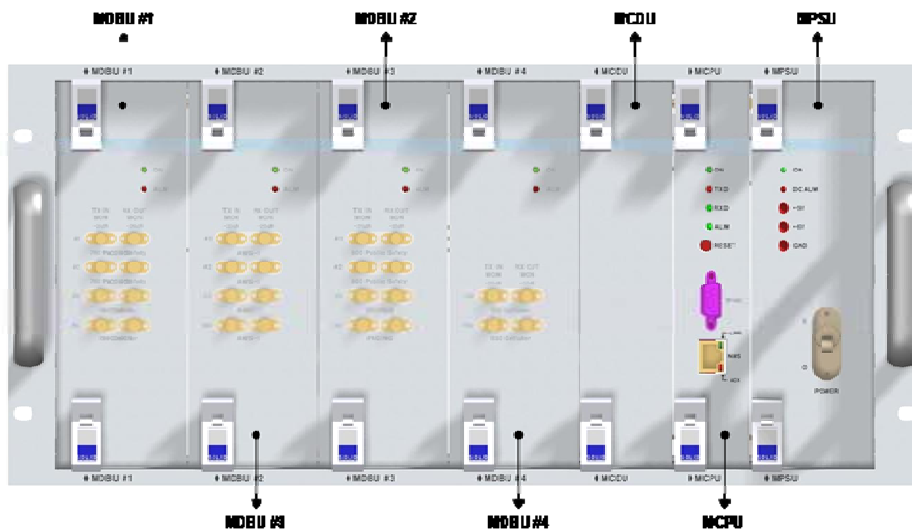
Figure 4.2 – BIU mounting diagram
