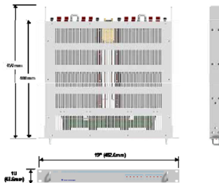
Figure 4.9 – ODU Outer Look
