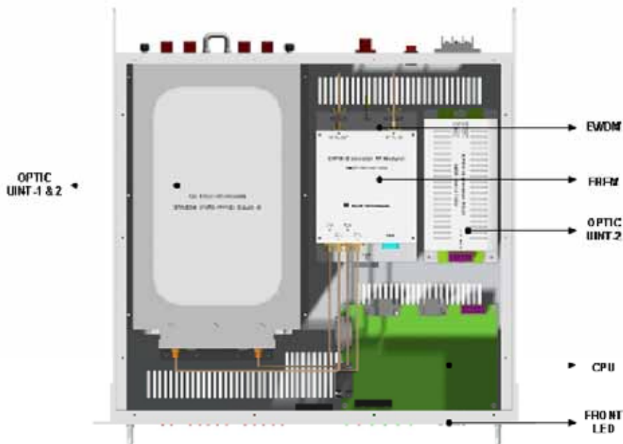
Figure 4.17 – OEU Inner Look
