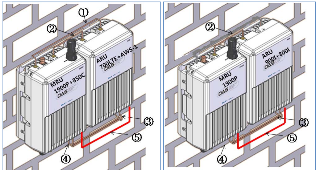
(a)MRU1900P+850C/ARU700LTE/AWS-1
