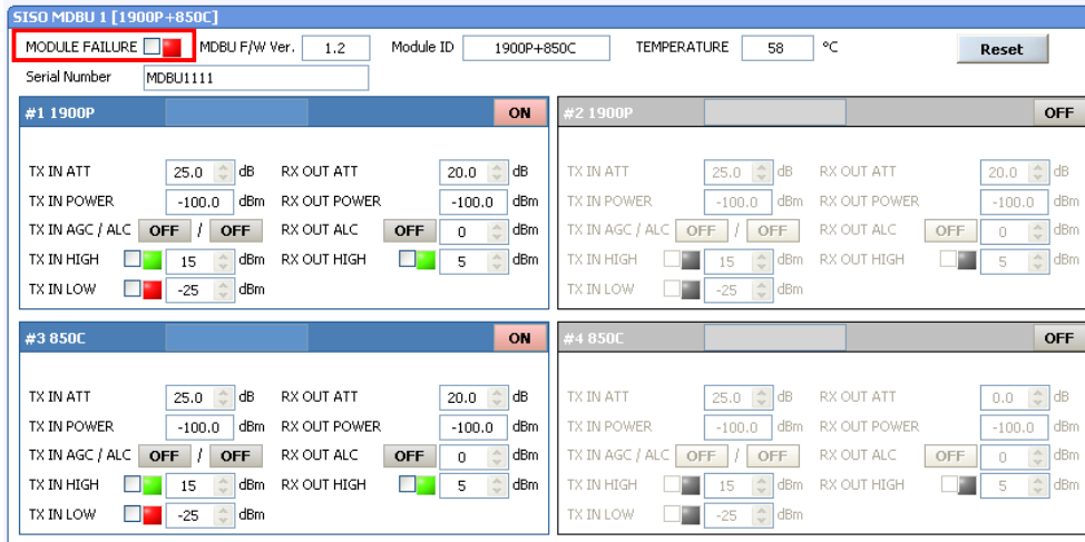
Figure 6.6 –MDBU Module Failure information at the BIU
