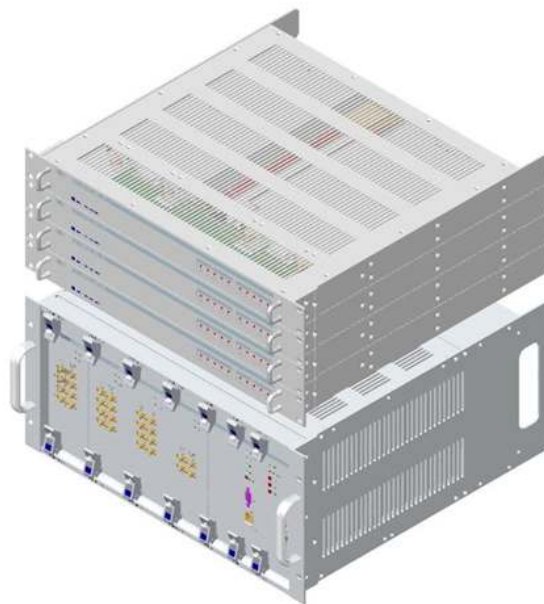
Figure 4.15 – Interface between BIU and ODU
