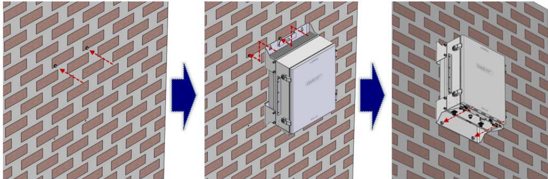
First, install 2 of M12 mounting bolts roughly half way on the enclosure and install enclosure over the bolts and secure tightly. Second, install 2 of M12 mounting bolts under the enclosure and secure tightly.
