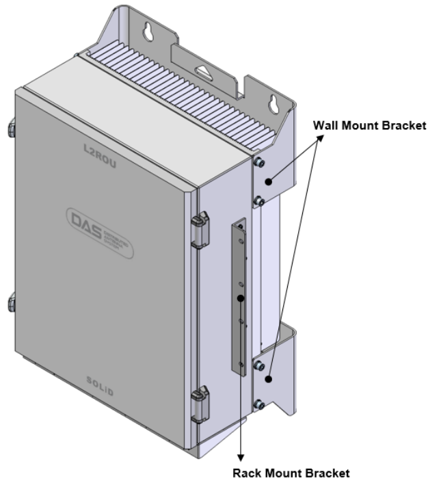
Figure 3.2 – How to install L2ROU
