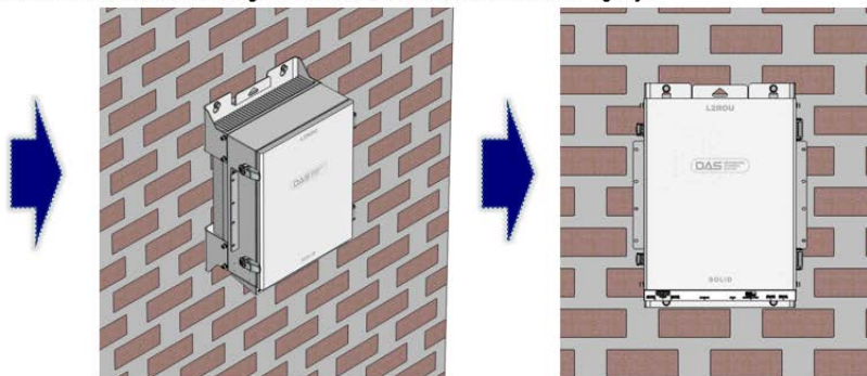
First, install 2 of M12 mounting bolts roughly half way on the enclosure and install enclosure over the bolts and secure tightly. Second, install 2 of M12 mounting bolts under the enclosure and secure tightly.
