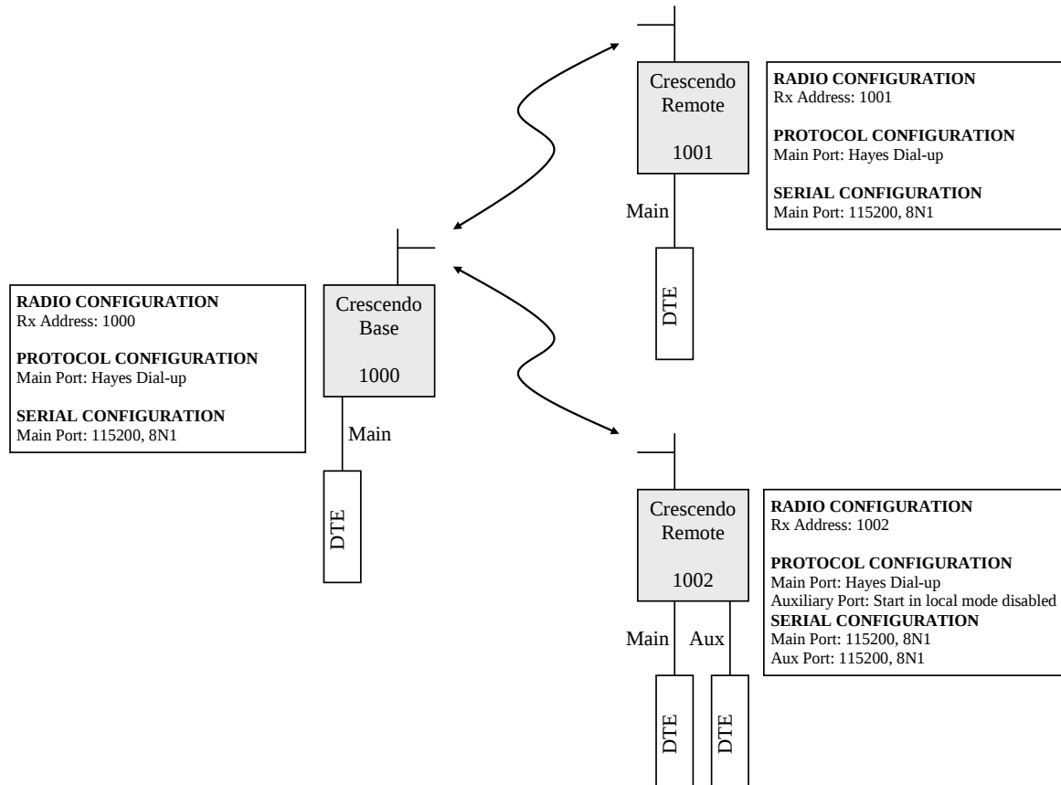
Figure 19: Basic Hayes dial-up network
