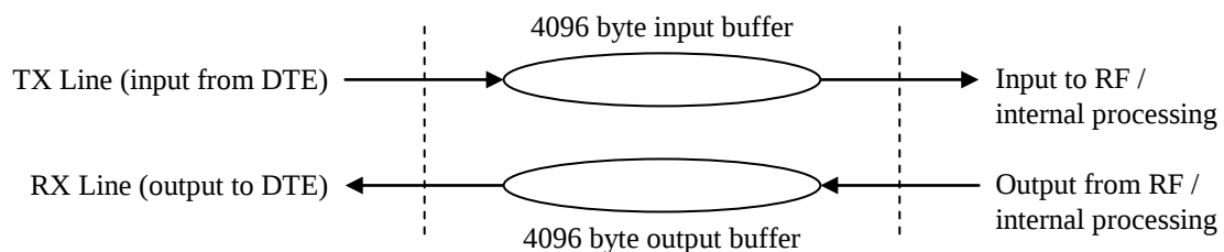
Figure 2: Buffering scheme on the Crescendo
