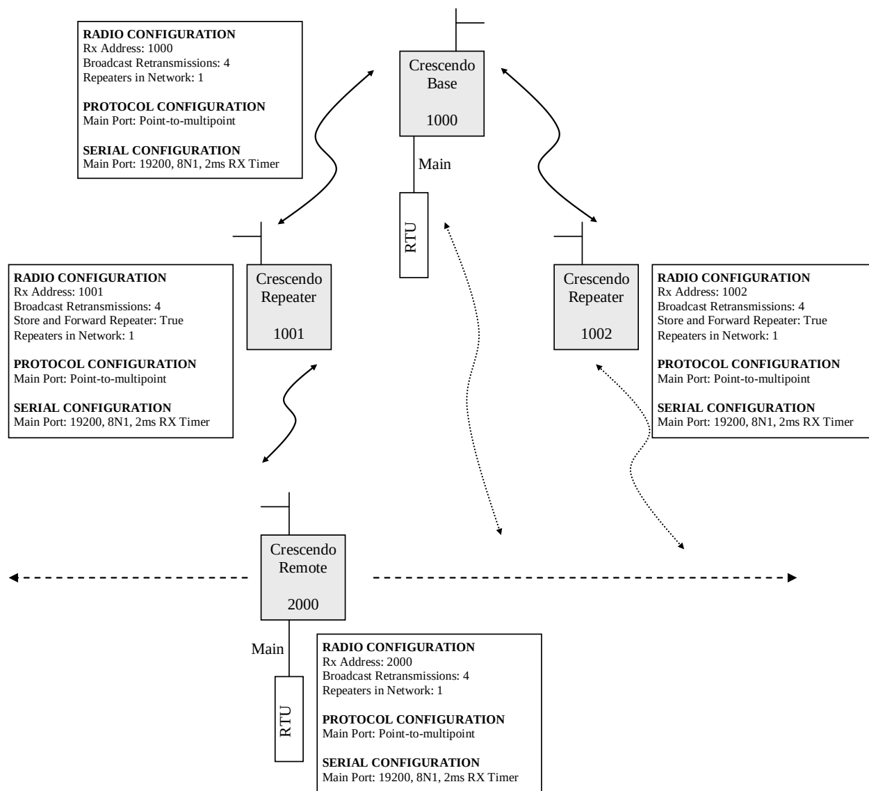
Figure 18: Point-to-multipoint network with roaming remote
