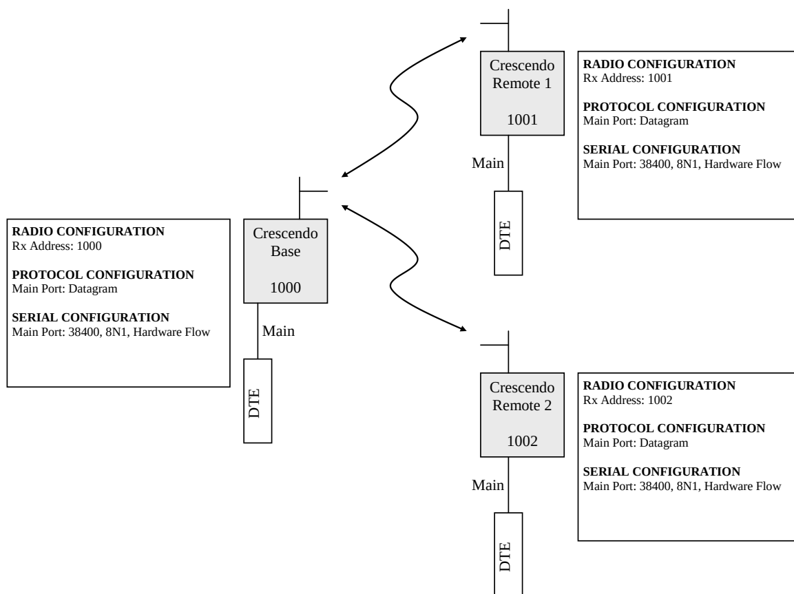
Figure 24: Basic datagram network
