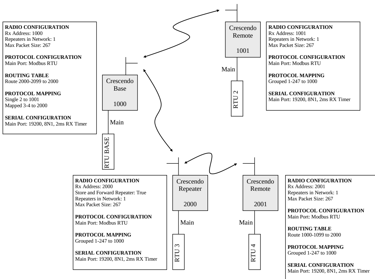
Figure 21: Modbus network with repeater
