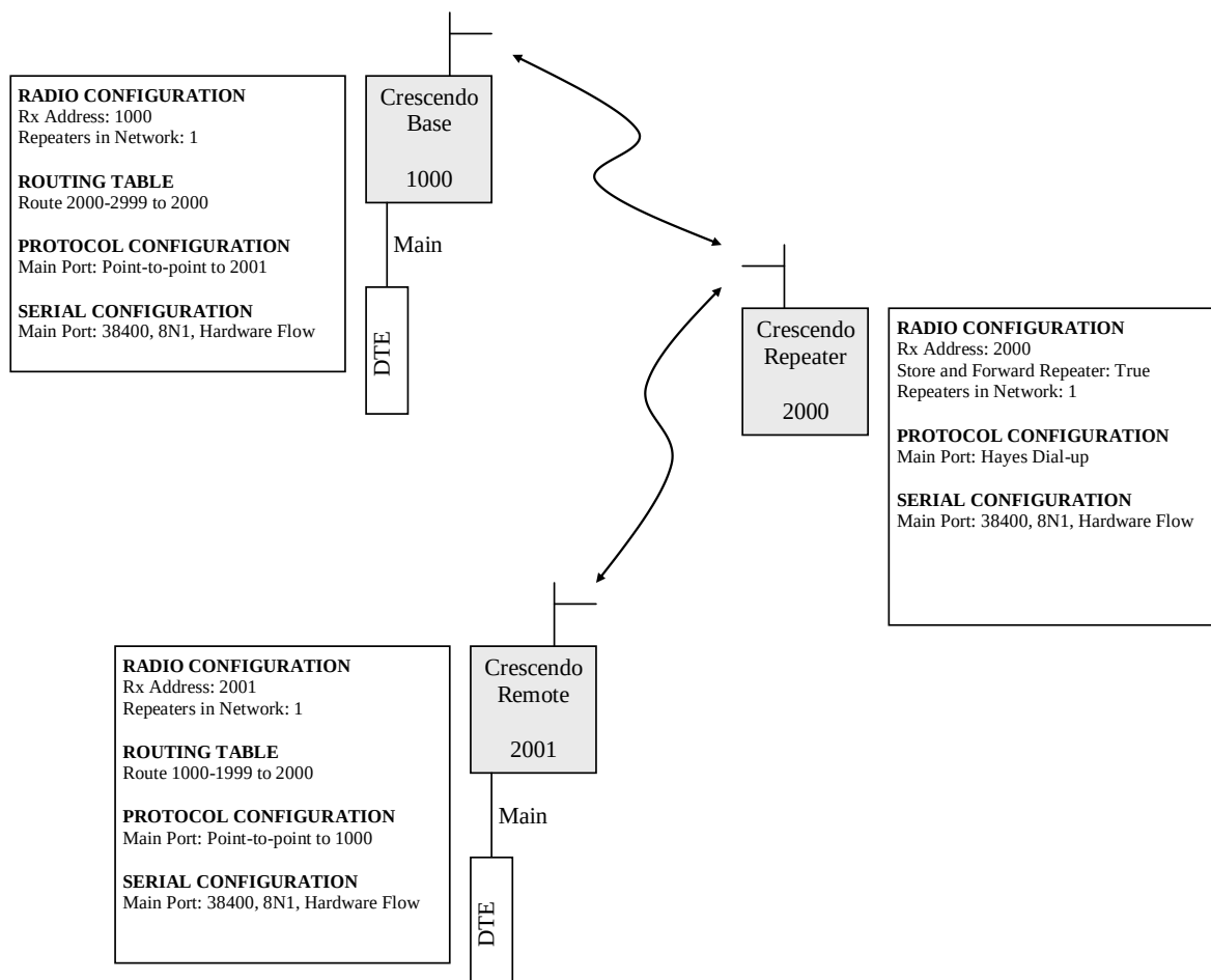
Figure 16: Point-to-point network with repeater
