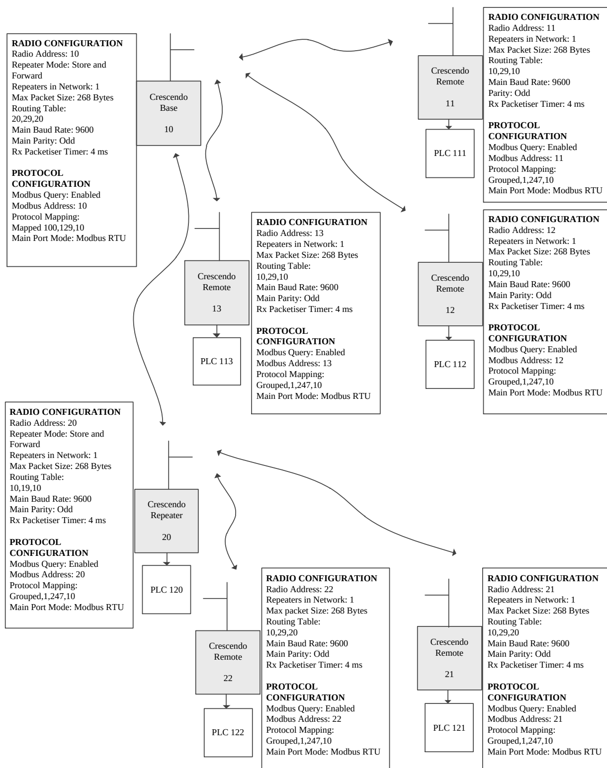
Figure 22: Modbus with Modbus query enabled
