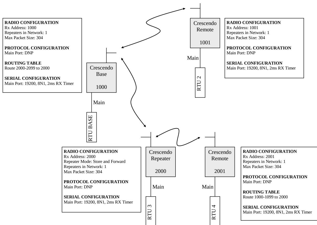
Figure 23: DNP network with repeater
