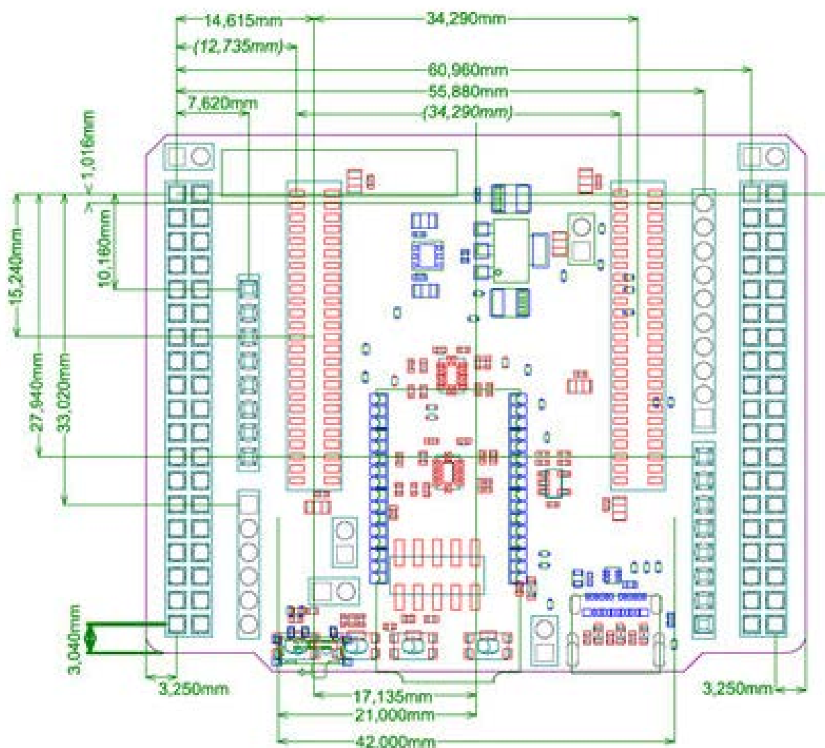
Figure 6. NUCLEO-WBA52CG mechanical dimensions (in millimeters)
