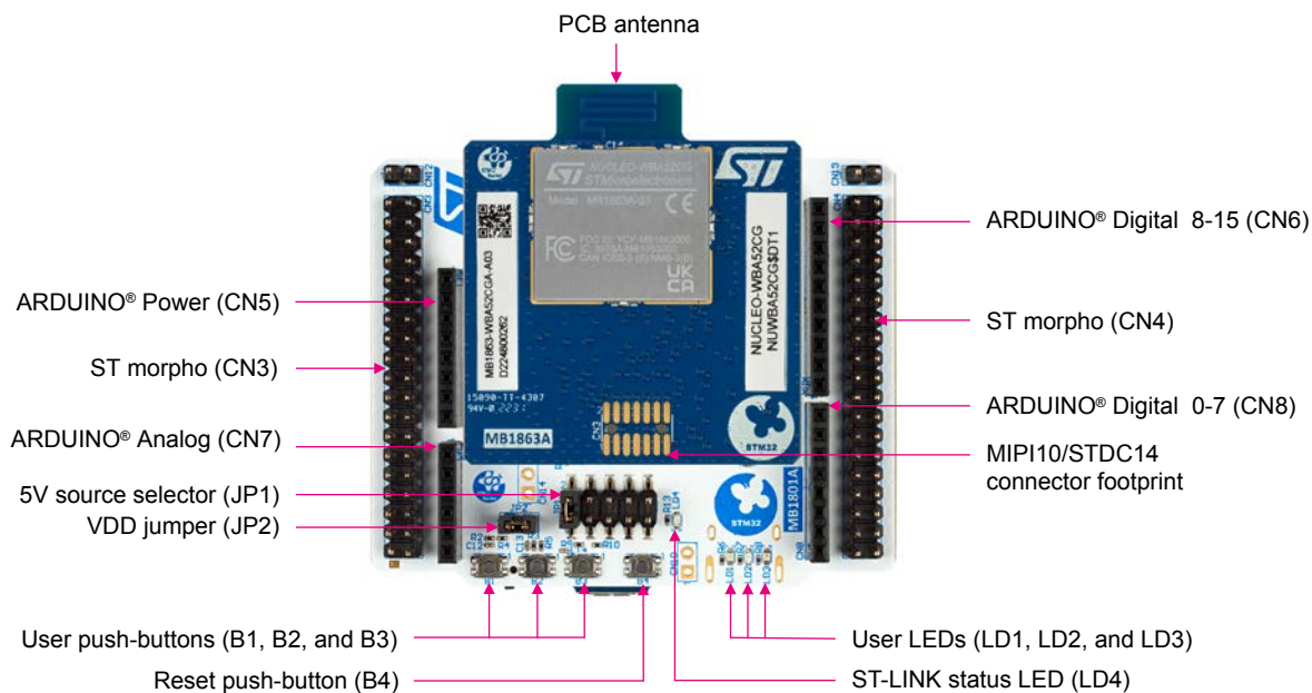
Figure 3. NUCLEO-WBA52CG PCB top view
