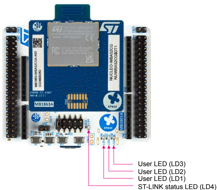
Figure 11. LEDs location
