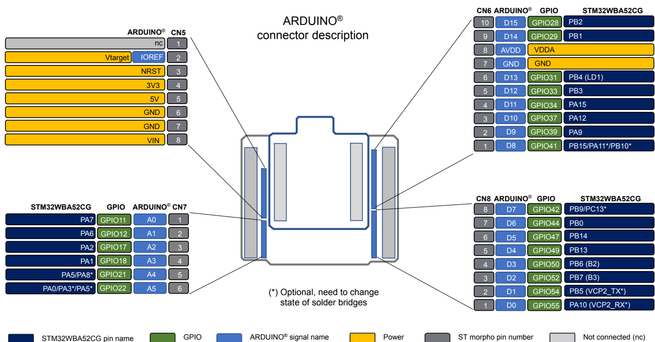
Figure 15. ARDUINO® connector pinout
