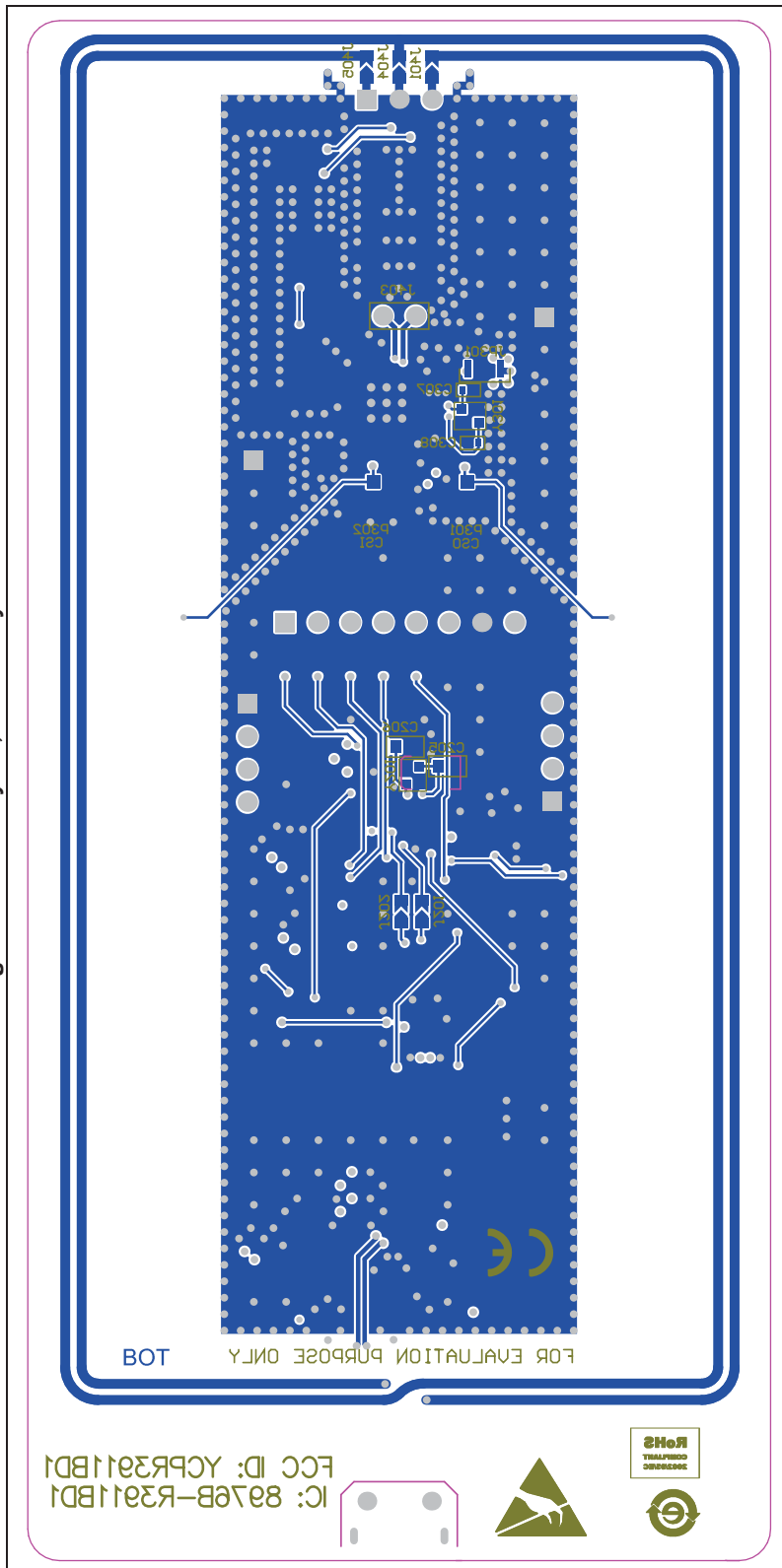
Figure 12. PCB layout, bottom layer
