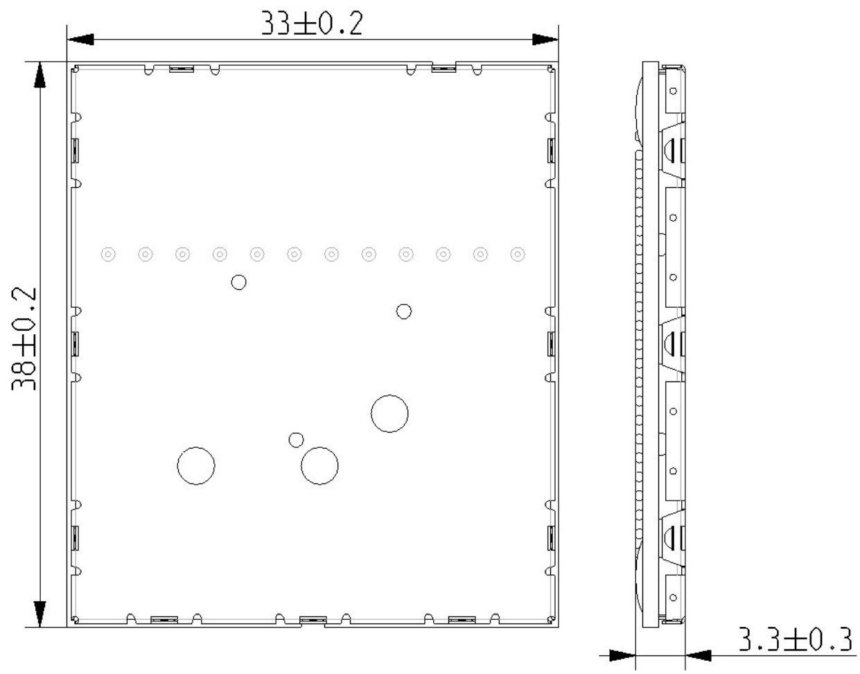
Figure 20 CO230 dimensions
