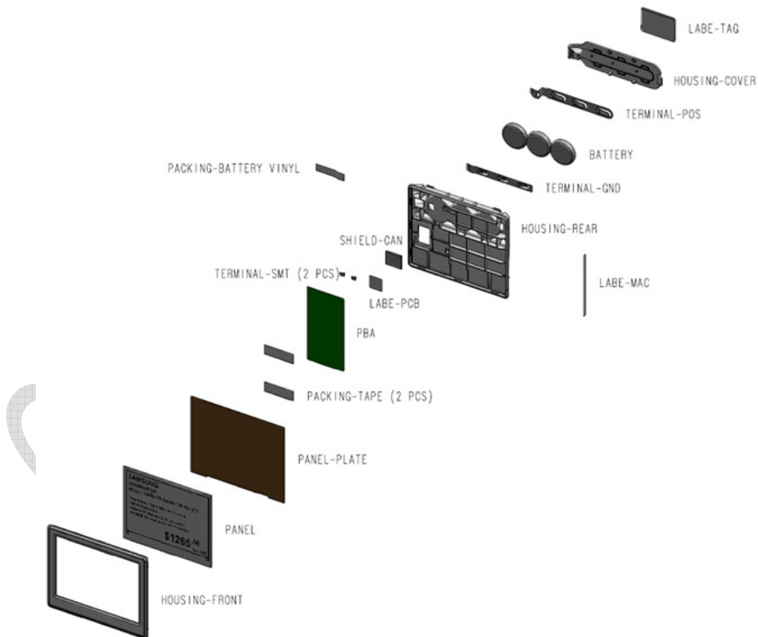
Figure 4 Exploded View
