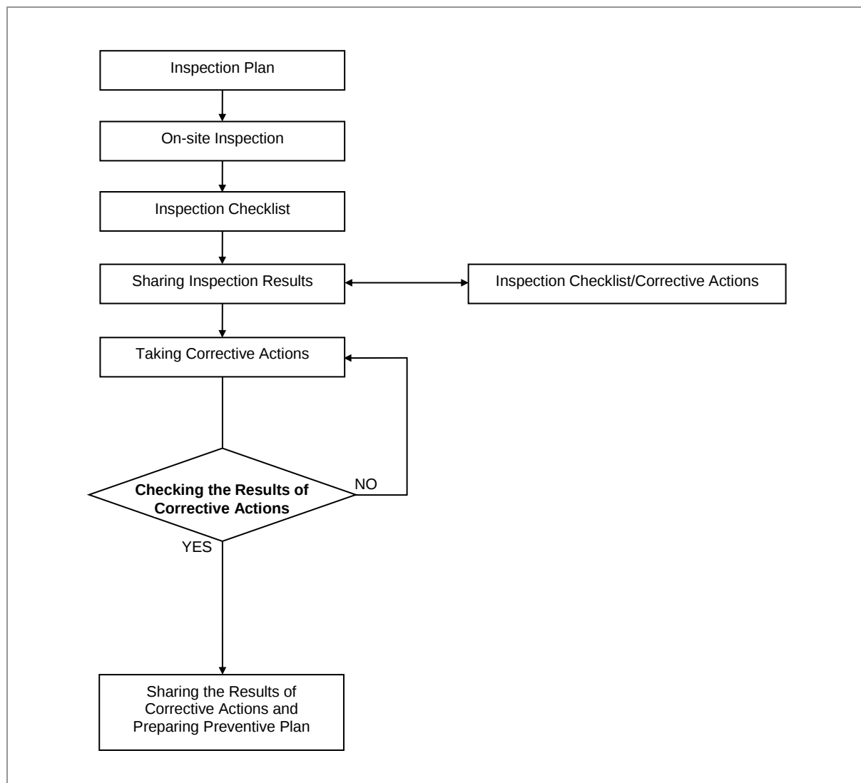
Figure 106. Installation Inspection Procedure
