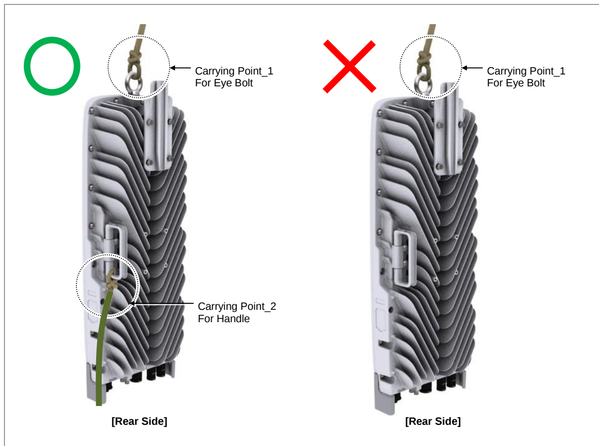
Figure 58. Lifting HRU (1)
