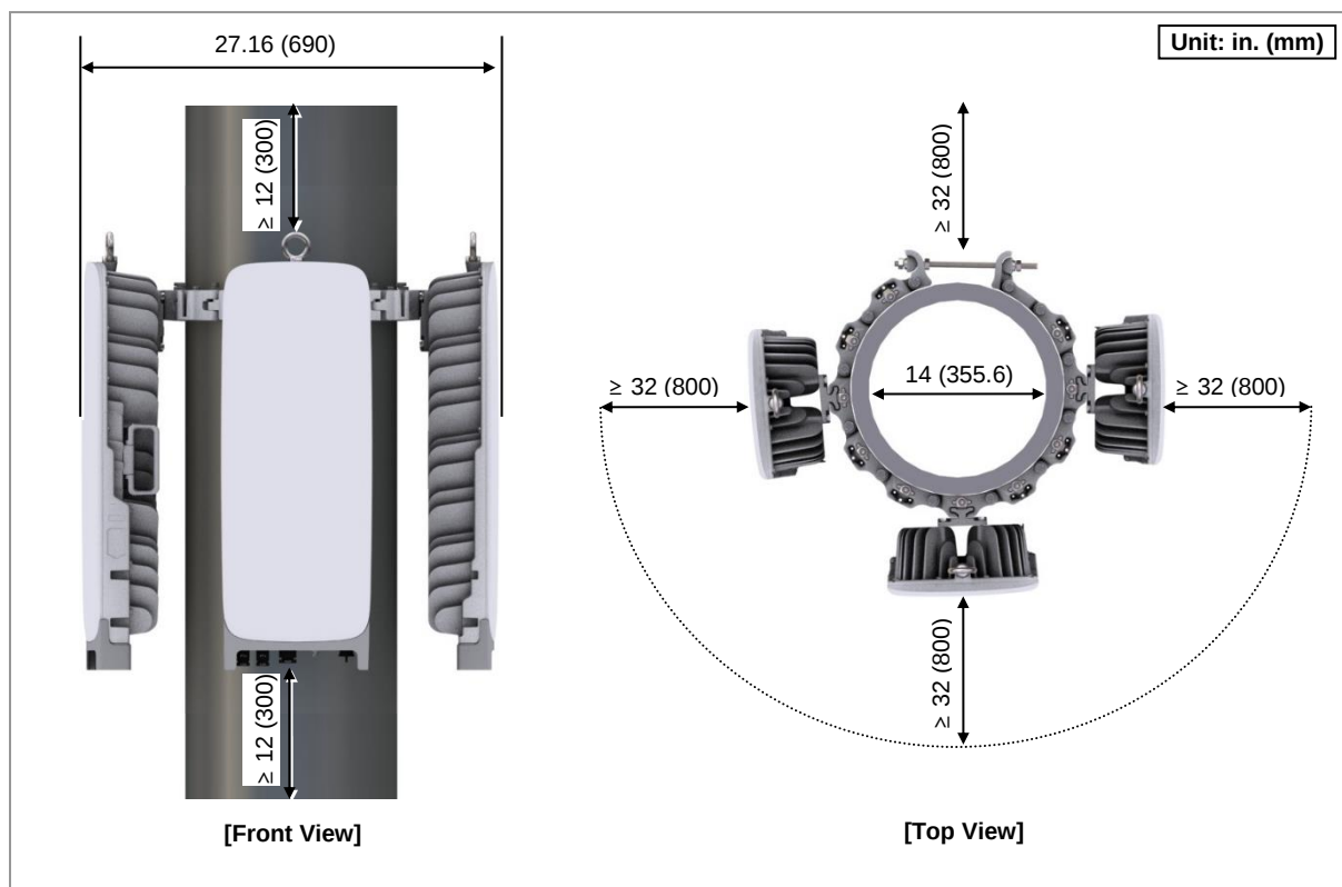
Figure 11. HRU Arrangement_3 Sector Pole Type Installation
