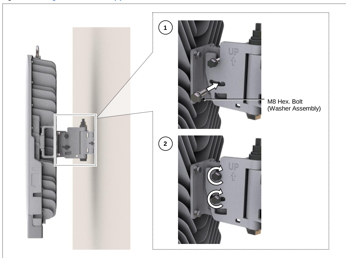
Figure 44. Fixing HRU on the Wall (2)
