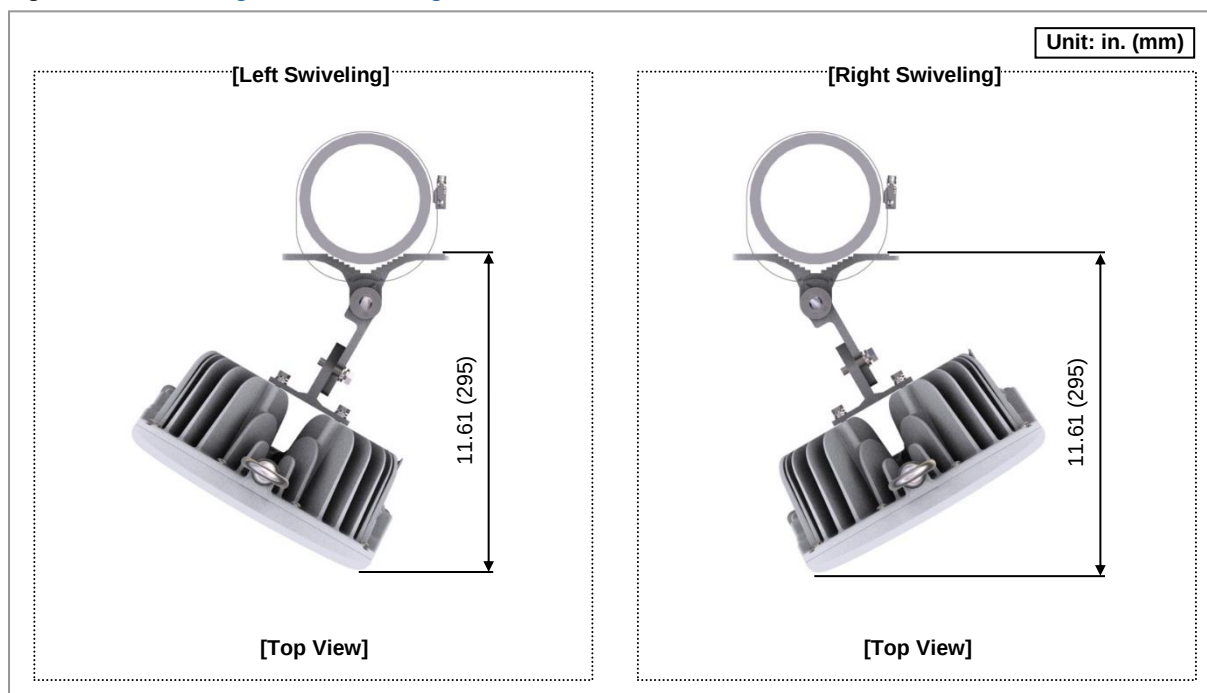
Figure 8. HRU Arrangement_Swiveling
