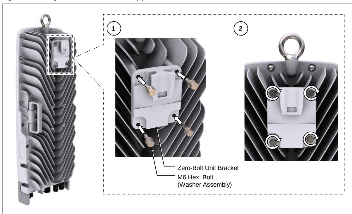
Figure 78. Fixing Zero-Bolt Unit Bracket (2)
