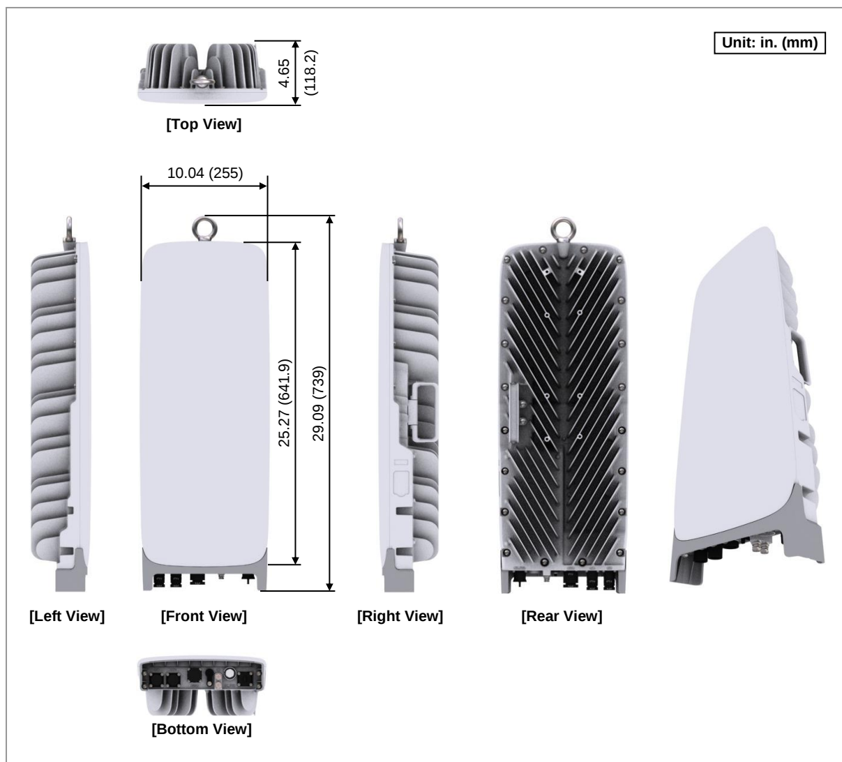
Figure 1. HRU View
