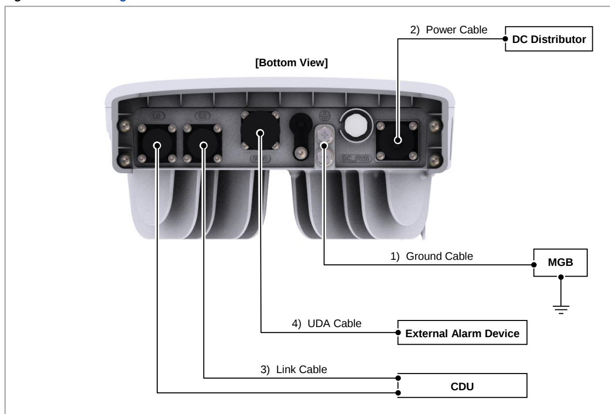
Figure 91. Cable Diagram
