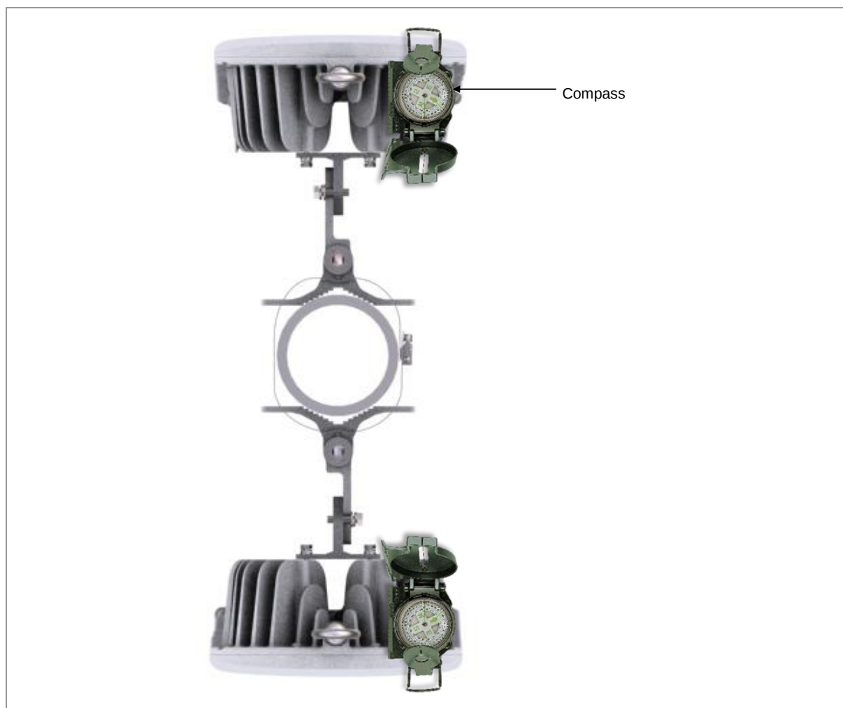
Figure 37. Fixing HRUs on the Pole (5)
