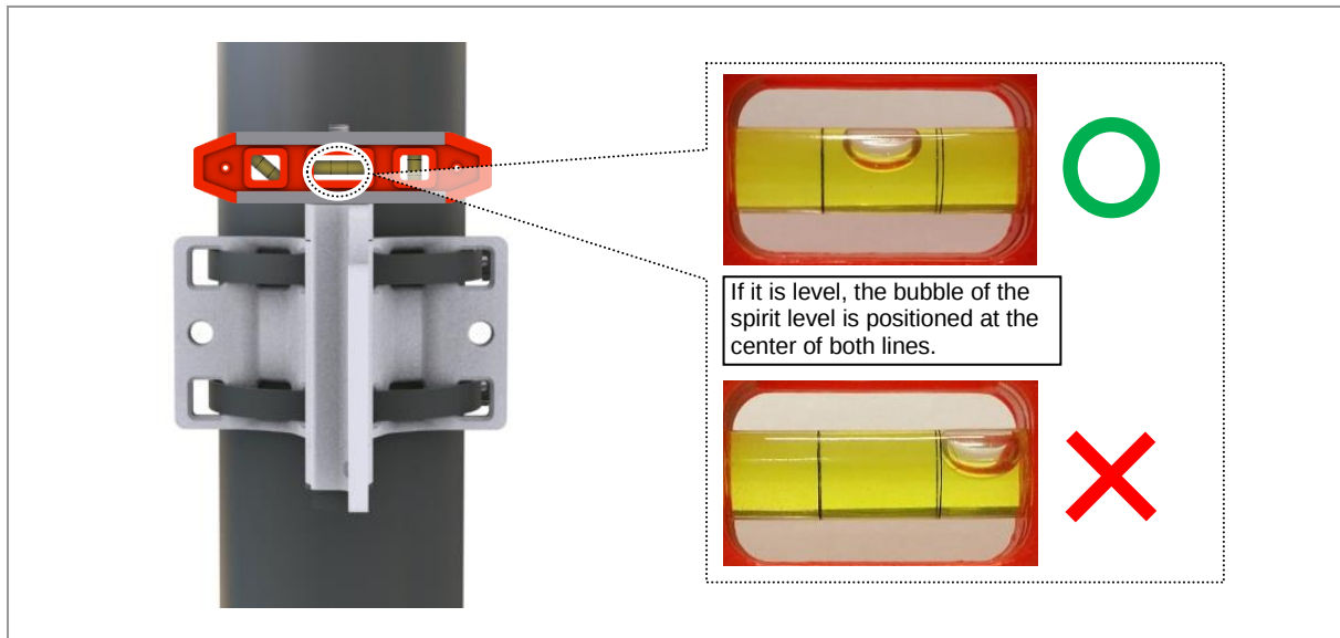
Figure 20. Fixing Mounting Bracket on the Pole (5)
