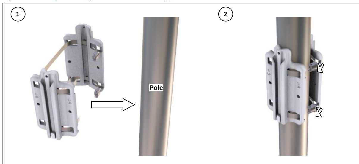
Figure 66. Fixing Mounting Bracket on the Pole (3)
