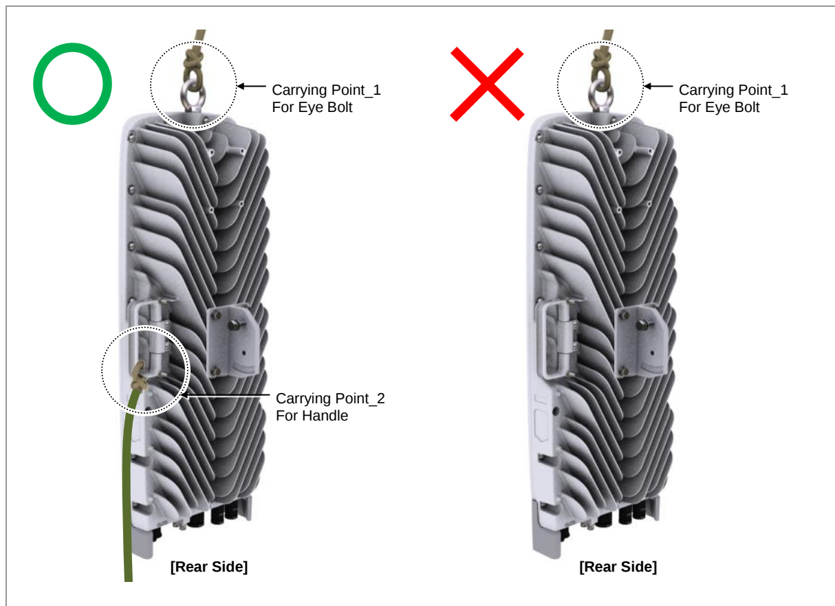
Figure 21. Lifting HRU (1)
