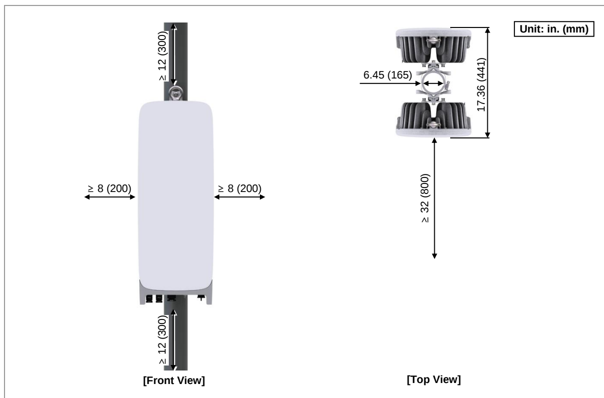
Figure 10. HRU Arrangement_2 Sector Pole Type Installation
