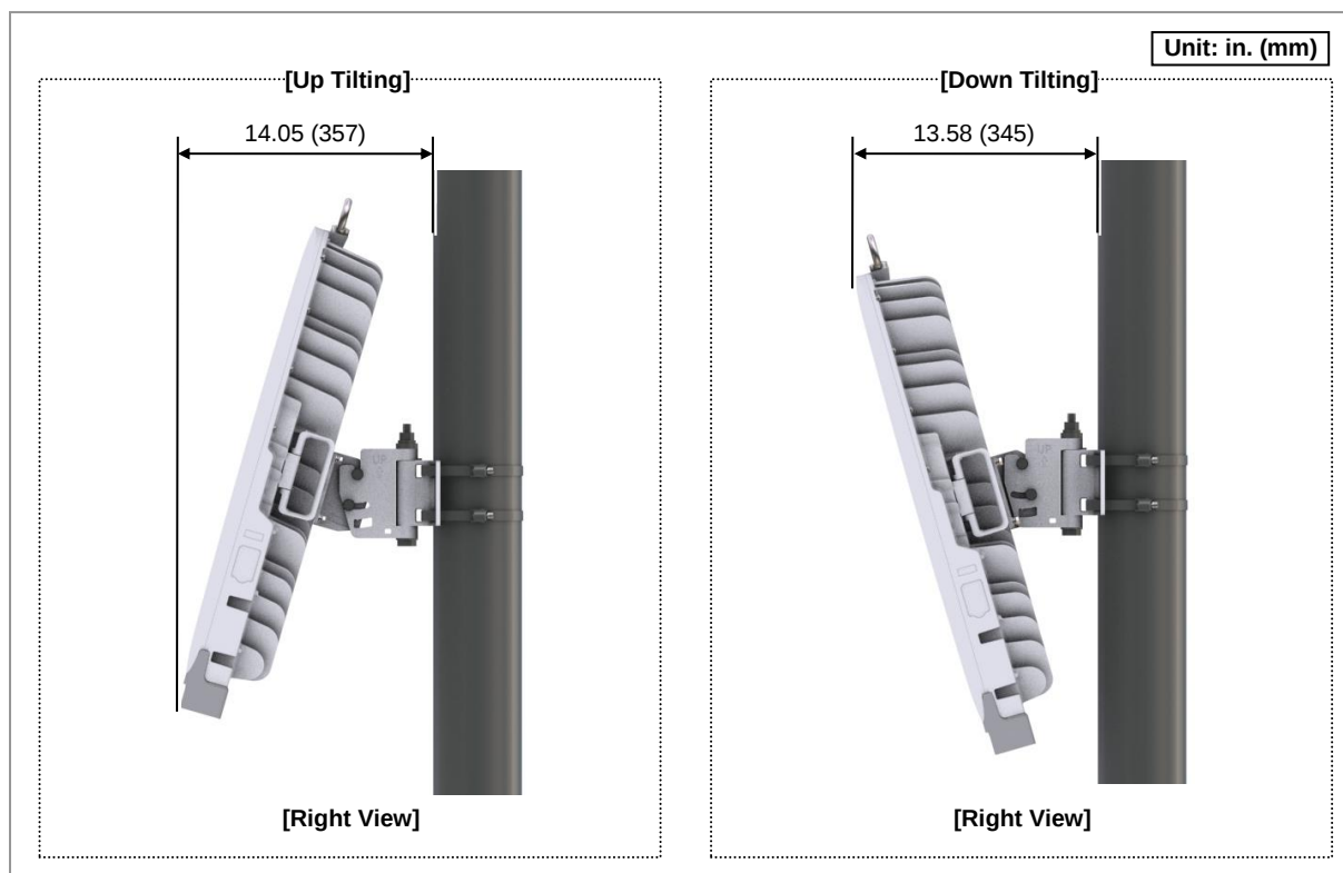
Figure 7. HRU Arrangement_Tilting
