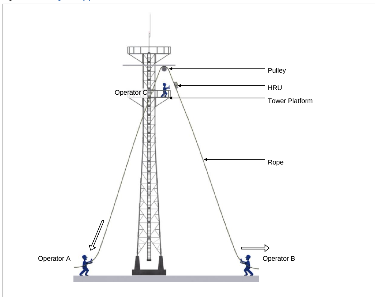
Figure 59. Lifting HRU (2)
