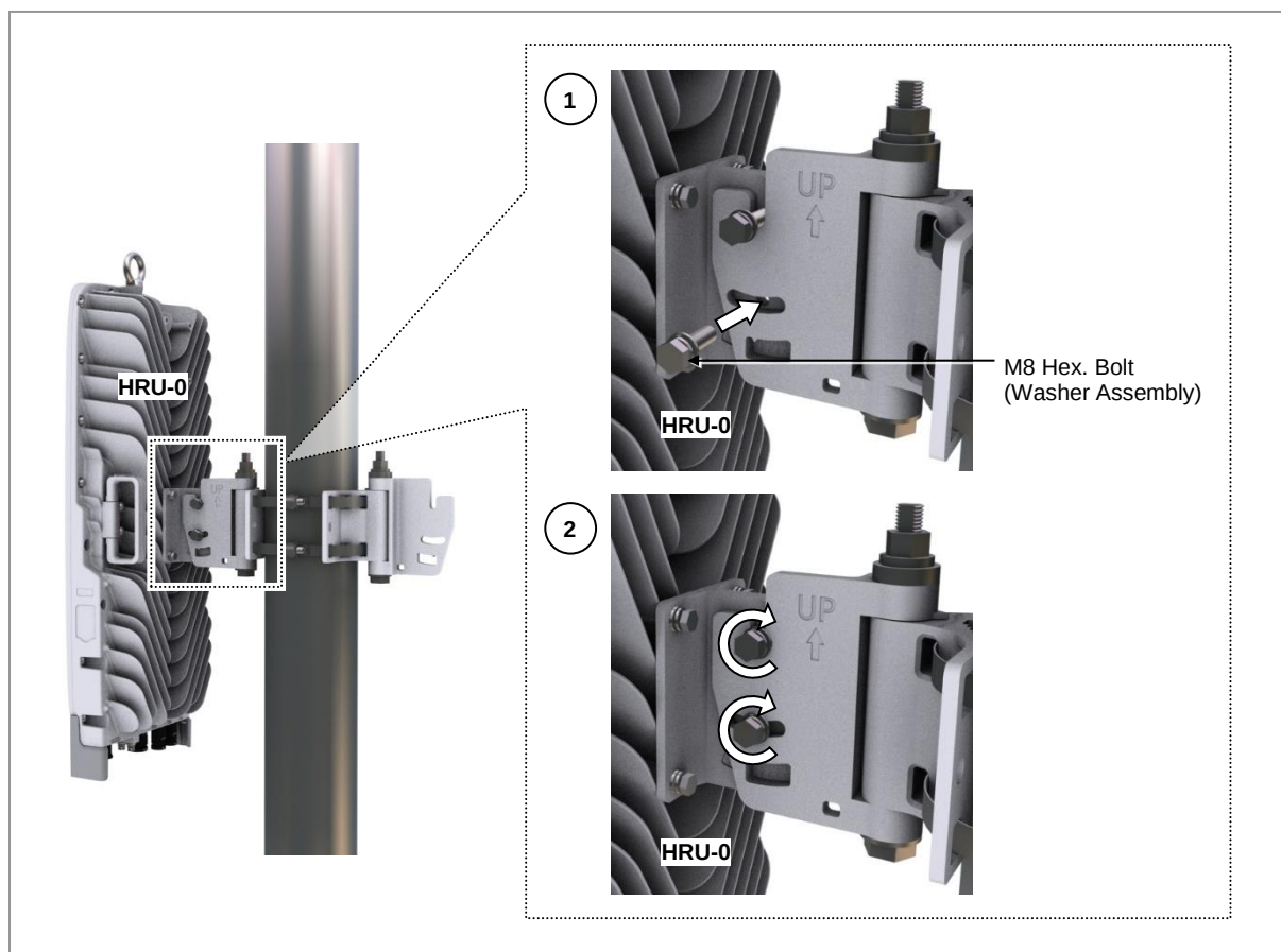
Figure 34. Fixing HRUs on the Pole (2)
