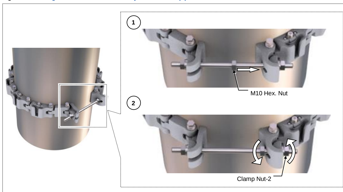
Figure 83. Fixing Chain Bracket Assembly on the Pole (3)
