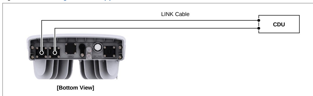
Figure 98. Connecting LINK Cable (1)
