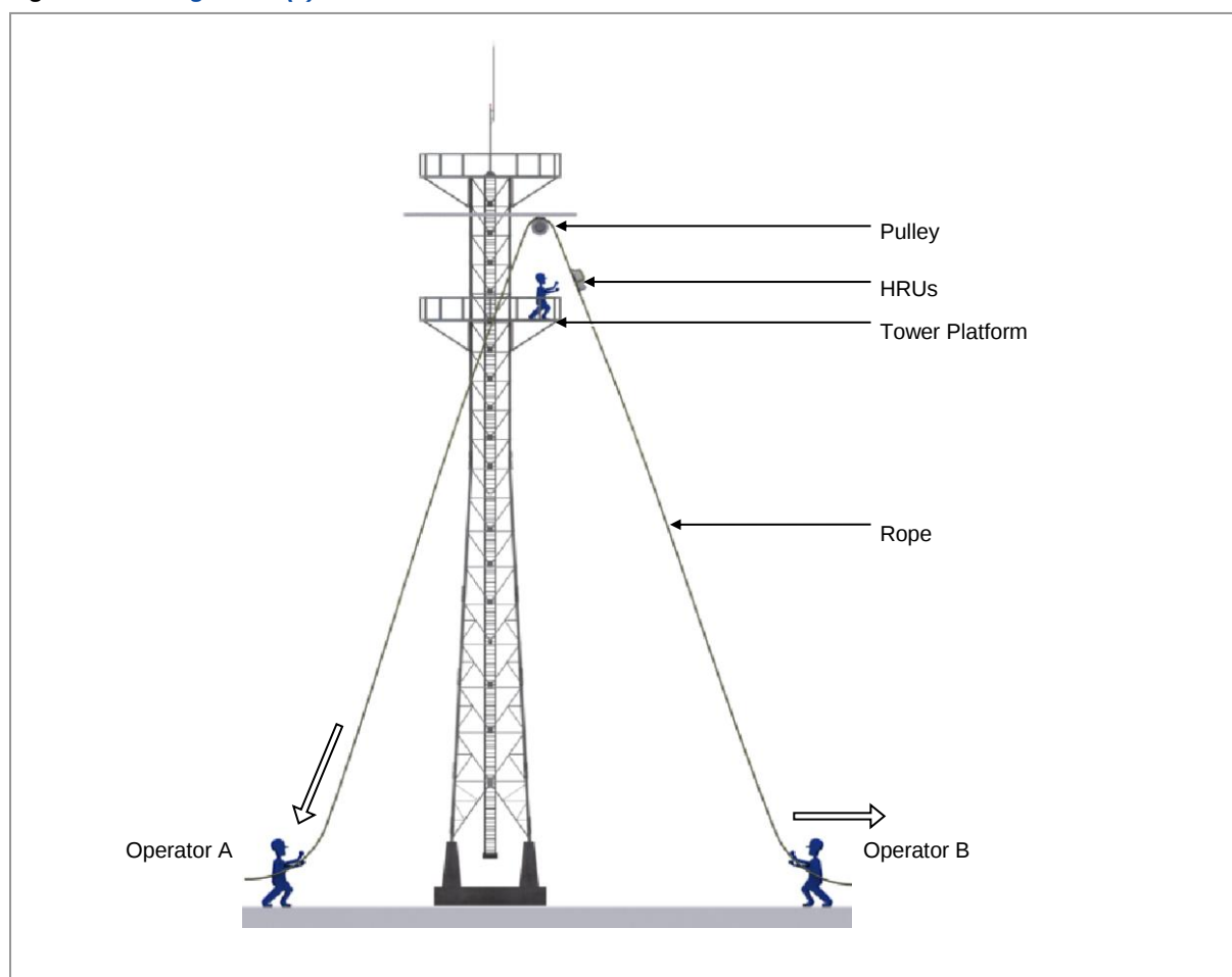
Figure 70. Lifting HRUs (2)
