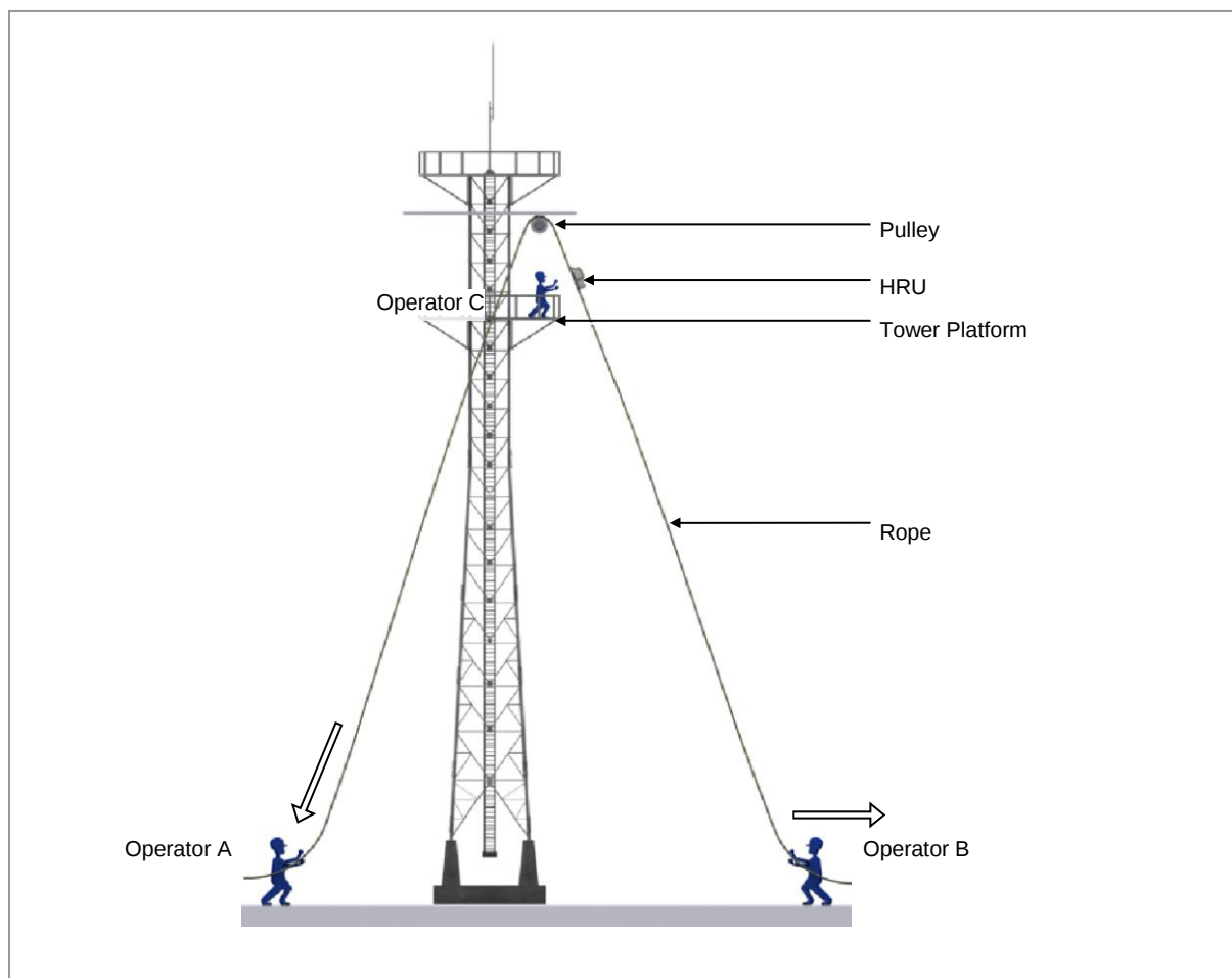
Figure 22. Lifting HRU (2)
