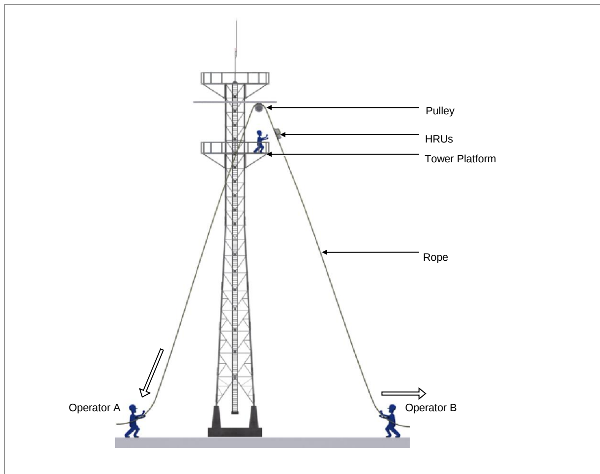
Figure 86. Lifting HRUs (2)
