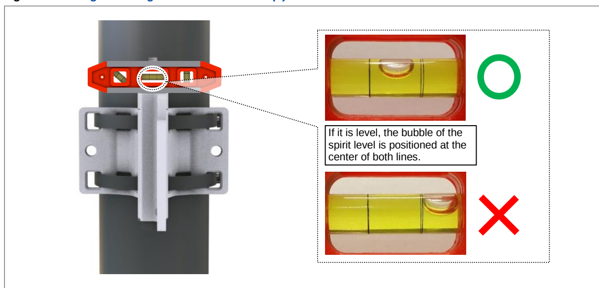
Figure 30. Fixing Mounting Bracket on the Pole (5)
