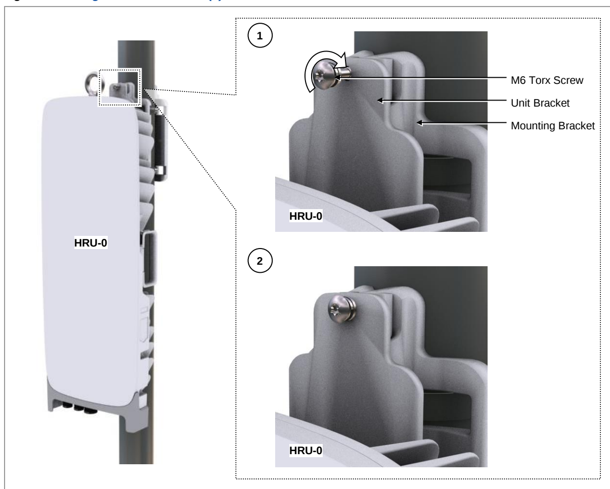
Figure 73. Fixing HRUs on the Pole (3)
