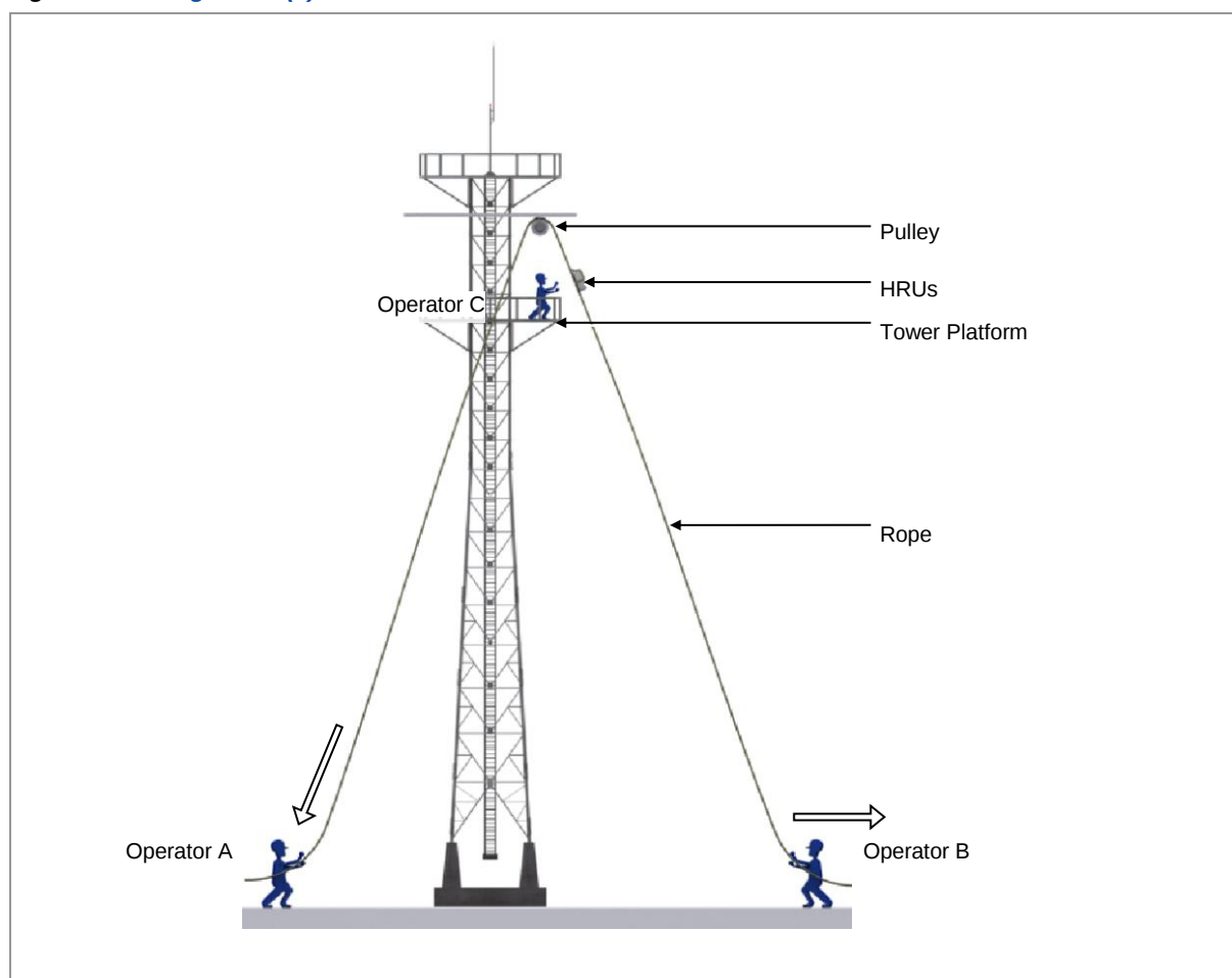
Figure 32. Lifting HRUs (2)
