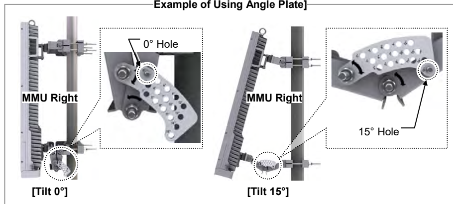
Example of Using Angle Plate]
