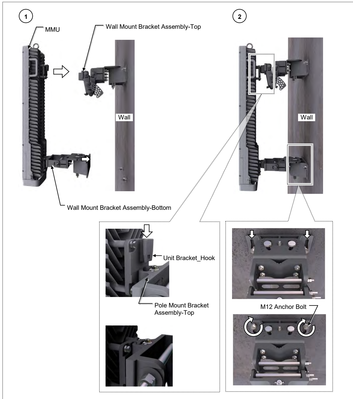
Figure 35. Fixing MMU
