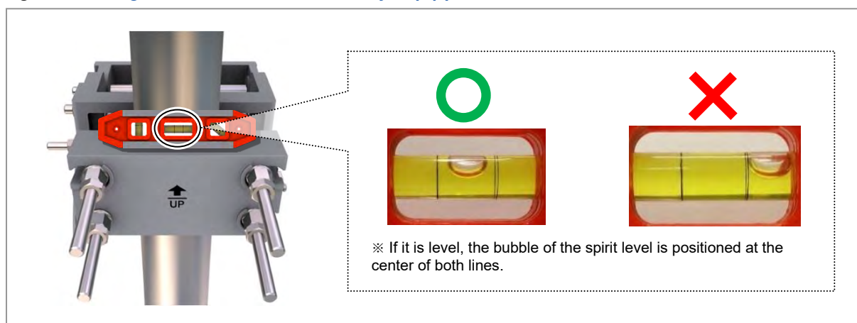
Figure 24. Fixing Pole Mount Bracket Assembly-Top (6)
