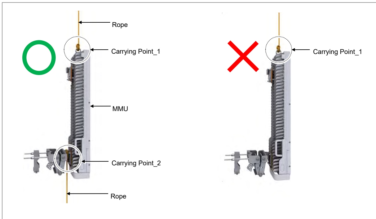
Figure 48. Lifting MMU & Pole Mount Bracket Assembly-Top (2)
