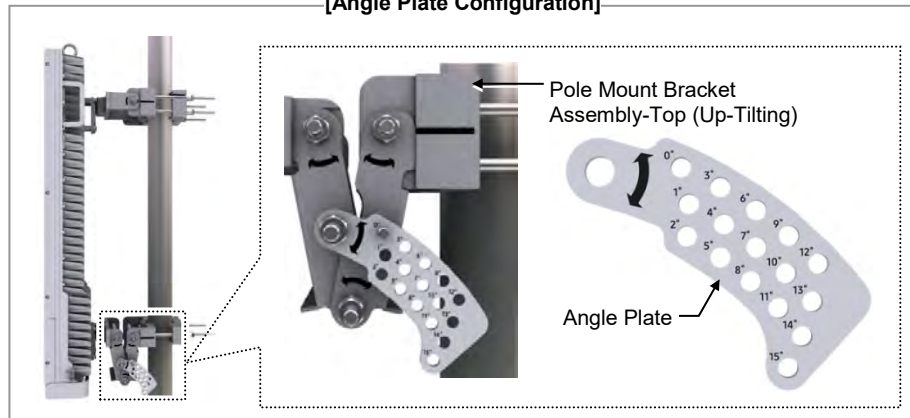
Example of Using Angle Plate]
