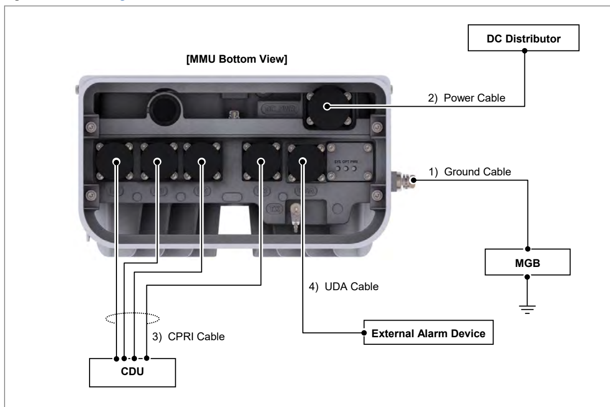
Figure 71. Cable Diagram
