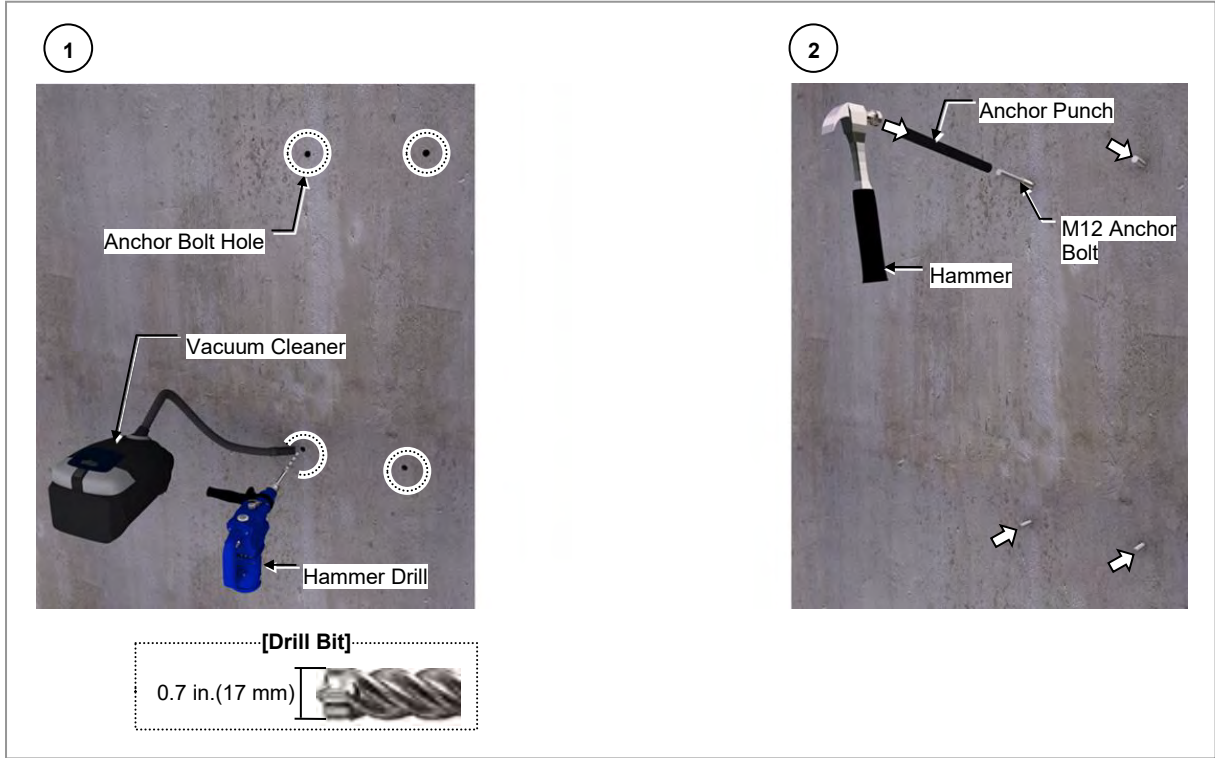
Figure 30. Drilling & Anchor (1)
