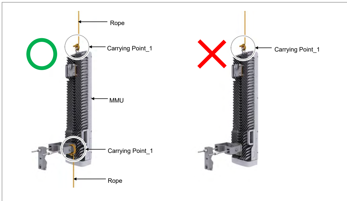
Figure 17. Lifting MMU & Pole Mount Bracket Assembly-Top (2)
