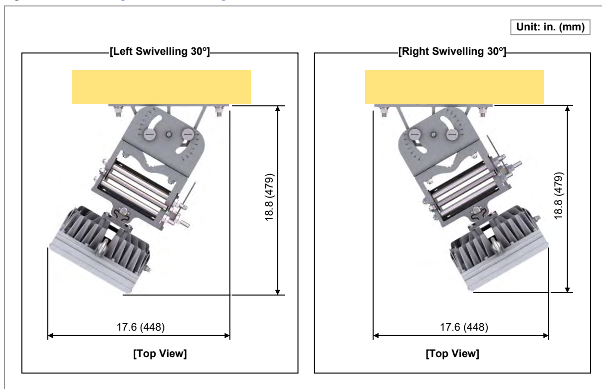
Figure 6. MMU Arrangement_Swivelling
