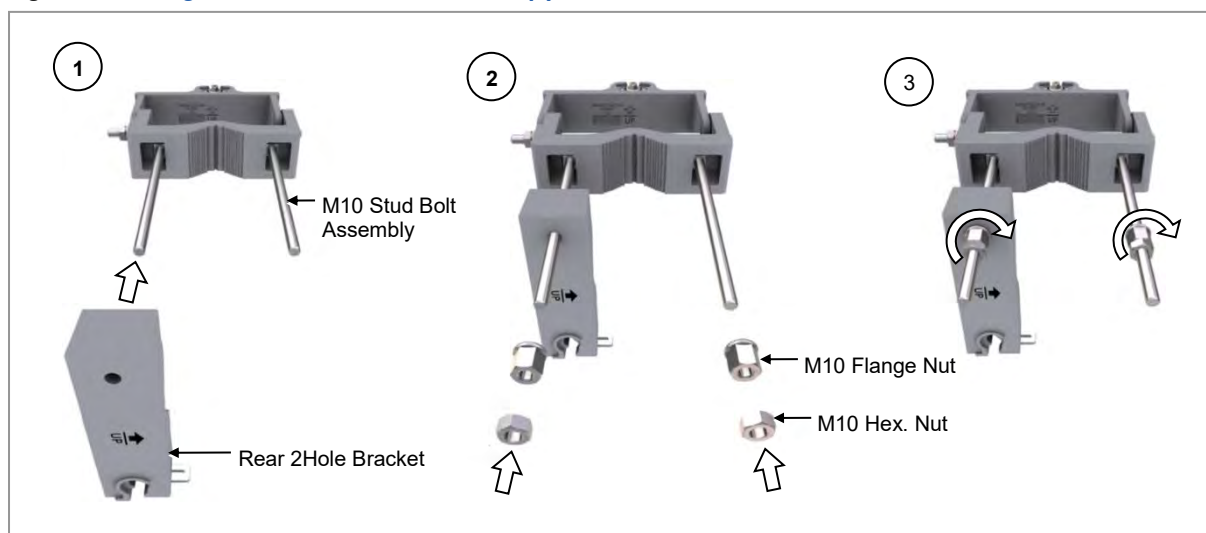
Figure 11. Fixing Pole Mount Bracket-Bottom (2)
