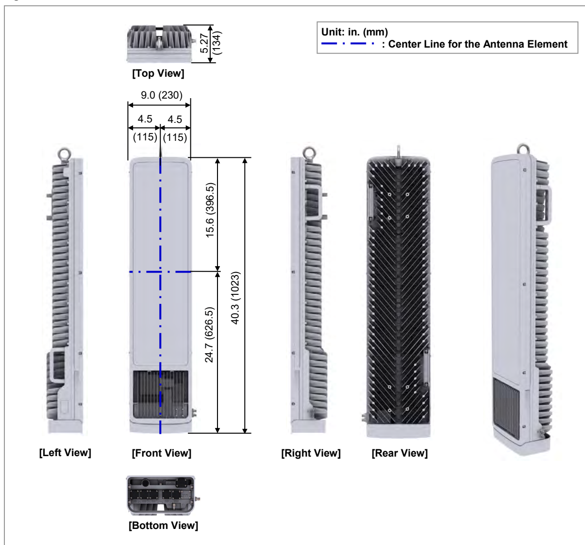
Figure 1. MMU View
