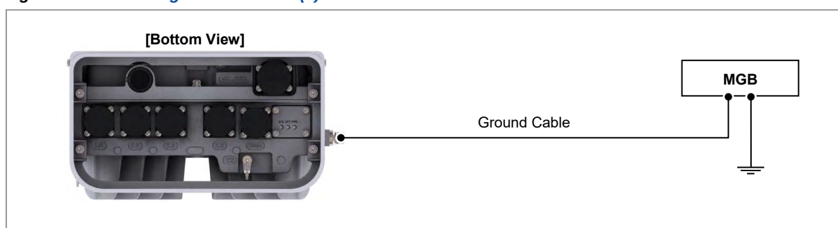
Figure 72. Connecting Ground Cable (1)
