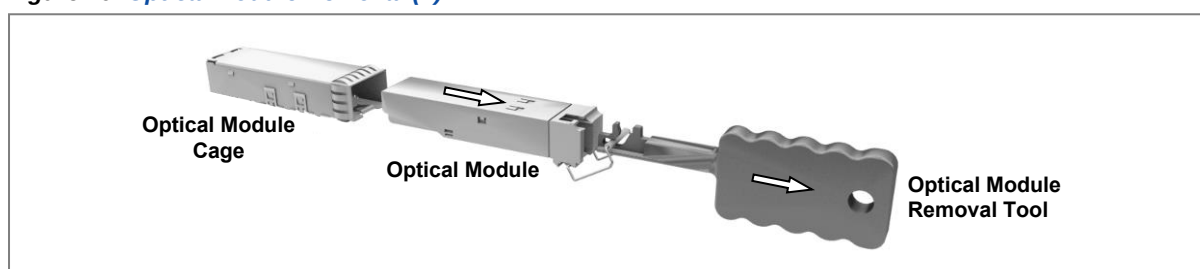
Figure 79. Optical Module Removal (2)
