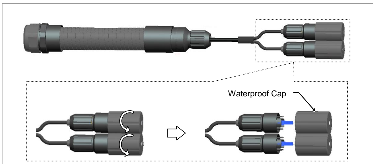
Figure 60. Optic Cable Adapter Assembly (9)
