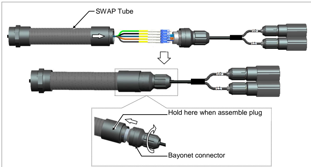
Figure 57. Optic Cable Adapter Assembly (6)
