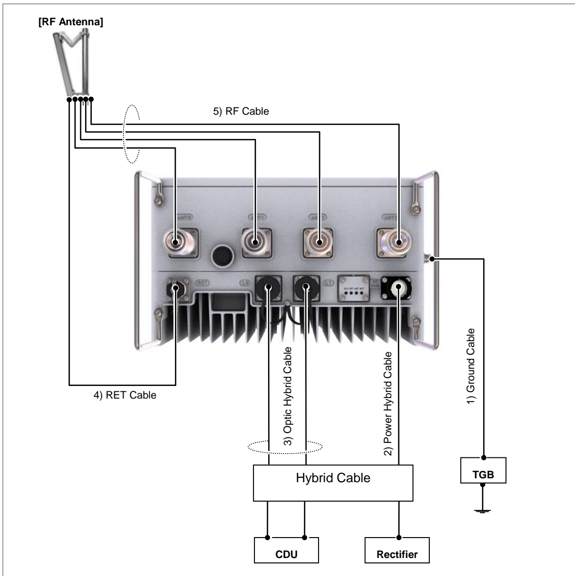
Figure 32. Cable Diagram
