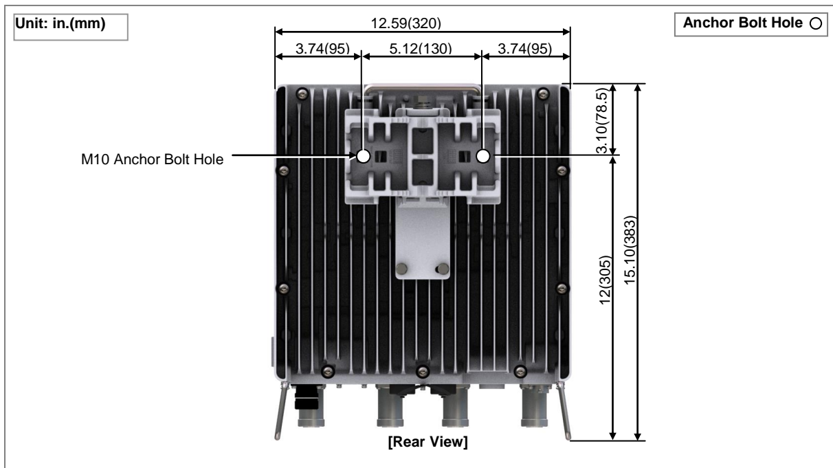
Figure 21. RRU dimensions for Wall Type (Standard Installation)
