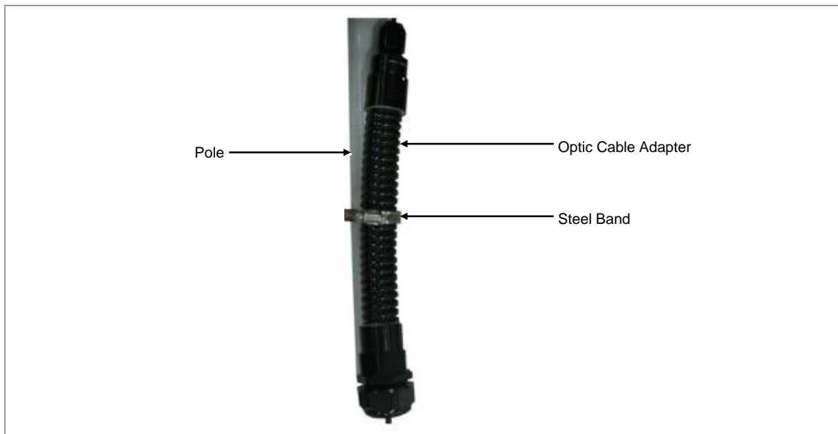
Figure 61. Optic Cable Adapter Assembly (10)
