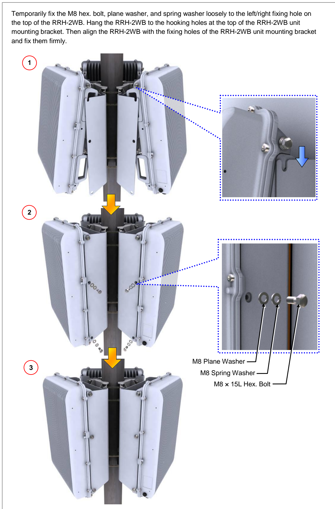
Figure 2.18 Fixing 3 Sector Pole Type RRH-2WB (5)
