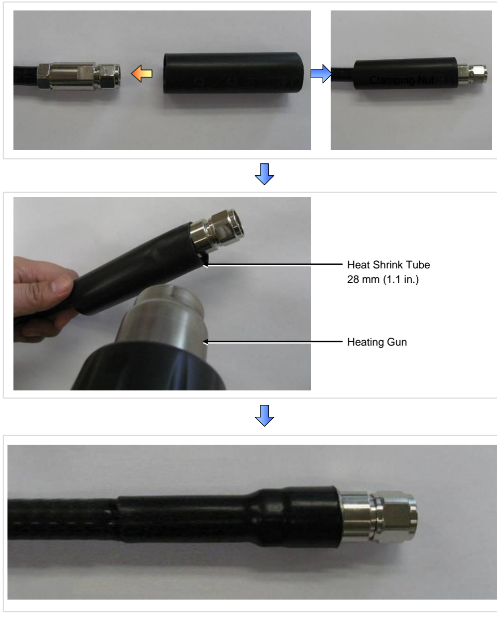
Figure C.4 Assembling the N type-male (1/2 in. Feeder Line) Connector (4)
