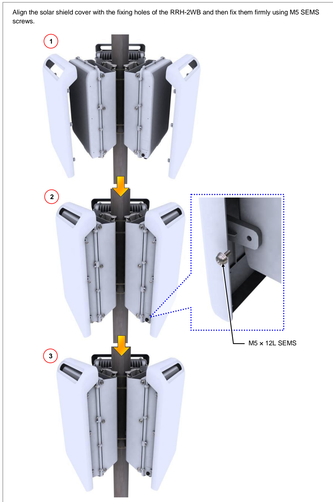
Figure 2.19 Fixing 3 Sector Pole Type RRH-2WB (6)
