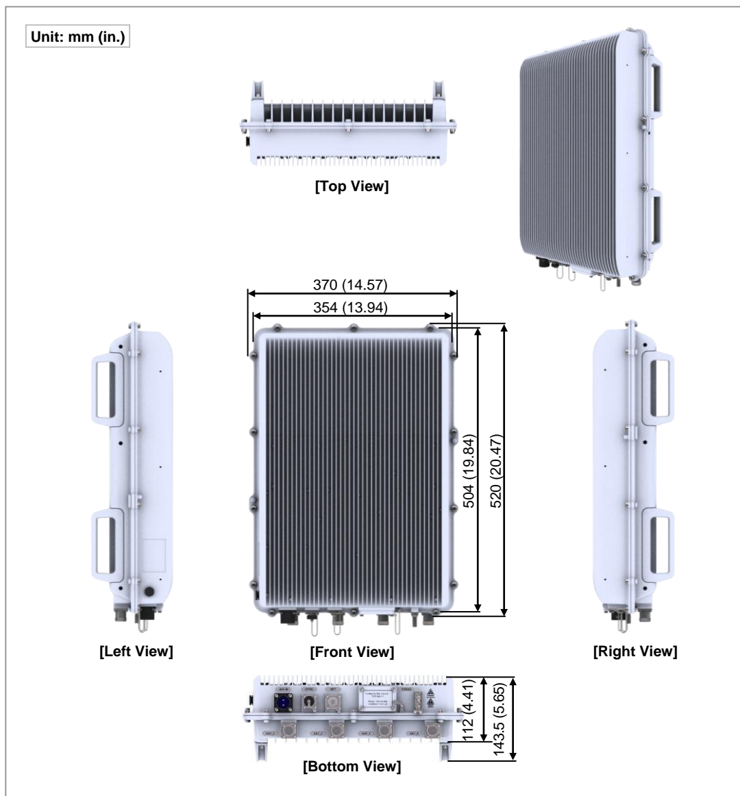
Figure 1.1 RRH-2WB Configuration
