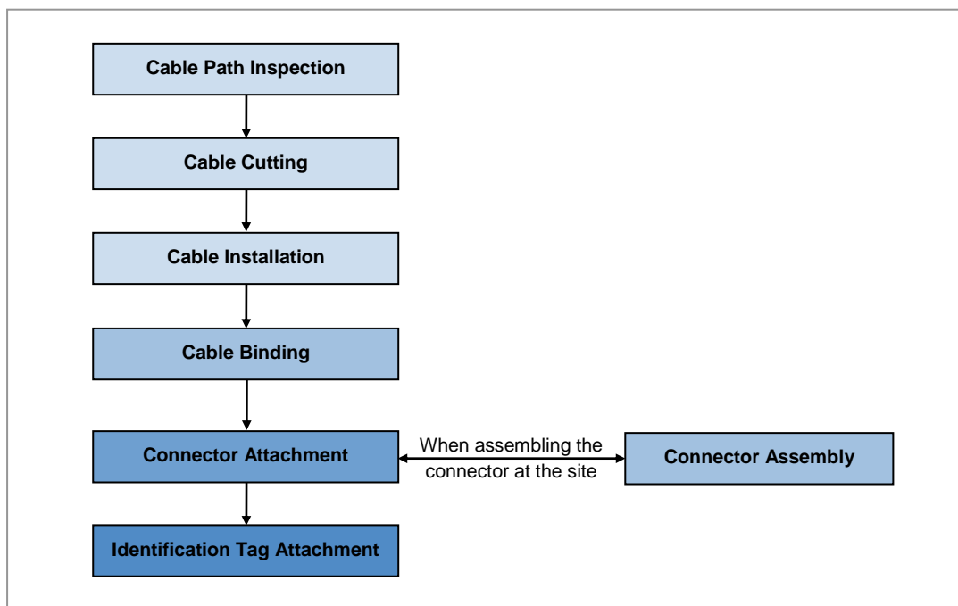
Figure 3.1 Work Flow for Cabling
