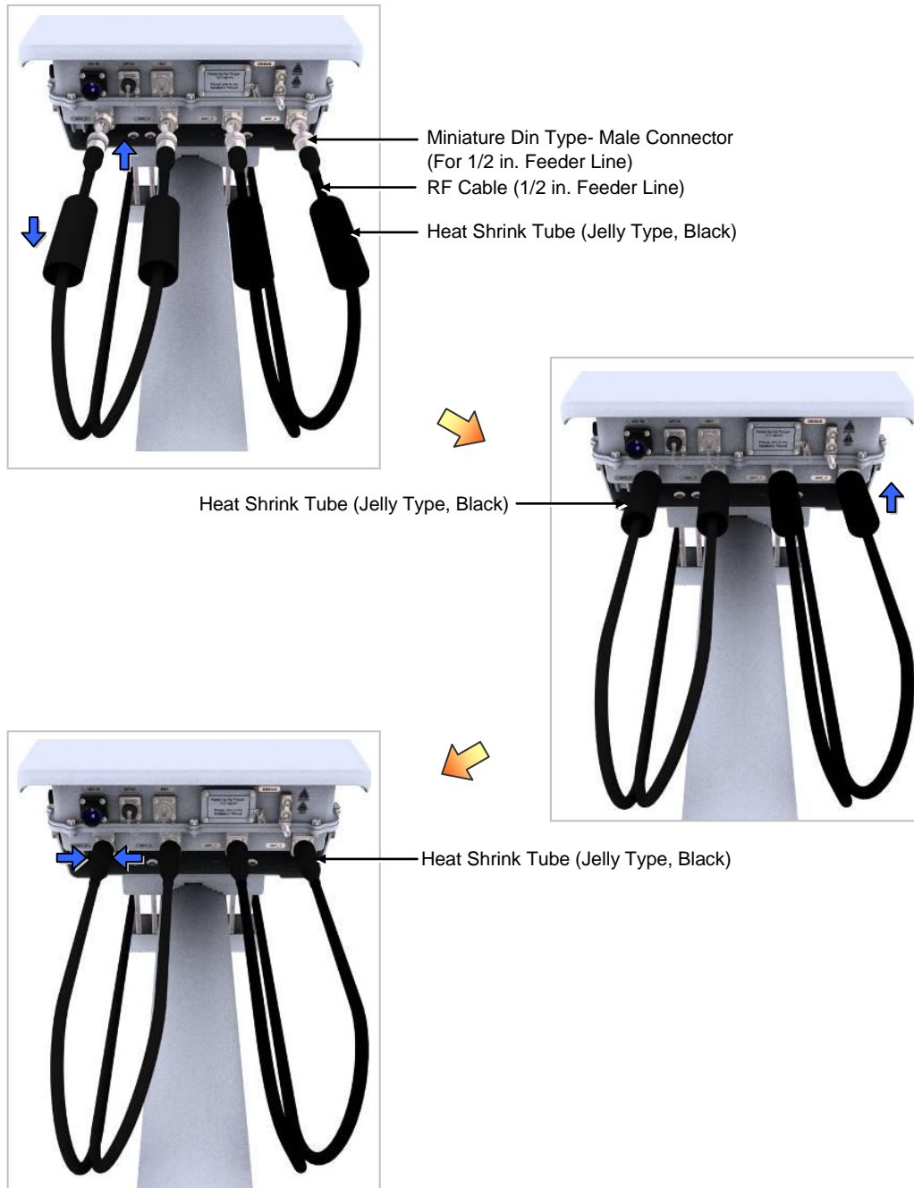
Figure 3.13 Connection of Feeder Cable (Detail A)
