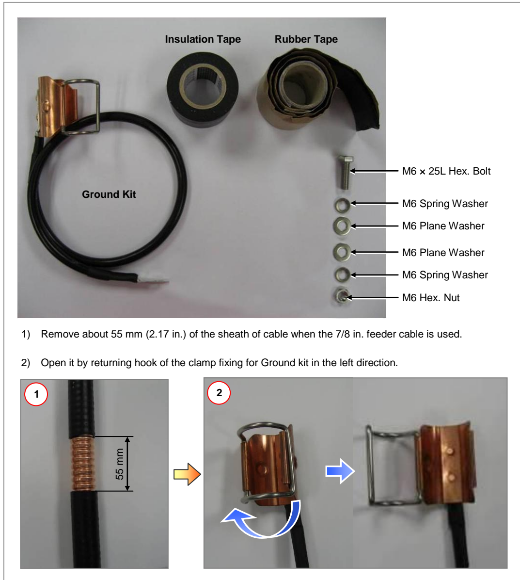
Figure B.1 Feeder Cable Grounding (1)
