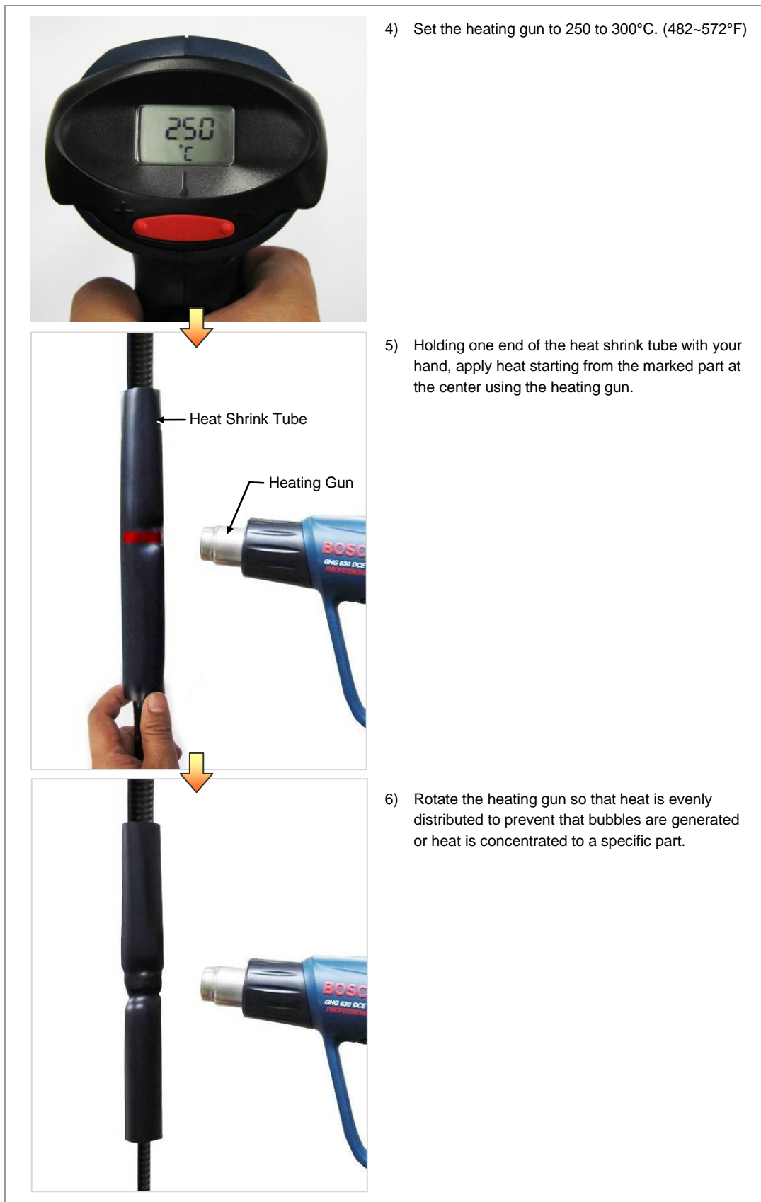
Figure C.11 Shrinking the Heat Shrink Tube_Connection between Connectors (2)
