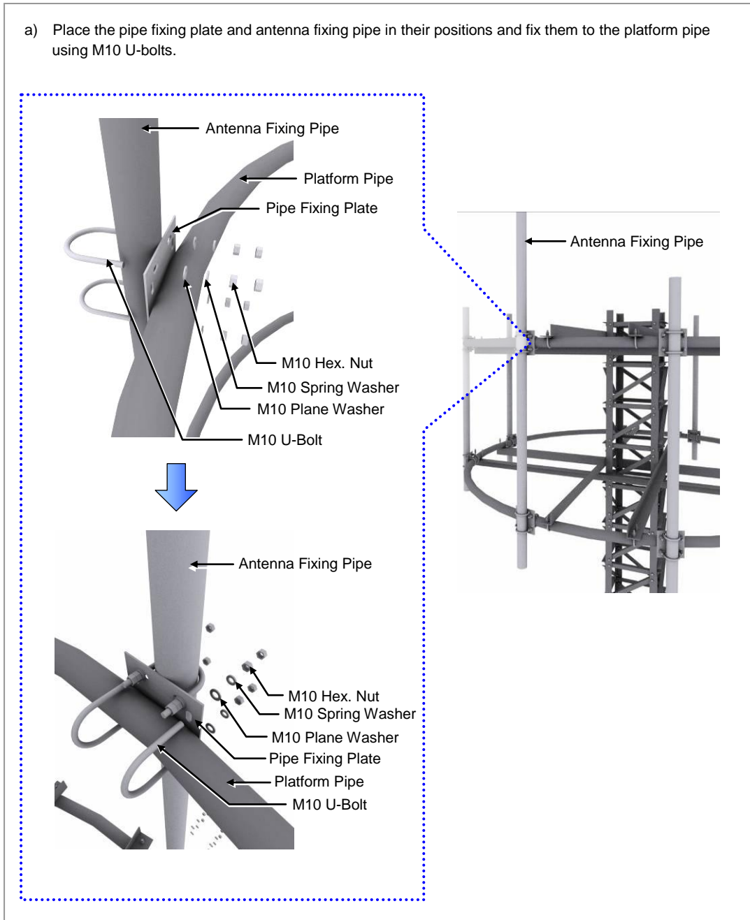
Figure 2.28 Fixing Tower Type RRH-2WB (7)
