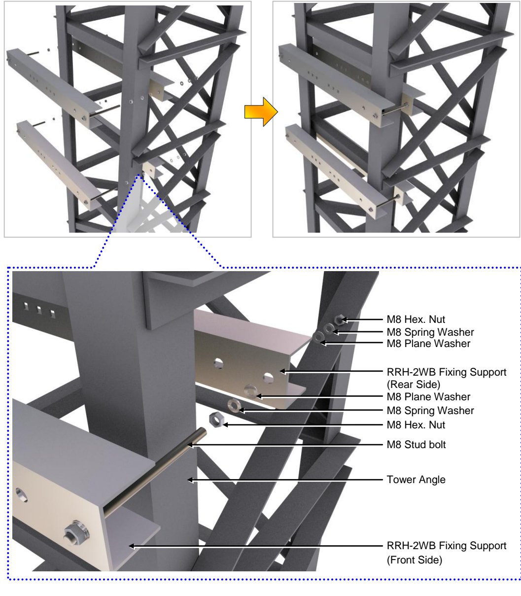
Figure 2.23 Fixing Tower Type RRH-2WB (2)
