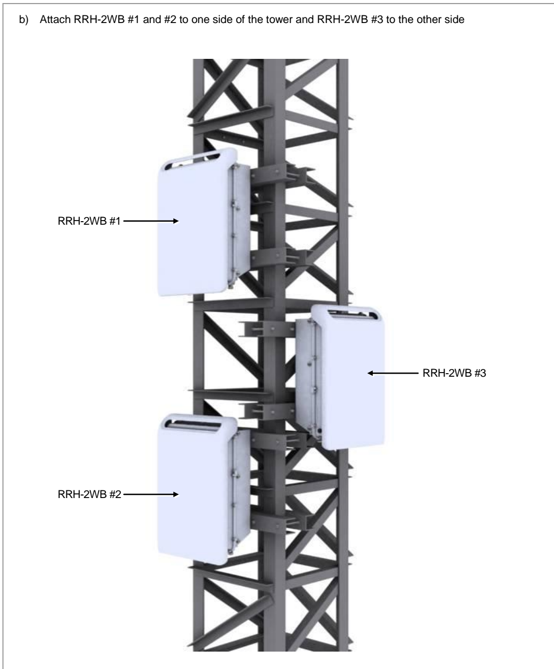
Figure 2.27 Fixing Tower Type RRH-2WB (6)
