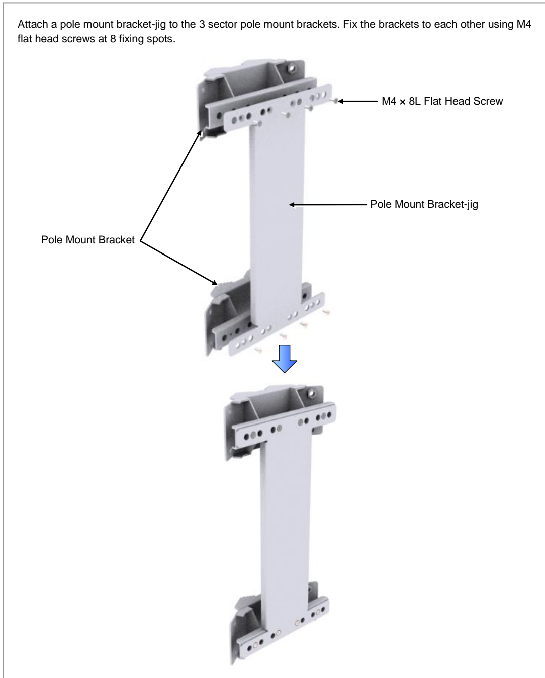
Figure 2.14 Fixing 3 Sector Pole Type RRH-2WB (1)
