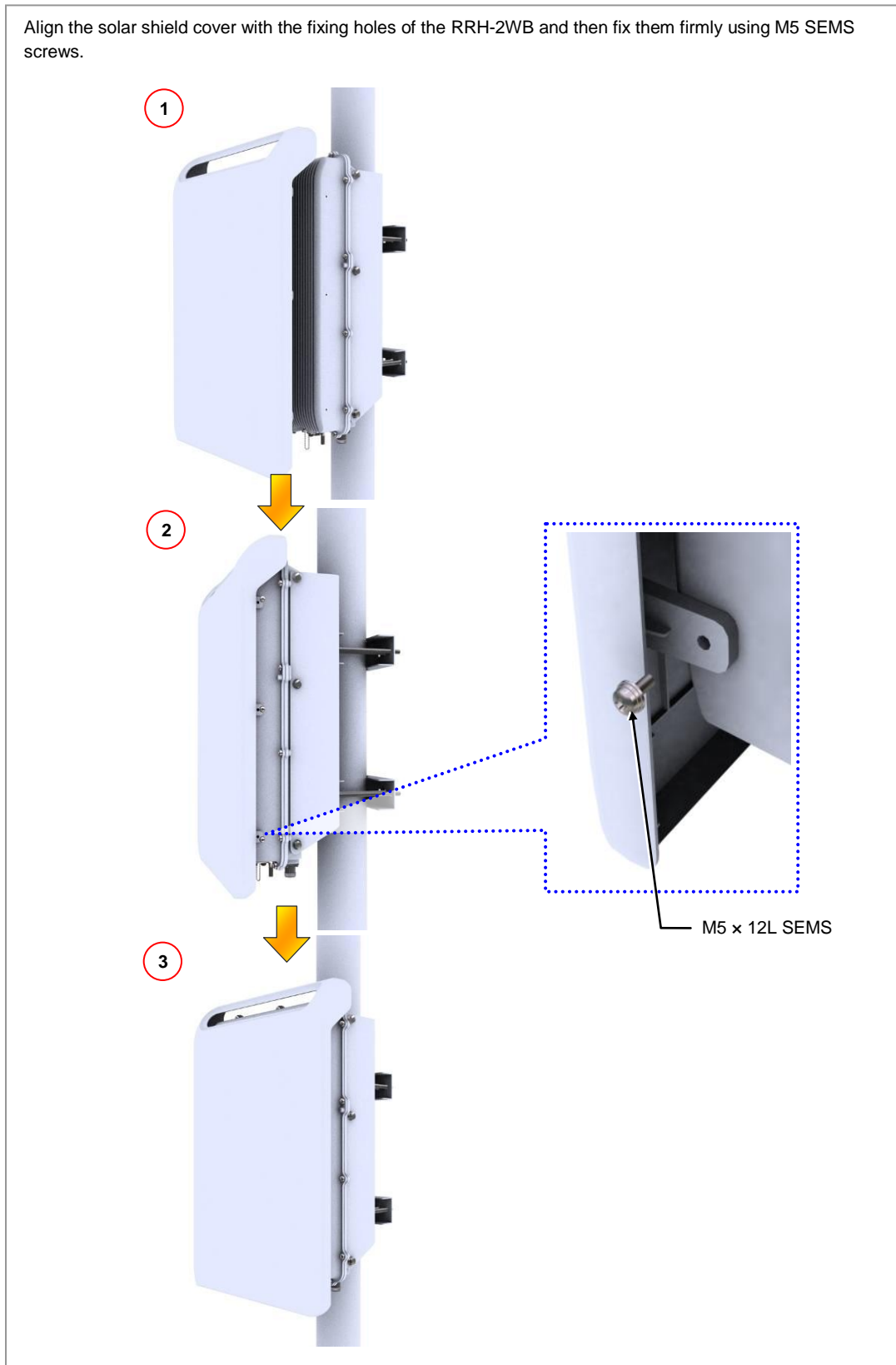
Figure 2.13 Fixing 1 Sector Pole Type RRH-2WB (3)
