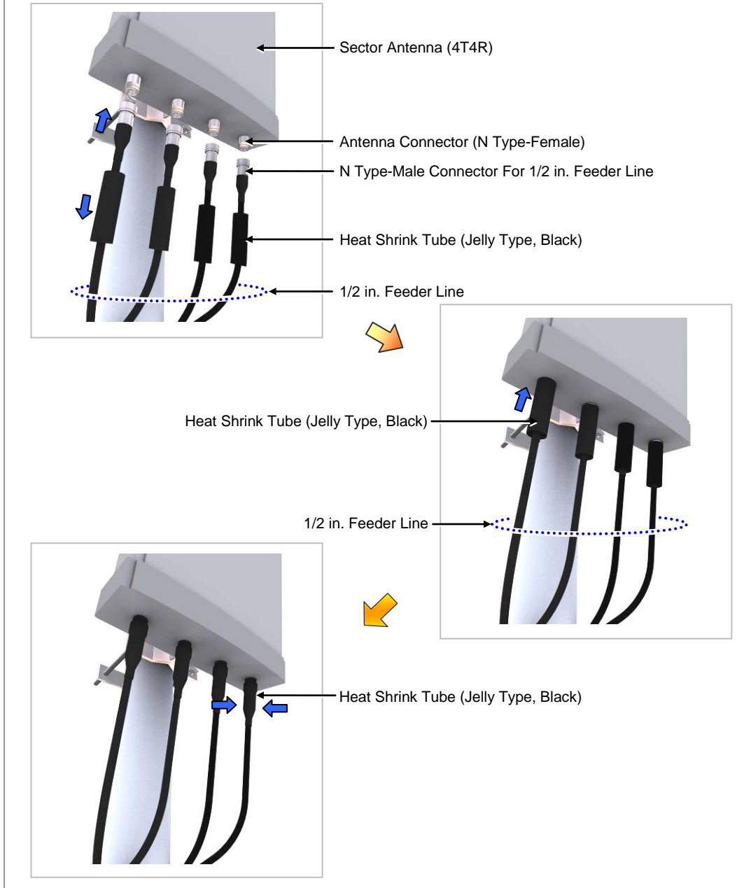
Figure 3.14 Connection of Feeder Cable (Detail B)
