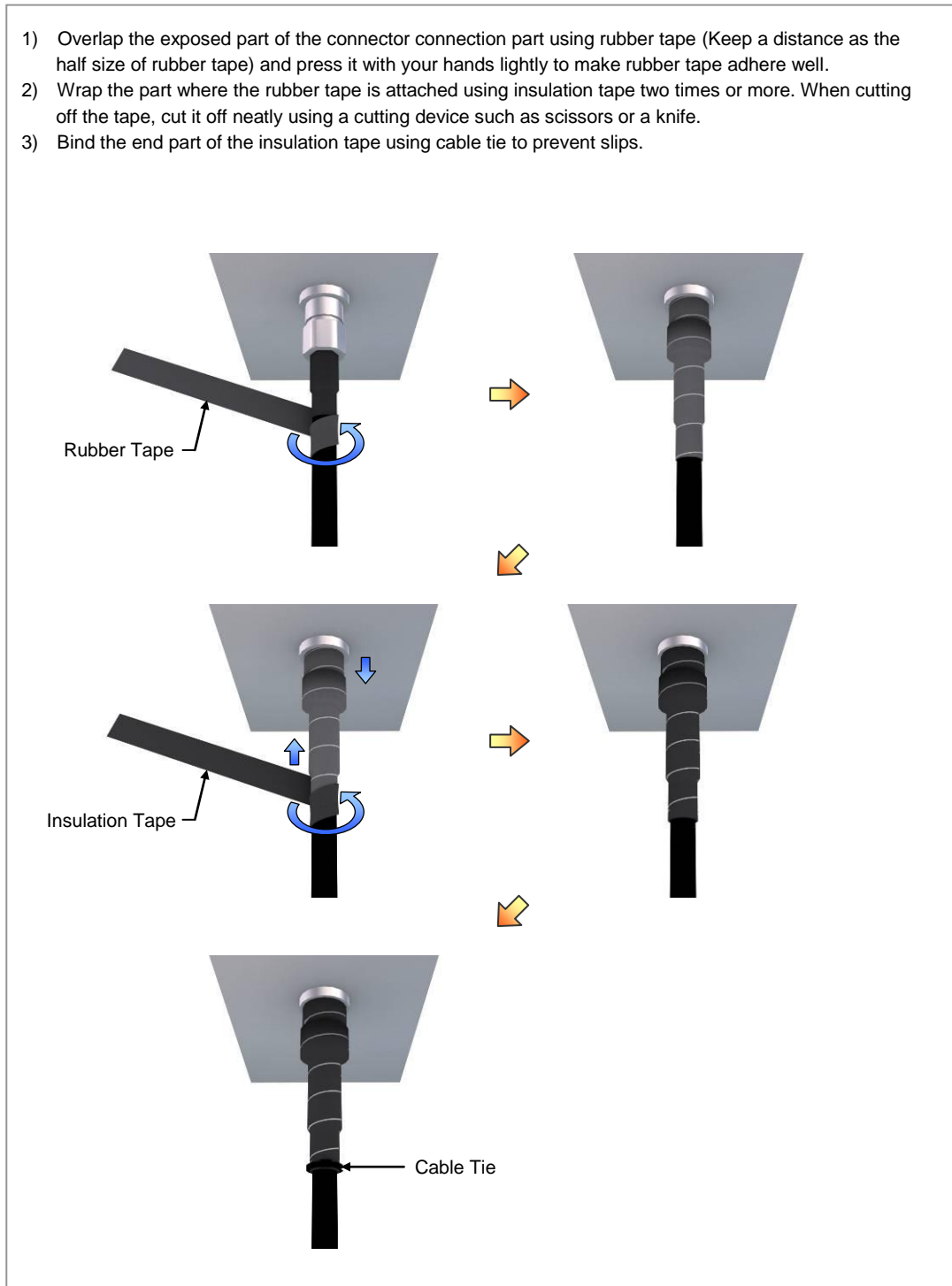
Figure C.7 Finishing the Connector Connection Part by Tape
