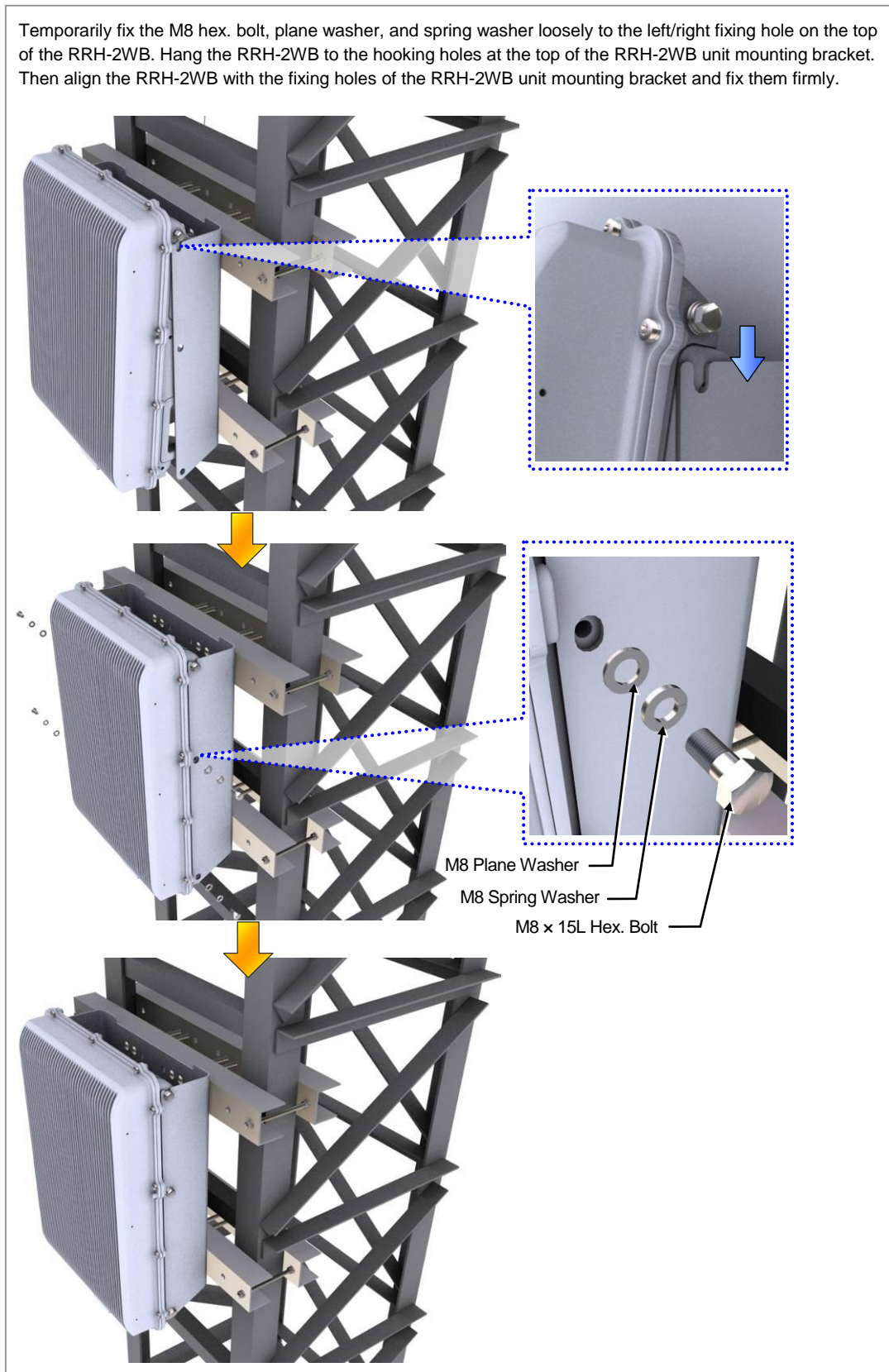
Figure 2.25 Fixing Tower Type RRH-2WB (4)
