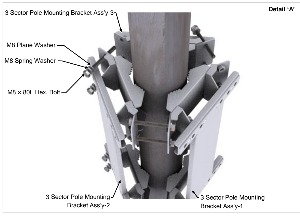
Figure 2.16 Fixing 3 Sector Pole Type RRH-2WB (3)
