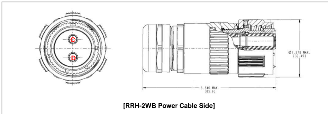
Figure 3.7 Power Cable Connector
