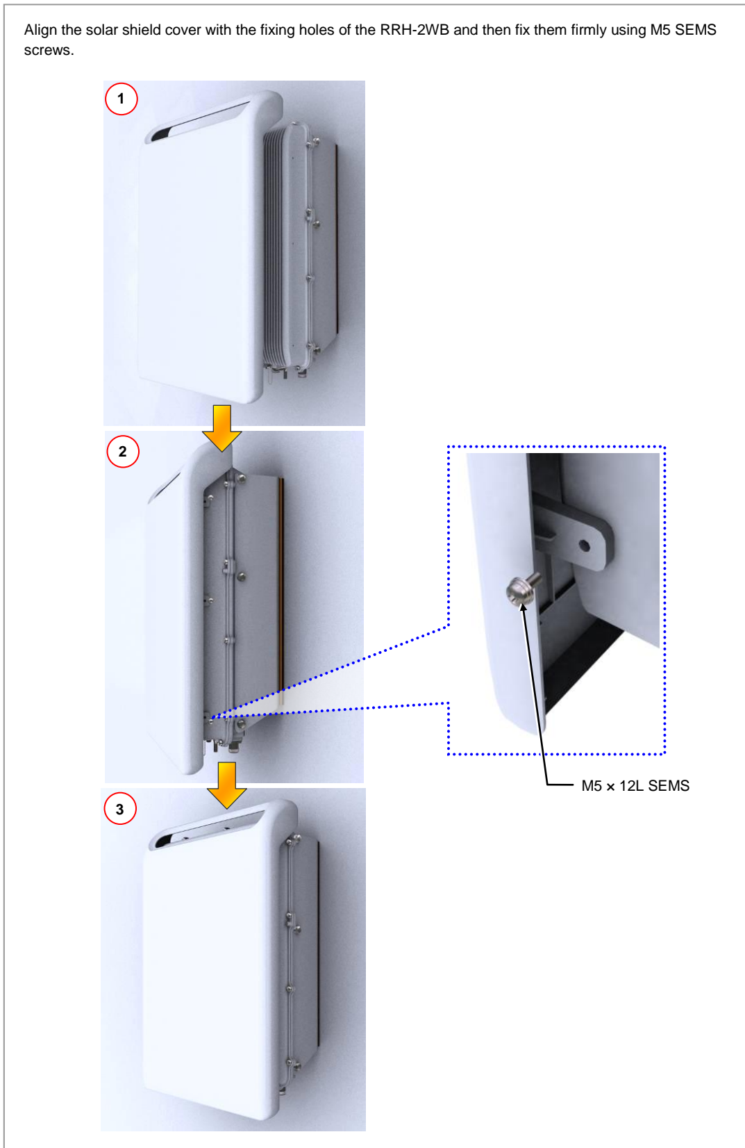
Figure 2.6 Fixing the RRH-2WB_Wall Type (3)
