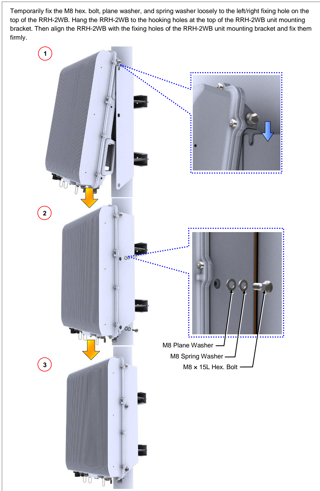
Figure 2.12 Fixing 1 Sector Pole Type RRH-2WB (2)
