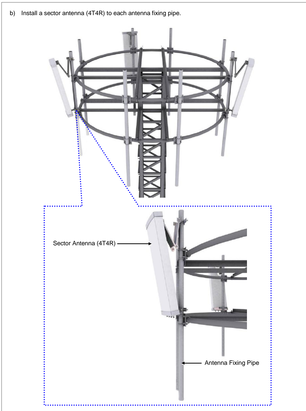
Figure 2.29 Fixing Tower Type RRH-2WB (8)
