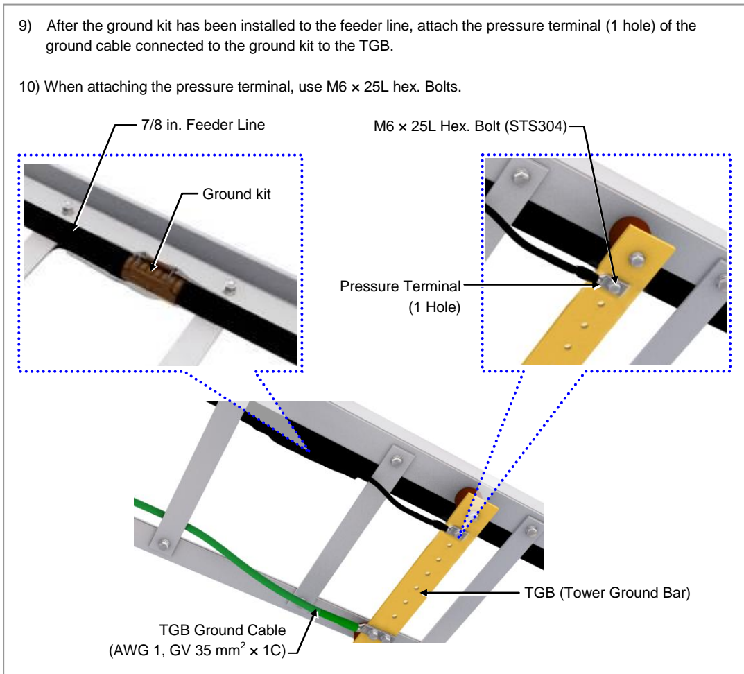
Figure B.4 Feeder Cable Grounding (4)
