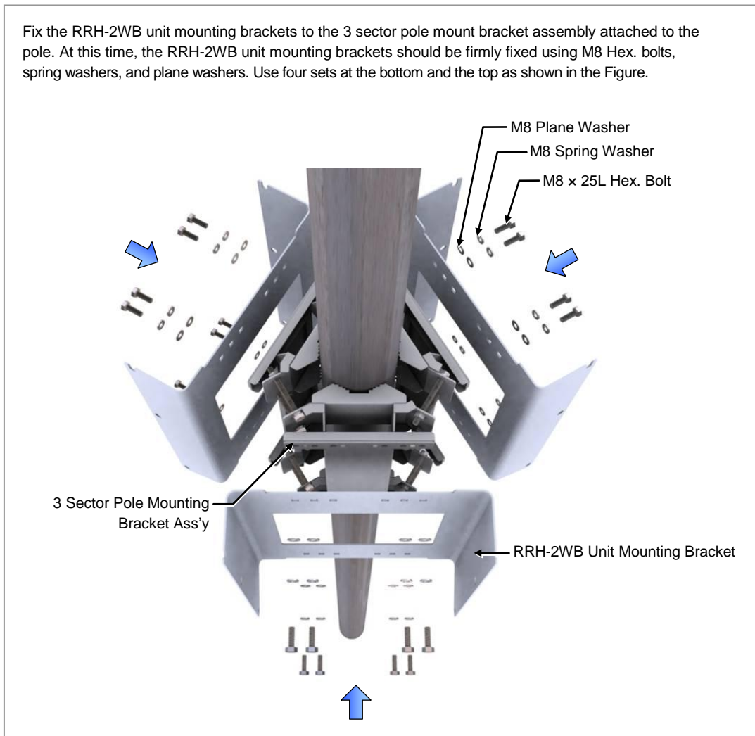
Figure 2.17 Fixing 3 Sector Pole Type RRH-2WB (4)
