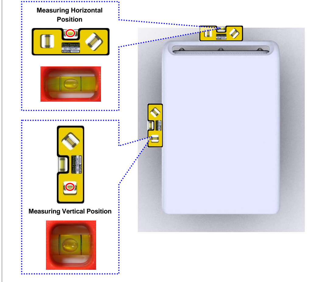
Figure 2.31 Leveling Test before Fixing System
