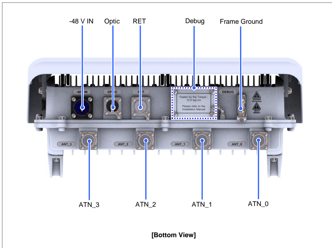
Figure 1.3 RRH-2WB External Interface
