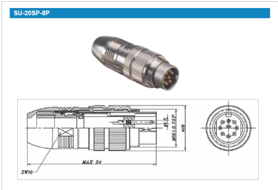
Figure 3.11 RET Cable Connector
