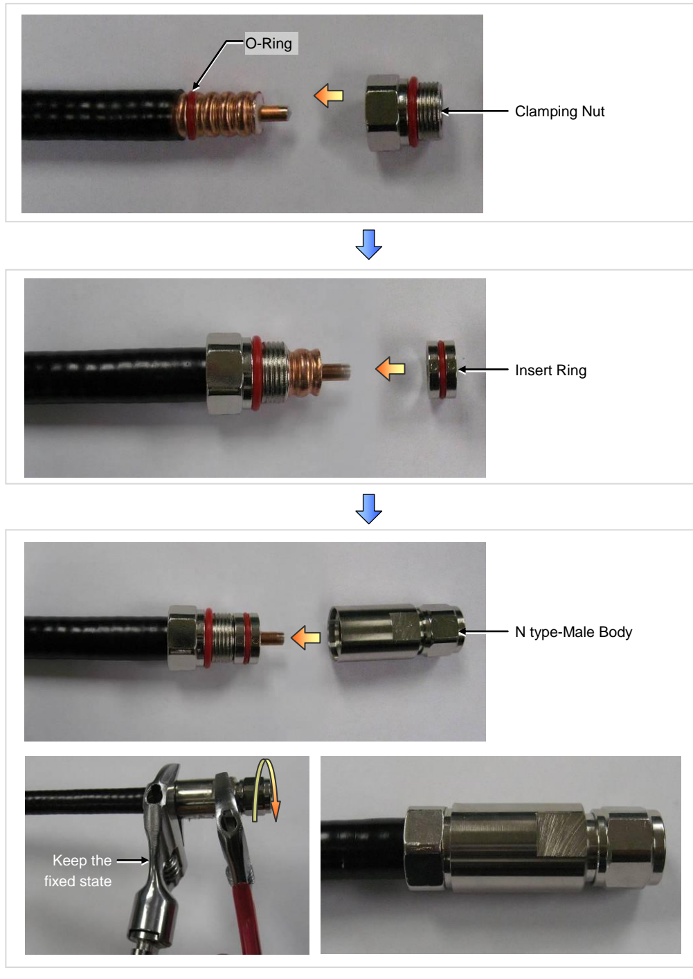
Figure C.3 Assembling the N type-male (1/2 in. Feeder Line) Connector (3)
