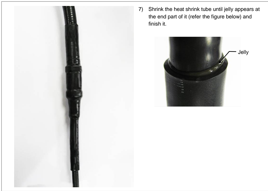
Figure C.12 Shrinking the Heat Shrink Tube_Connection between Connectors (3)
