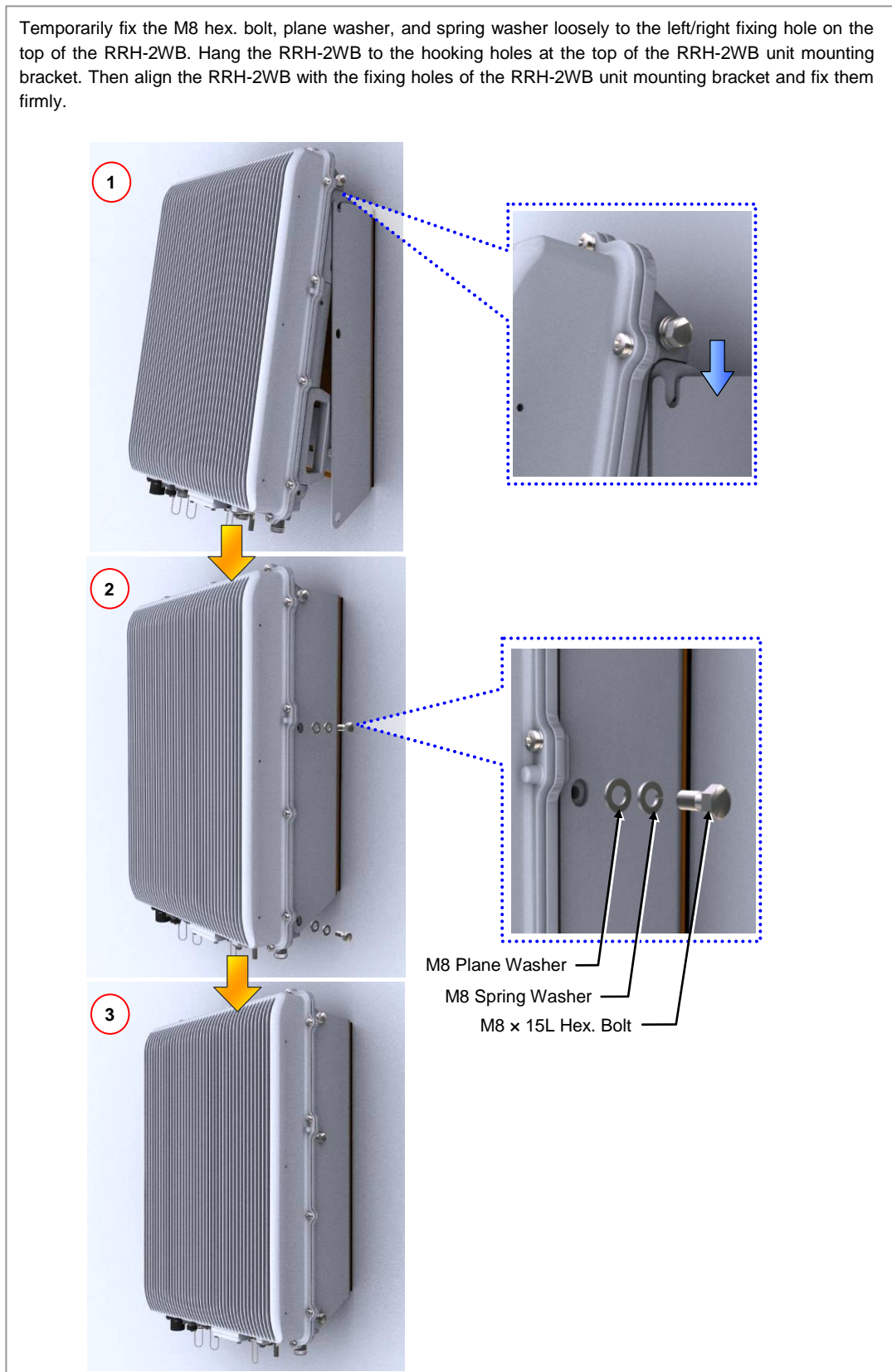
Figure 2.5 Fixing the RRH-2WB_Wall Type (2)
