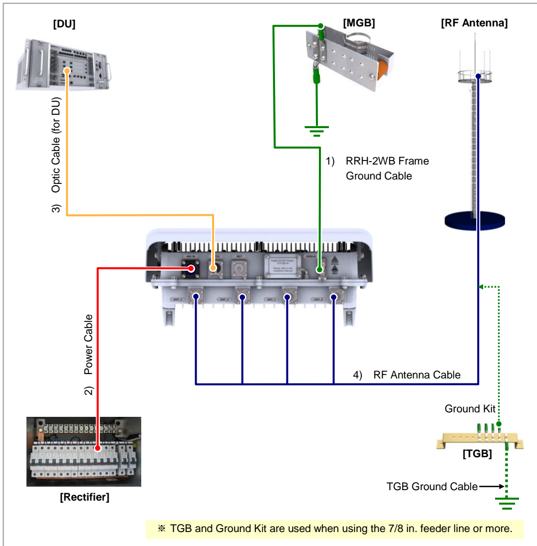
Figure 3.2 Cabling Diagram
