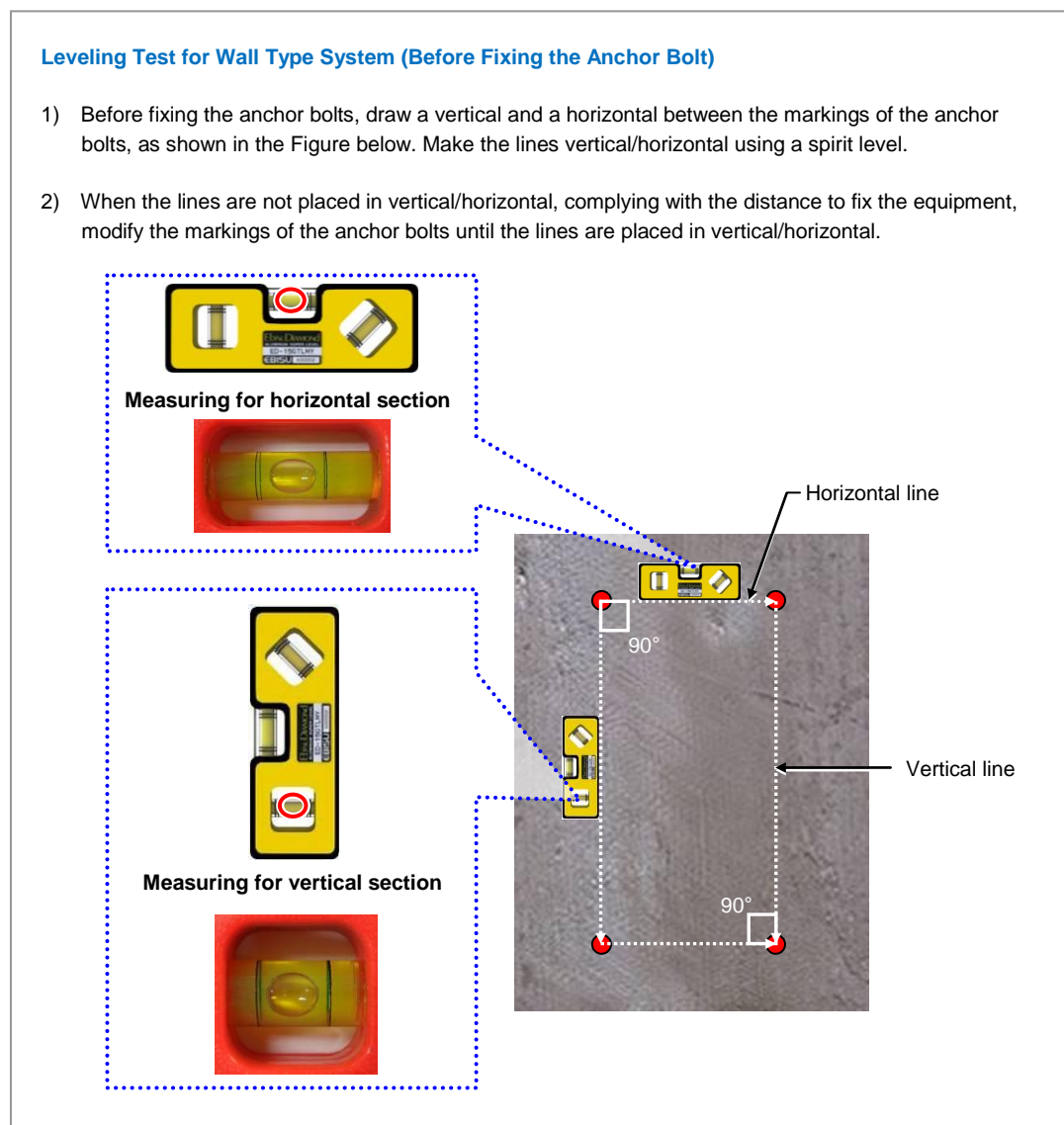
Figure 2.30 Leveling Test before Fixing Anchor Bolts
