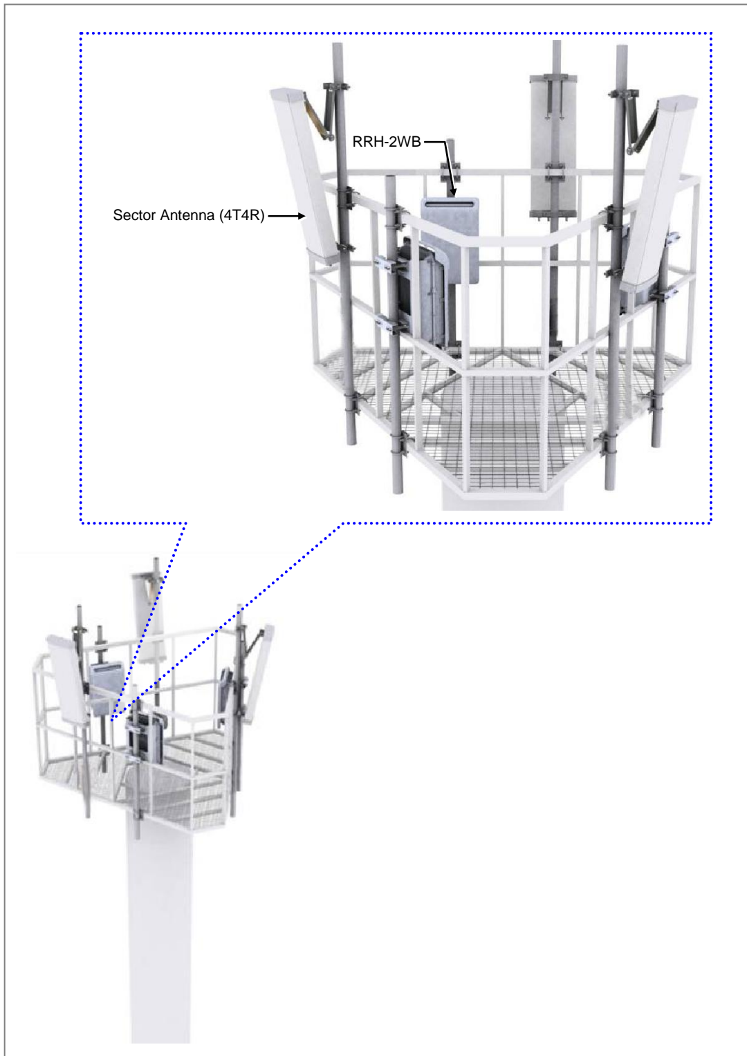
Figure 2.8 Example of Installing on Mono Pole
