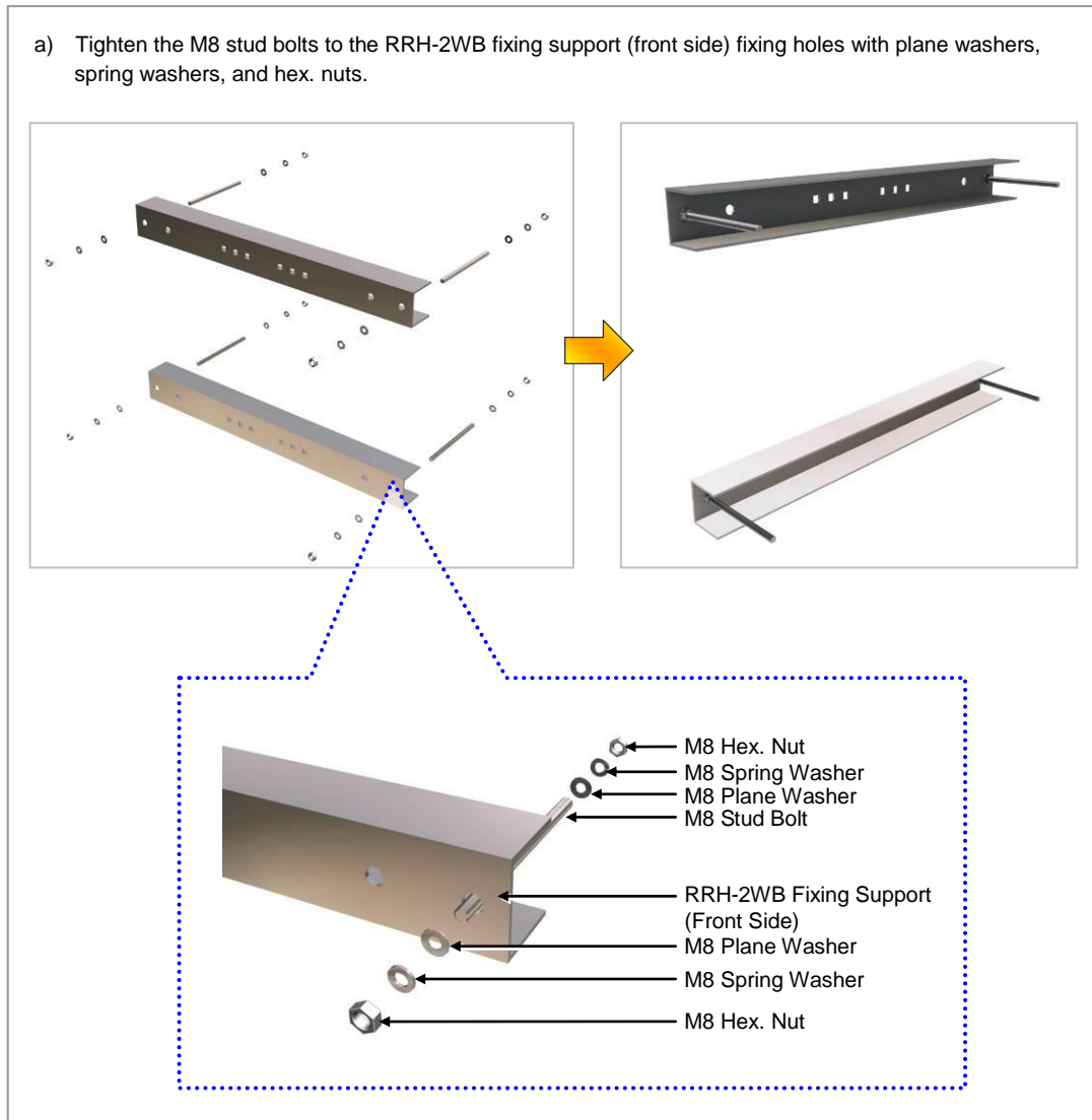
Figure 2.22 Fixing Tower Type RRH-2WB (1)
