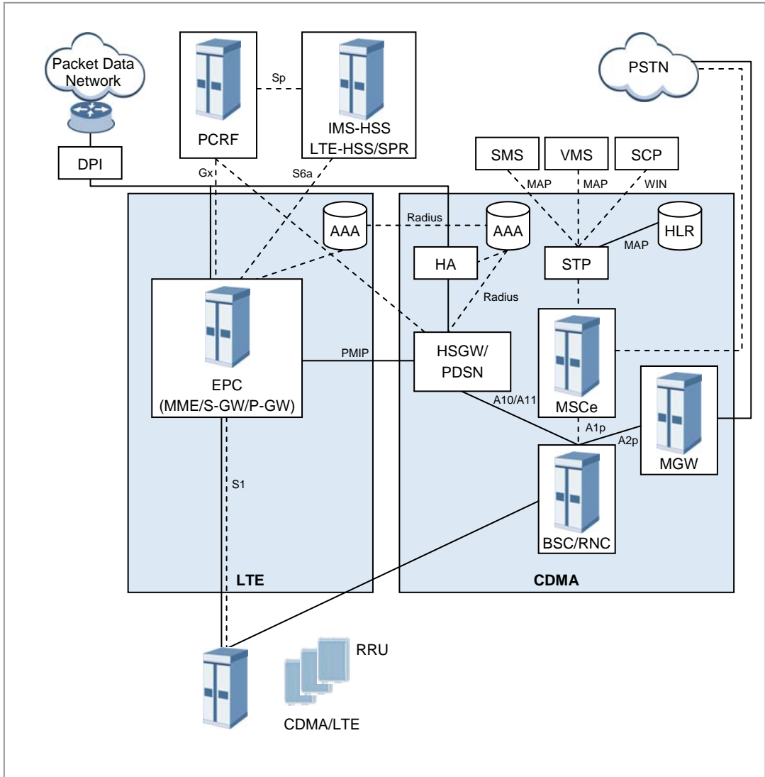
Figure 1.2 Samsung Multi-modal Network Architecture
