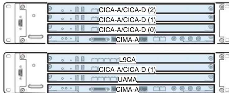
Figure 3.12 UADU Configuration - CDMA+LTE Dual Mode(Two UADU)
