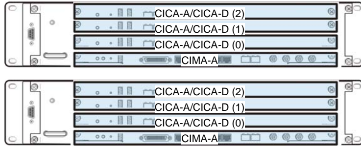
Figure 3.9 UADU Configuration - CDMA Only(Two UADU)
