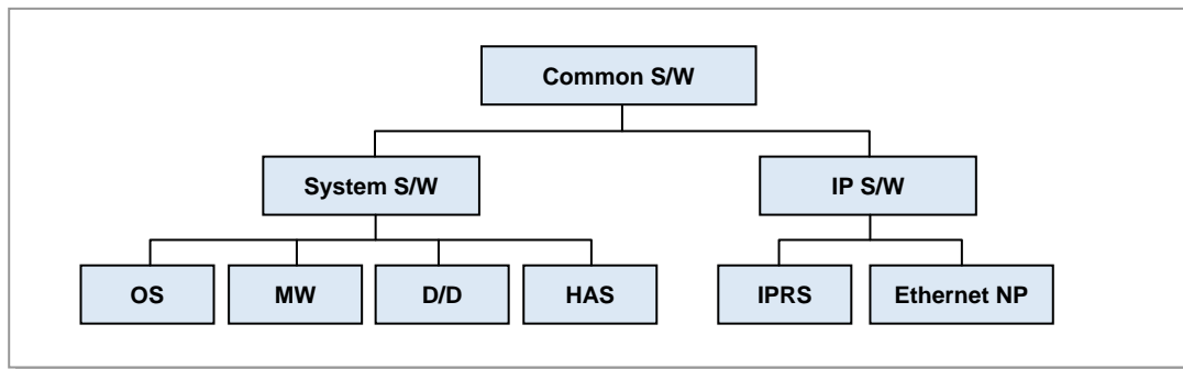
Figure 4.2 CDMA Common Software Architecture
