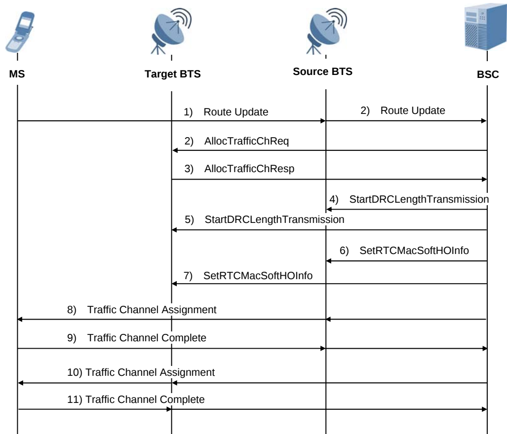
Figure 4.14 1xEV-DO soft handoff
