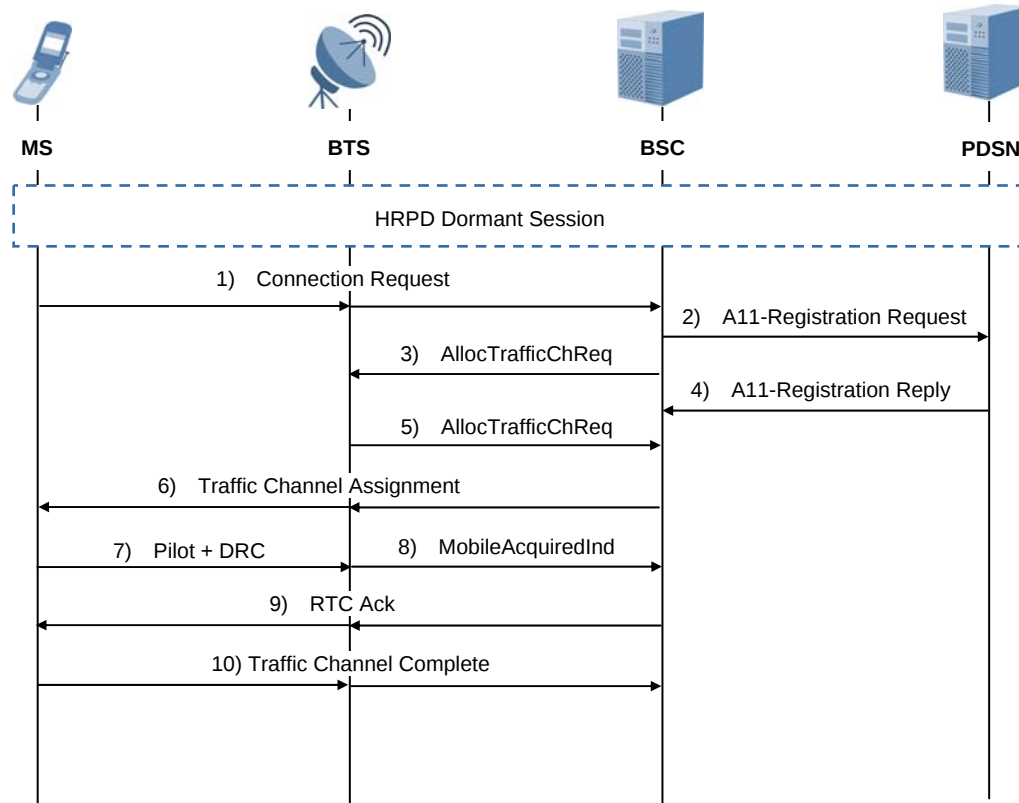
Figure 4.11 Transition from 1xEV-DO Dormant status to the Active state by MS
