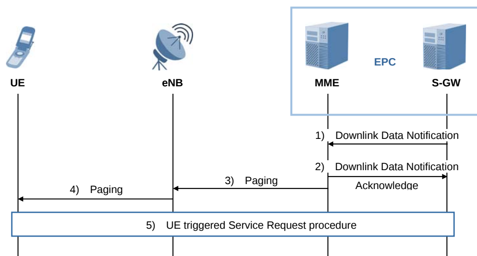
Figure 4.17 Service Request Process by Network
