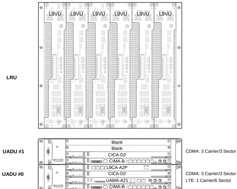
Figure 3.4 CDMA/LTE 6 Sector Configuration
