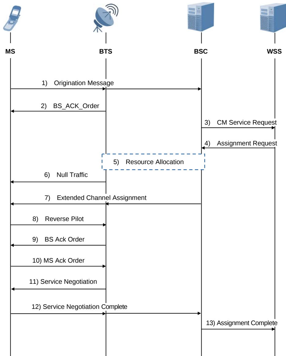
Figure 4.1 1X voice call origination
