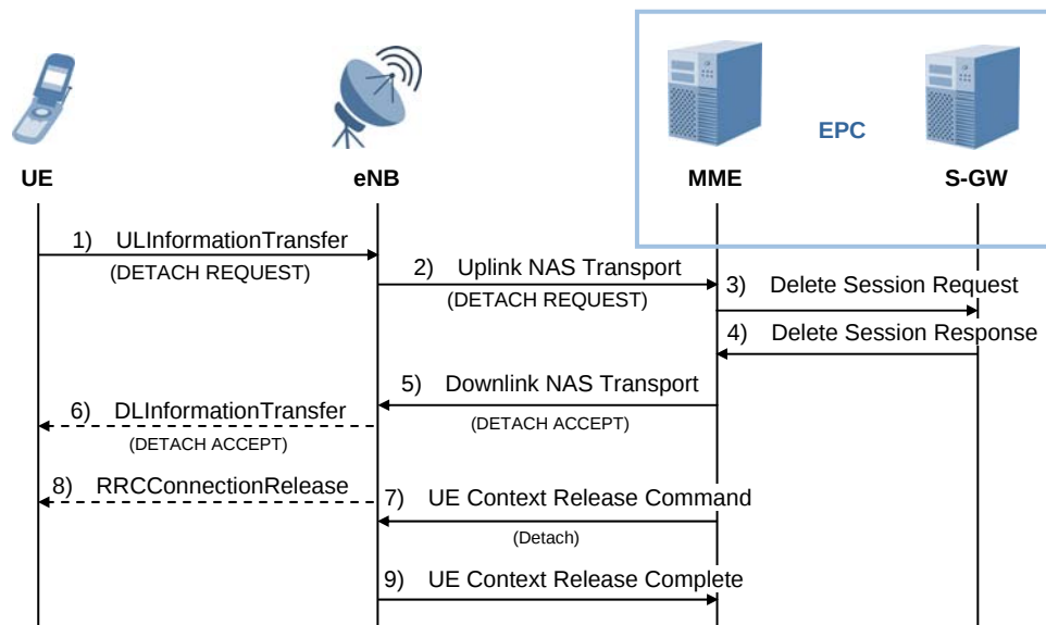
Figure 4.18 Detach Process by UE
