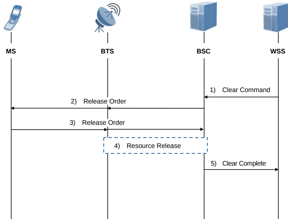
Figure 4.7 1X call release by WSS
