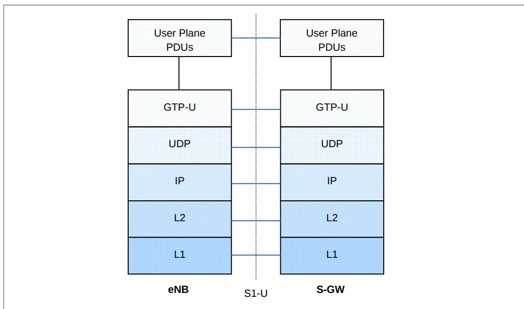
Figure 2.6 Protocol Stack between eNB and EPC
