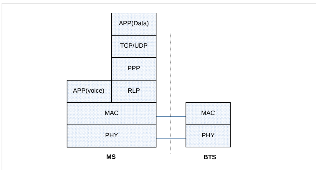
Figure 2.1 Protocol Stack between BTS and MS
