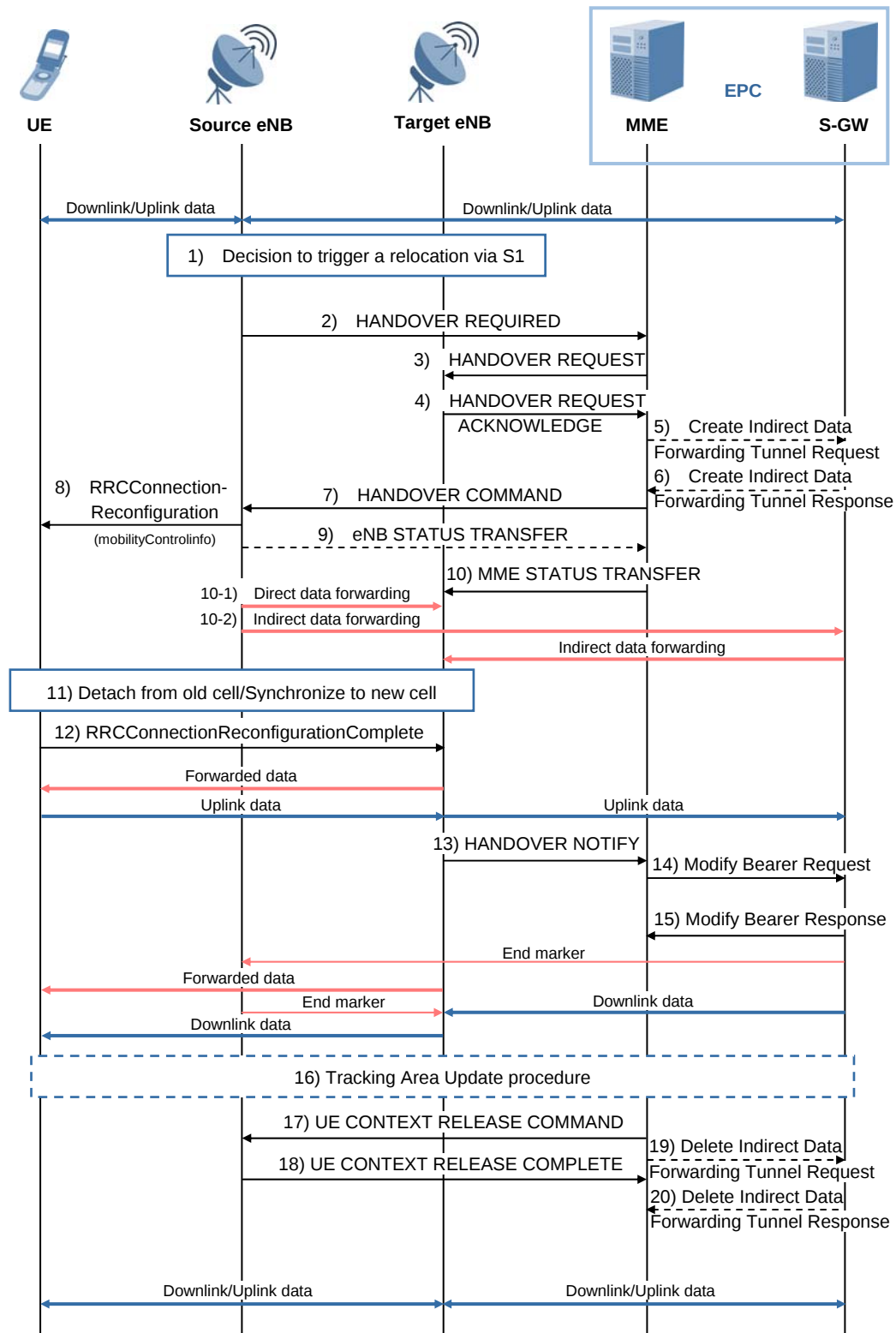
Figure 4.21 S1-based Handover Procedure
