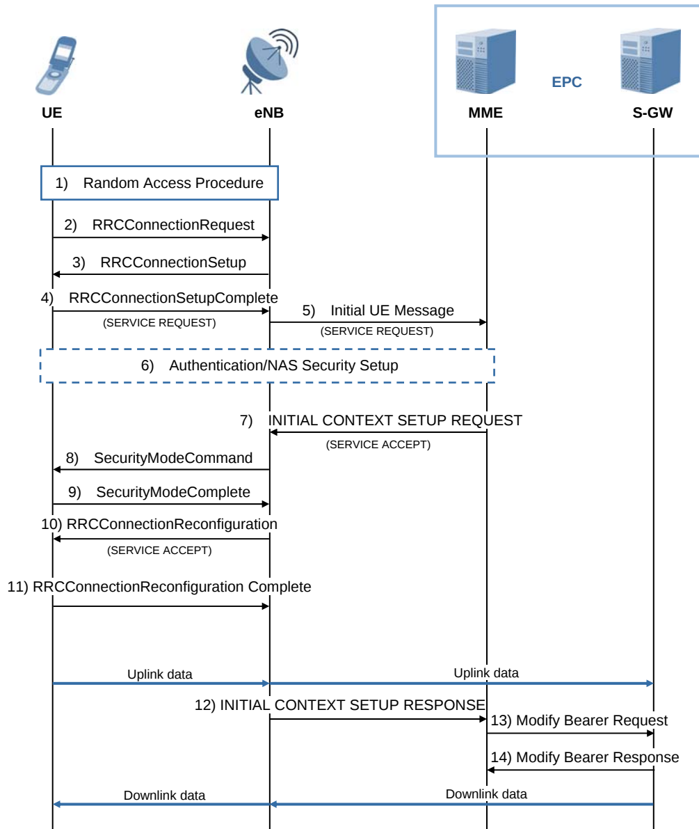
Figure 4.16 Service Request Process by UE
