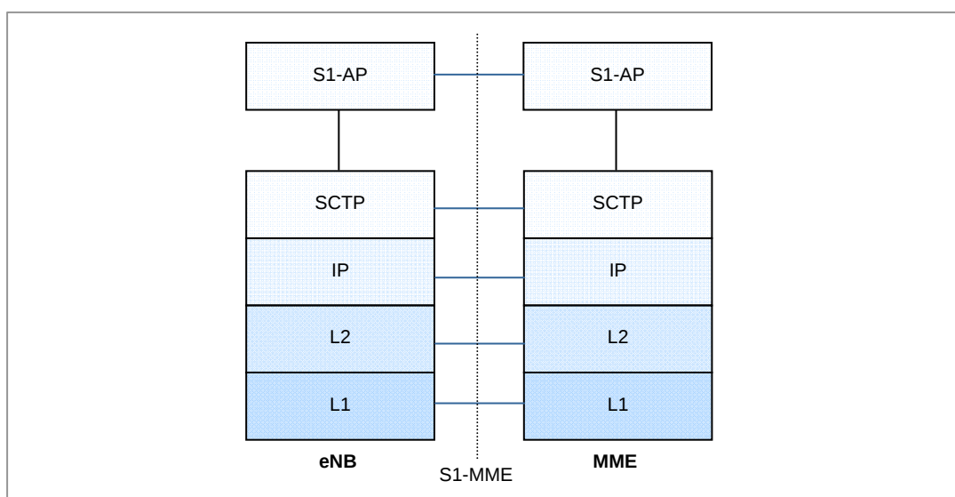
Figure 2.7 Protocol Stack between eNB and MME
