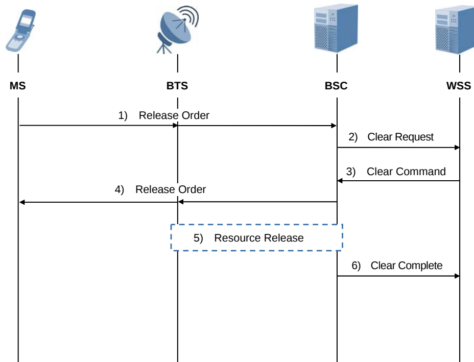
Figure 4.6 1X call release by MS
