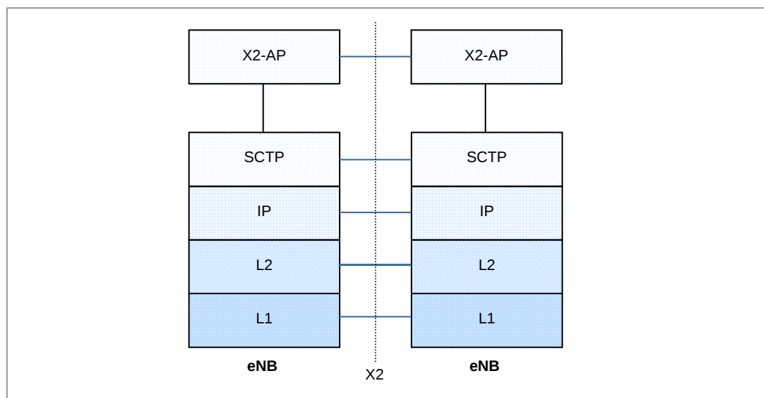
Figure 2.9 Protocol Stack between eNBs (Control Plane)
