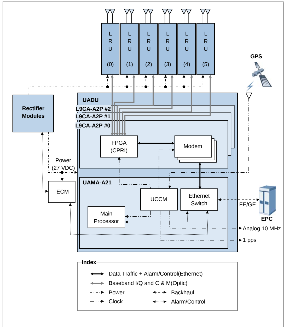
Figure 3.6 Internal Configuration of System (LTE)
