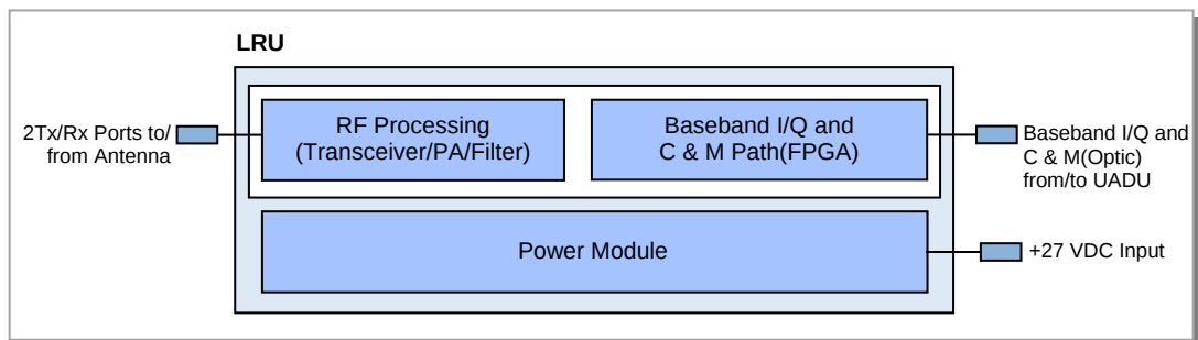
Figure 3.13 Hardware Interface structure of LRU-C2
