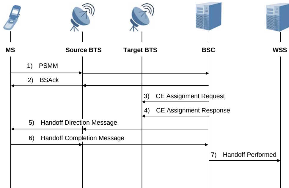
Figure 4.5 1X voice call soft handoff
