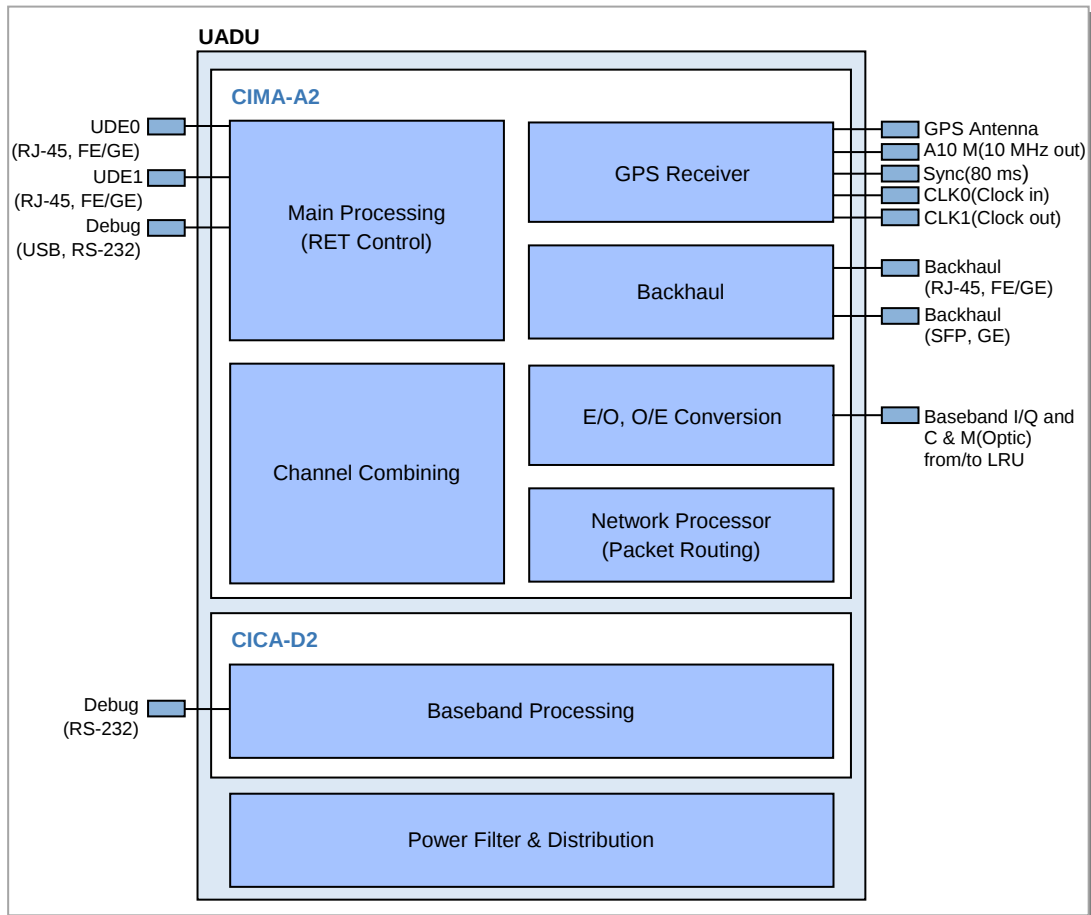
Figure 3.11 Hardware Interface structure of UADU (CDMA)
