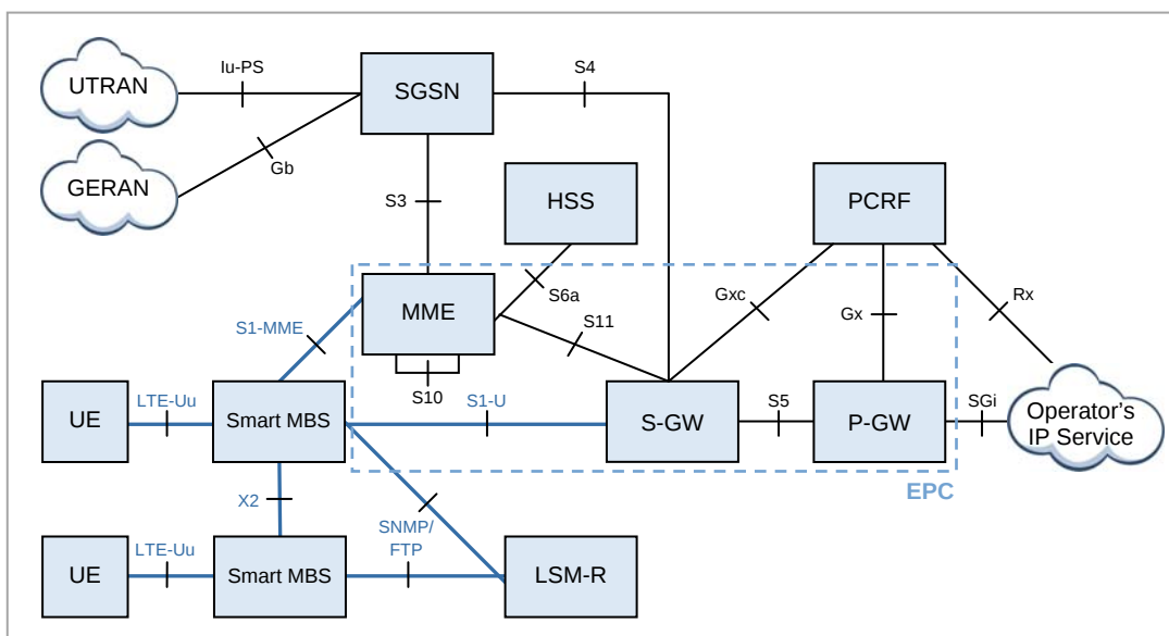
Figure 2.4 LTE Interface Structure
