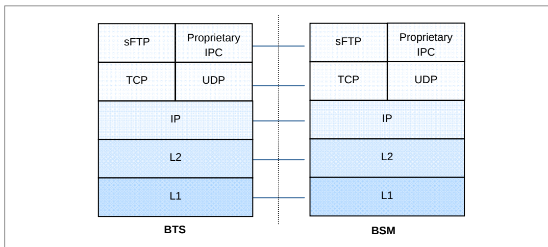
Figure 2.3 Protocol Stack between BTS and BSM
