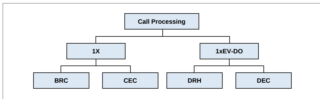
Figure 3.15 CDMA Call Processing Software Structure
