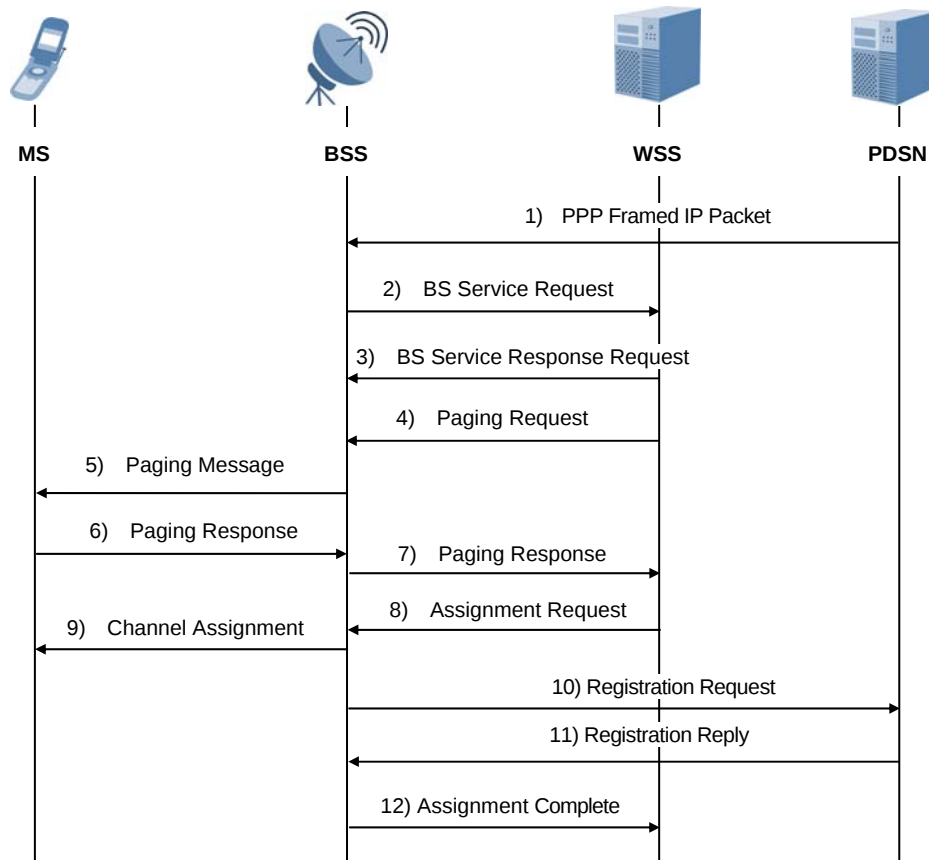
Figure 4.4 1X packet data call termination
