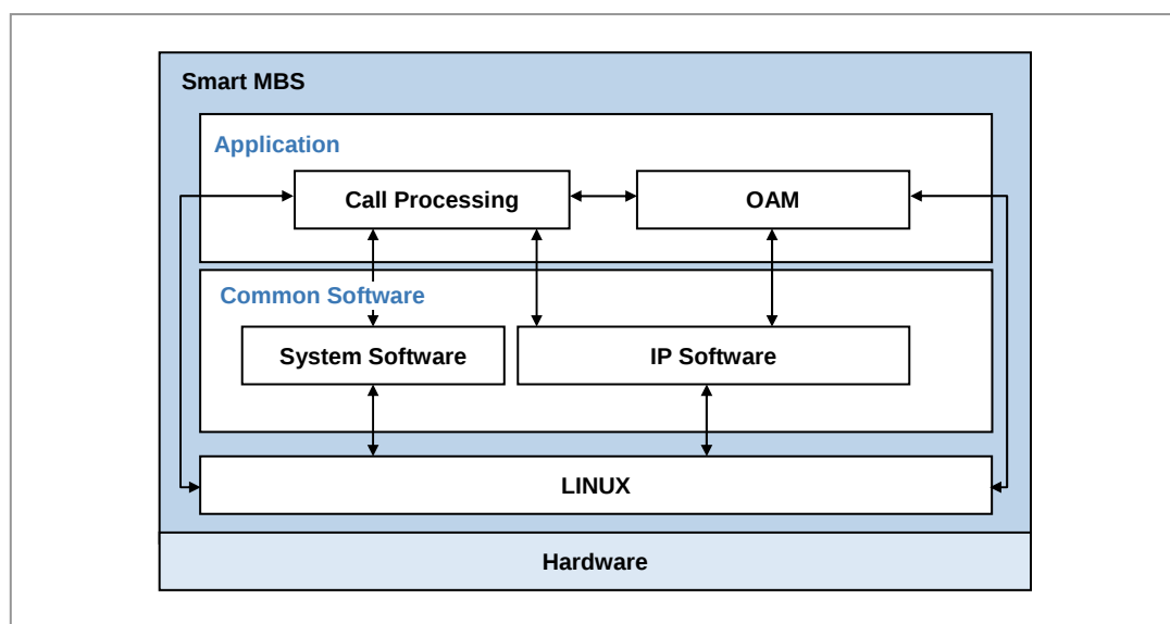
Figure 3.14 CDMA Software Structure
