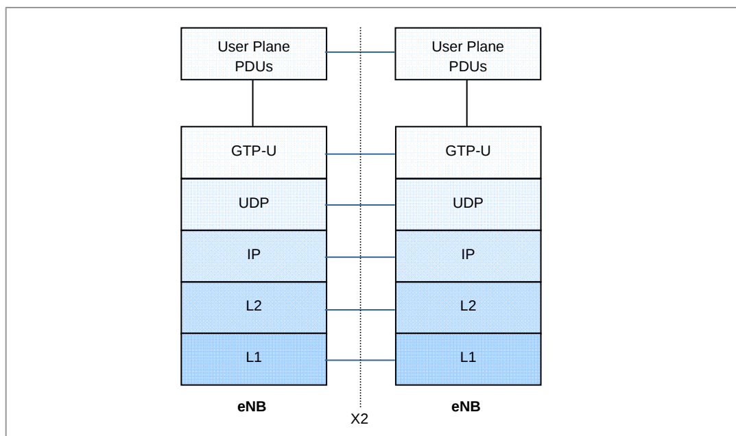
Figure 2.8 Protocol Stack between eNBs (User Plane)
