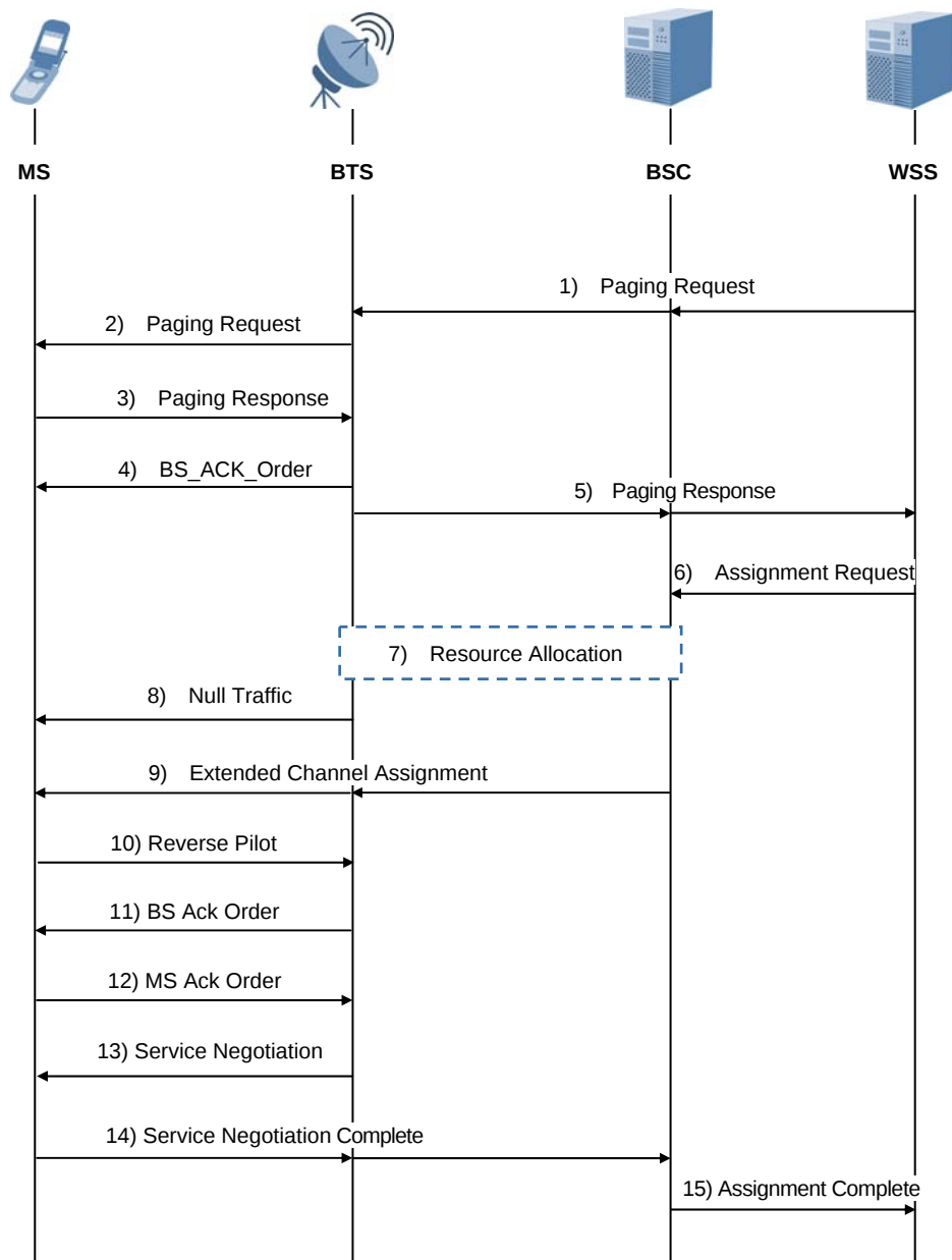
Figure 4.2 1X voice call termination
