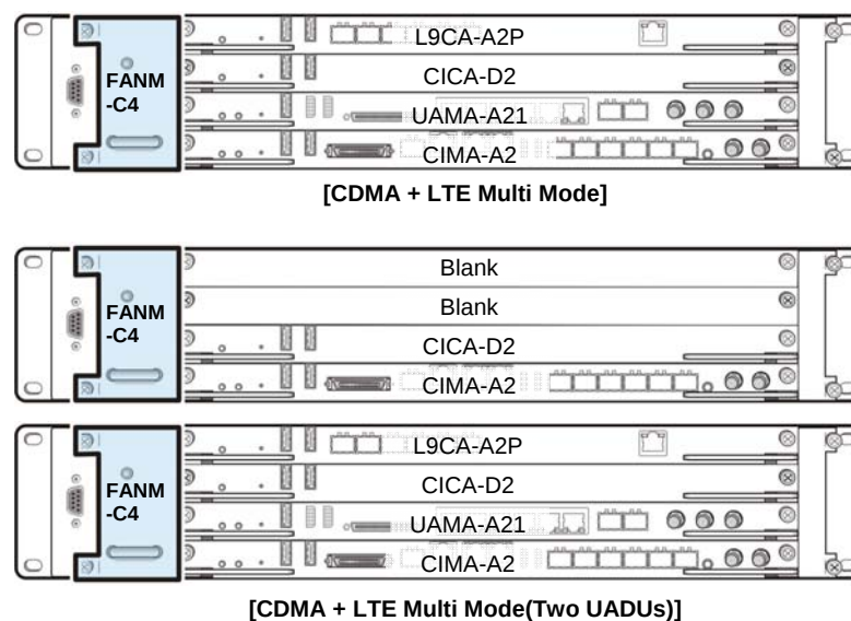
Figure 3.7 UADU Configuration
