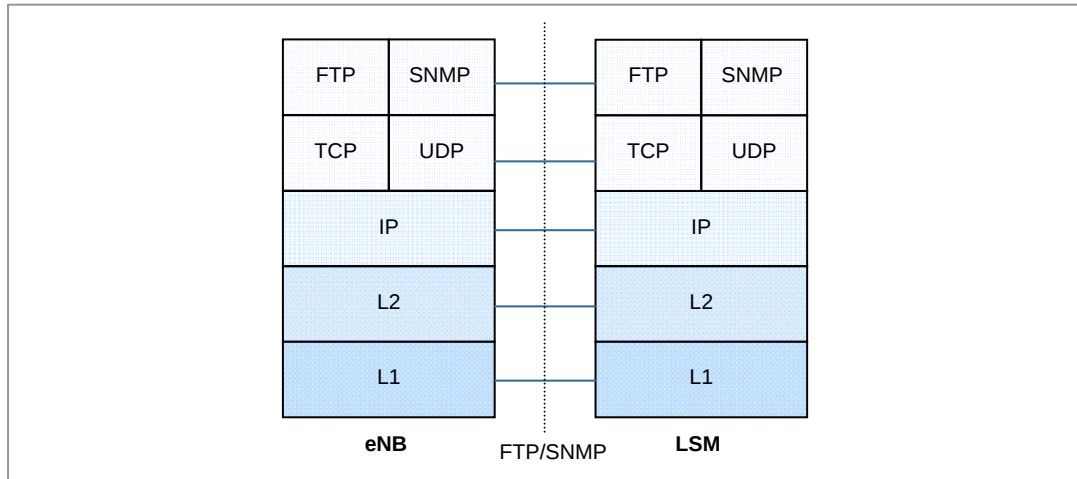
Figure 2.10 Protocol Stack between eNB and LSM
