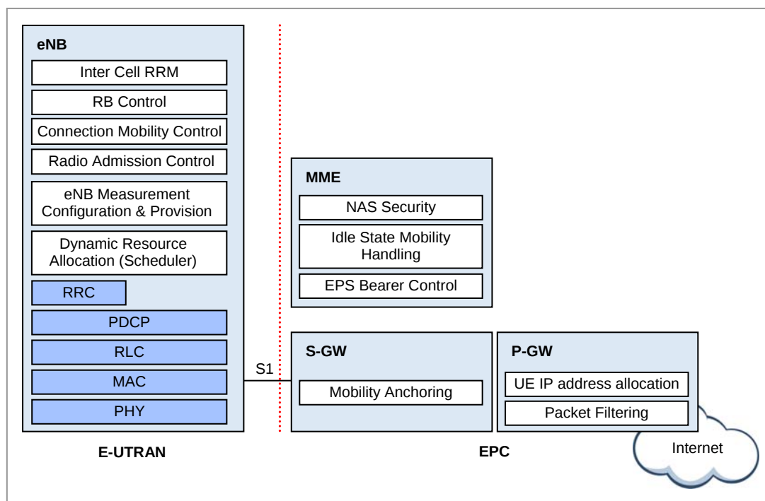
Figure 1.5 Functions of E-UTRAN and EPC
