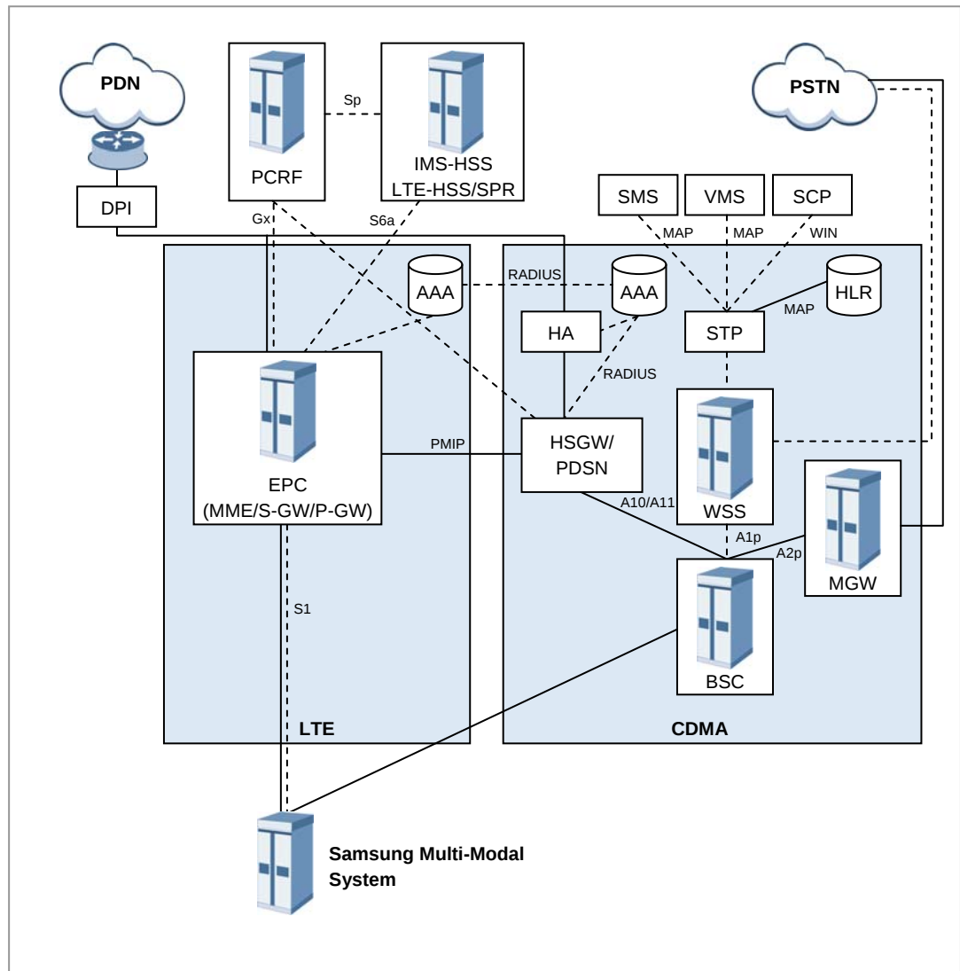
Figure 1.1 Network Configuration of Samsung Multi-Modal System
