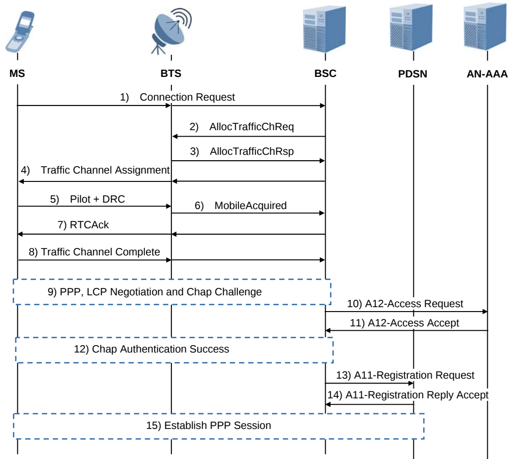
Figure 4.9 1xEV-DO MS authentication and PPP setup
