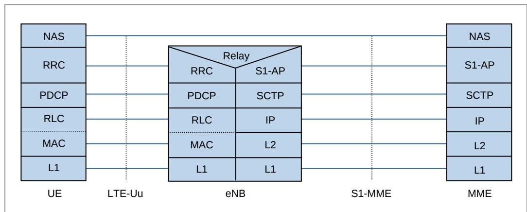
Figure 2.5 Protocol Stack between UE and eNB
