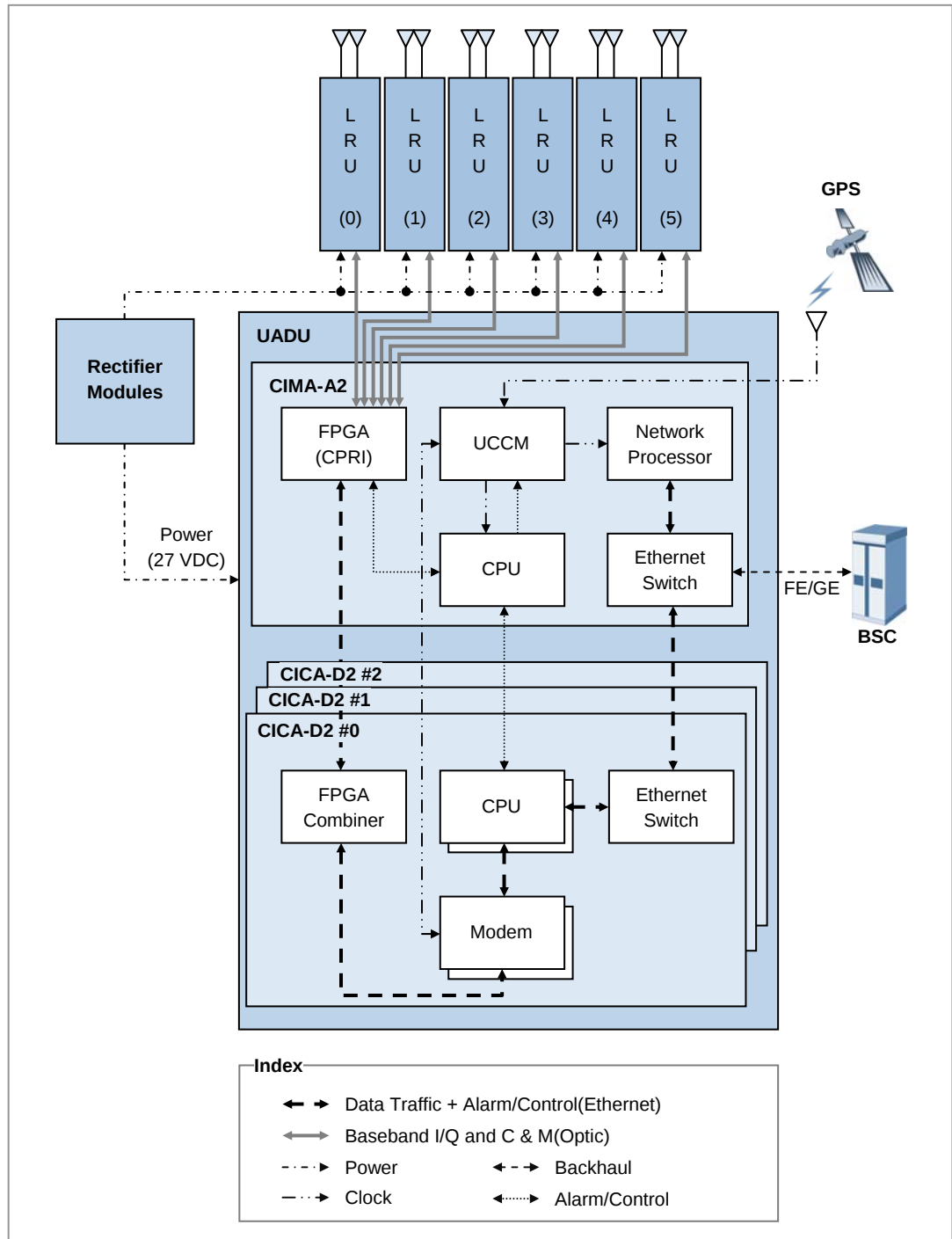
Figure 3.5 Internal Configuration of System (CDMA)
