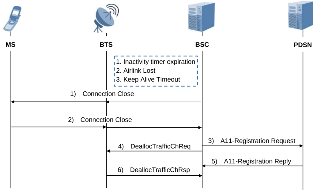
Figure 4.10 Transition to the 1xEV-DO Dormant state
