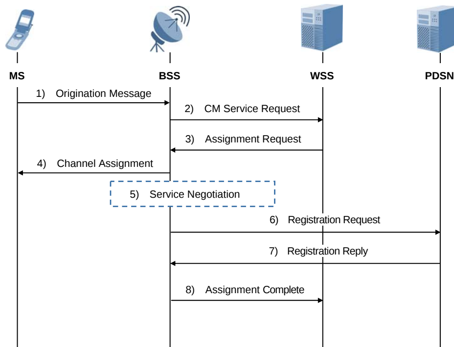
Figure 4.3 1X packet data call origination
