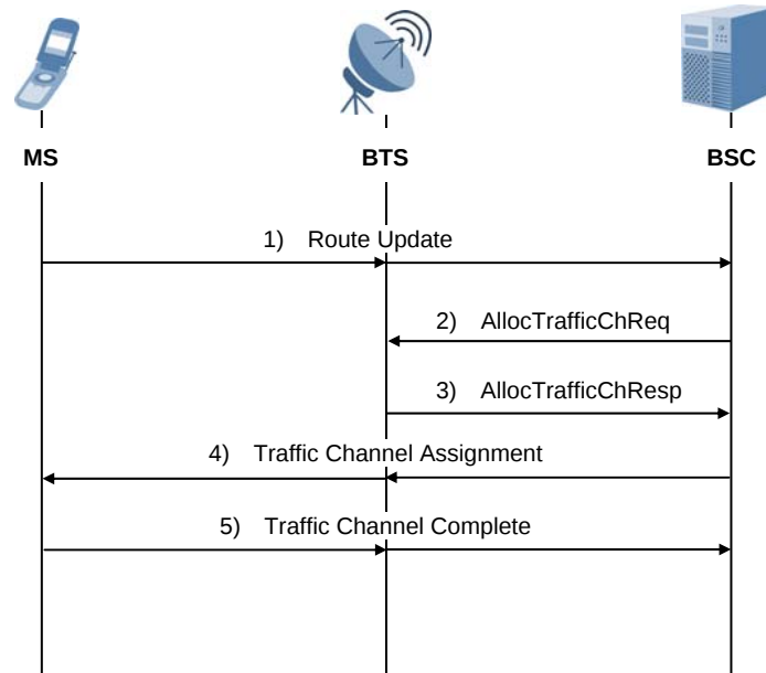
Figure 4.13 1xEV-DO softer handoff
