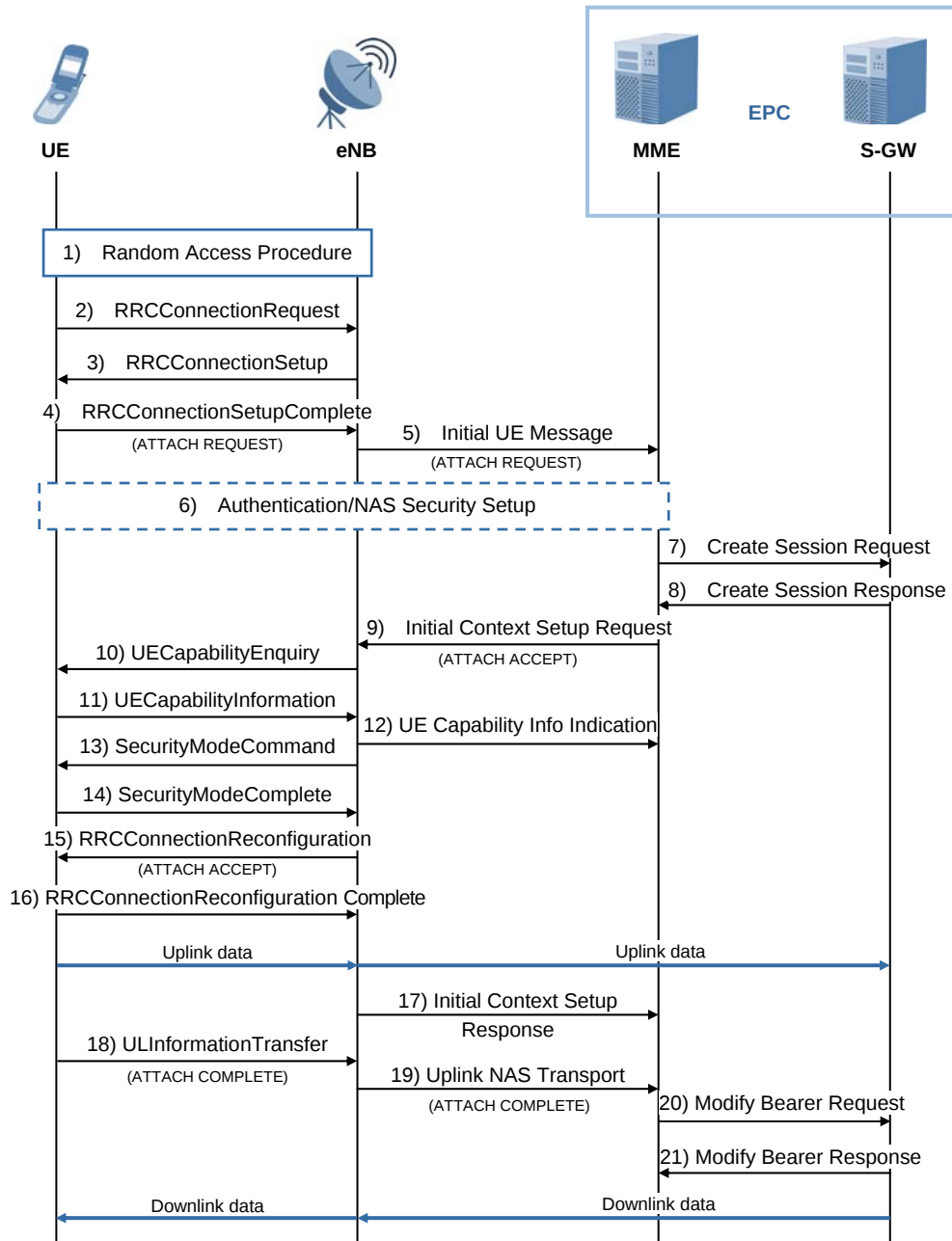
Figure 4.15 Attach Process
