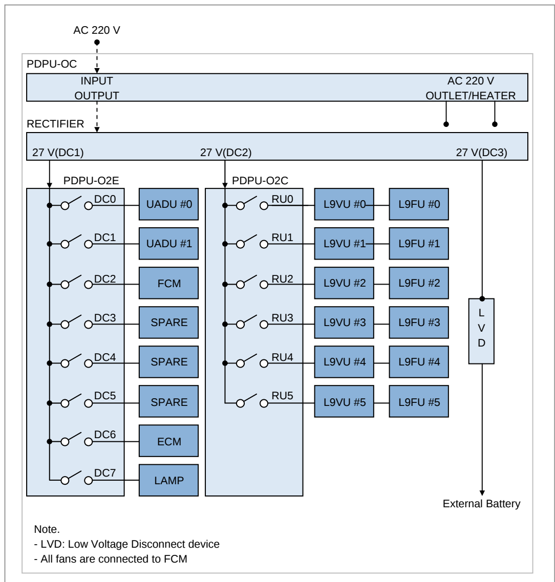
Figure 3.10 Power Structure
