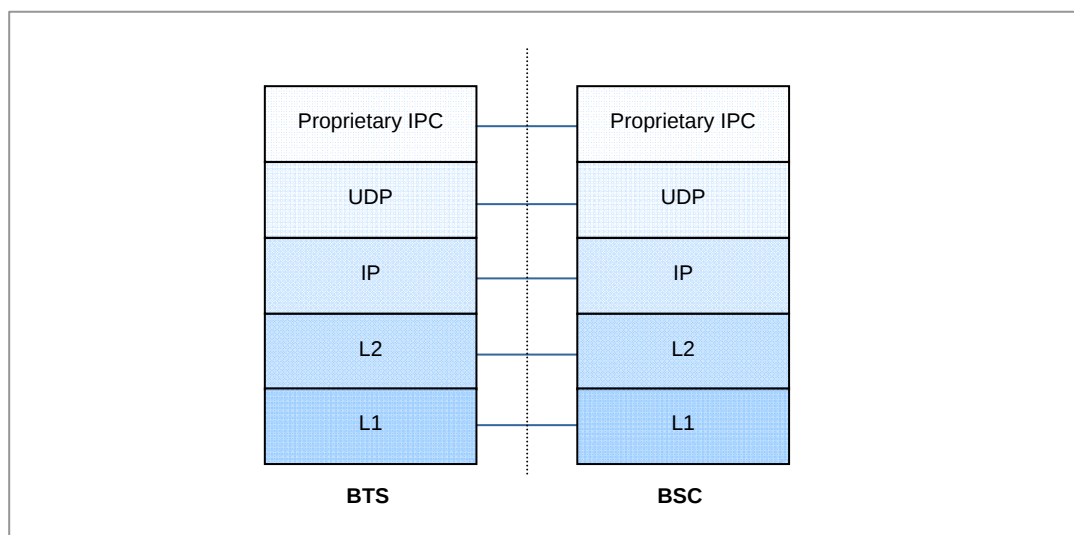
Figure 2.2 Protocol Stack between BTS and BSC
