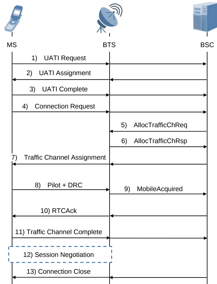
Figure 4.8 1xEV-DO Session setup
