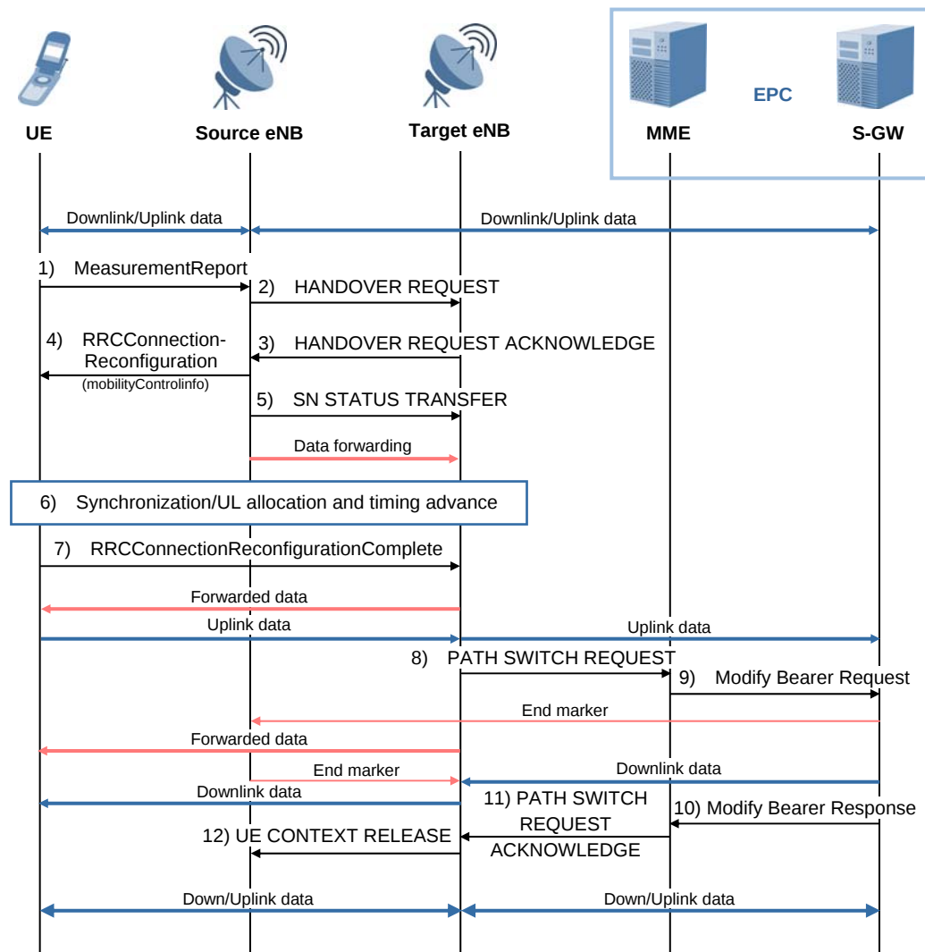
Figure 4.20 X2-based Handover Procedure
