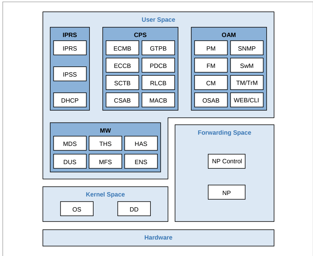
Figure 3.18 LTE Software Structure
