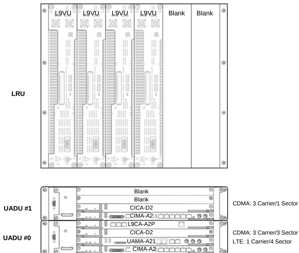
Figure 3.3 CDMA/LTE 4 Sector Configuration
