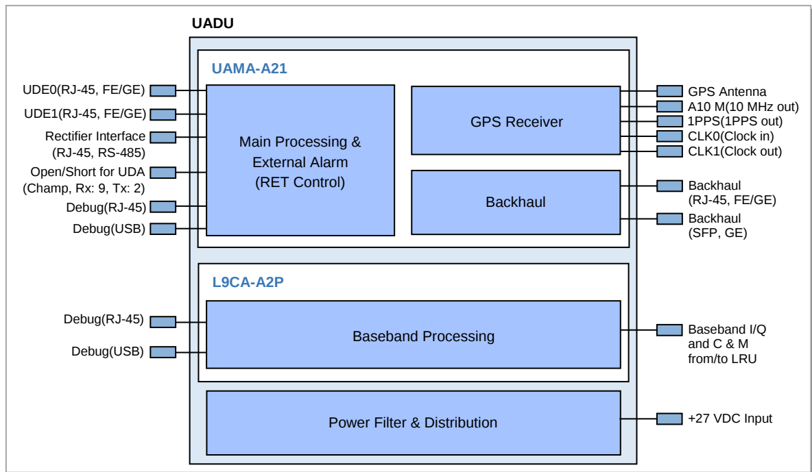
Figure 3.12 Hardware Interface structure of UADU (LTE)
