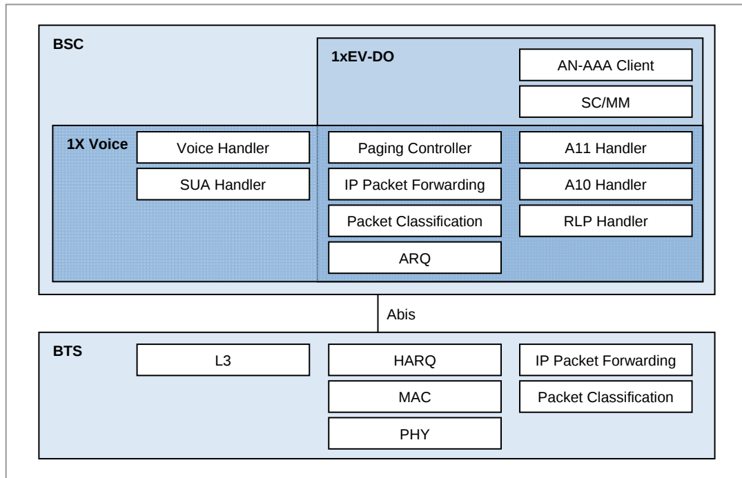
Figure 1.4 CDMA System Functional Structure
