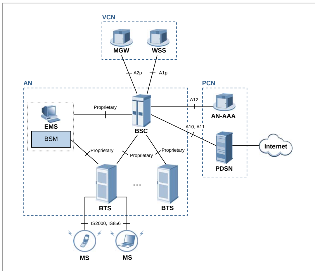
Figure 1.2 CDMA System Network Configuration
