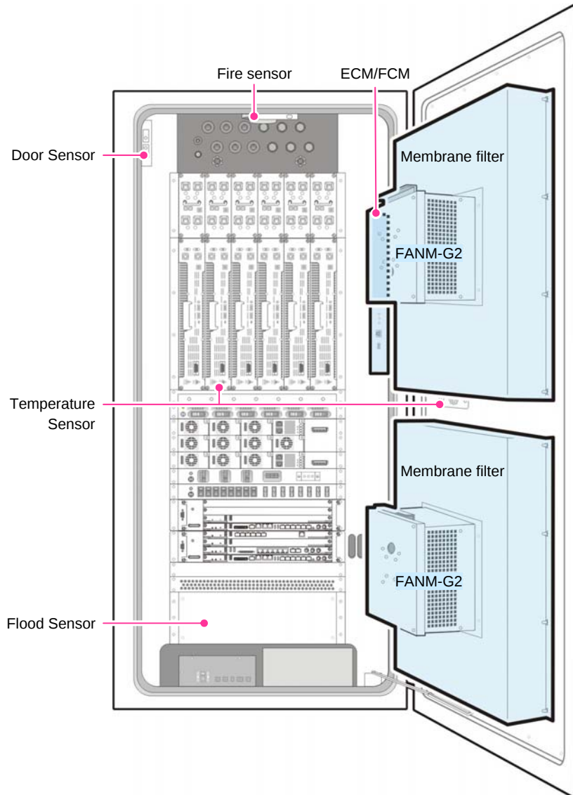
Figure 3.10 Configuration of Environment Devices
