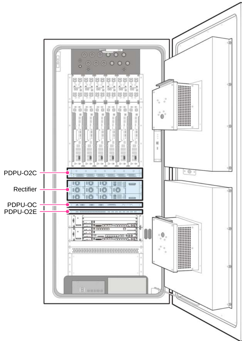
Figure 3.9 Power Device Configuration
