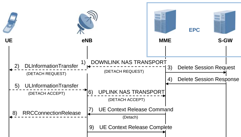
Figure 4.19 Detach Process by MME
