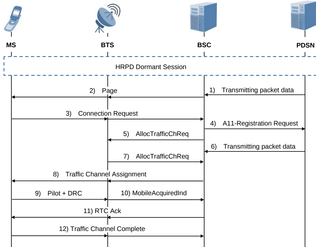
Figure 4.12 Transition from 1xEV-DO Dormant status to the Active state by network
