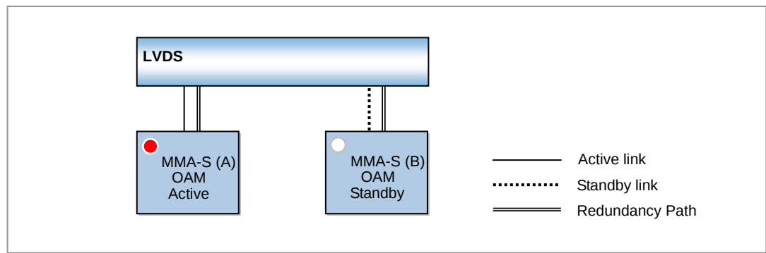
Figure 3.27 Redundancy Structure of OAM Block (MMA-S)
