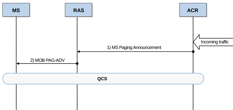
Figure 4.10 Paging Procedure
