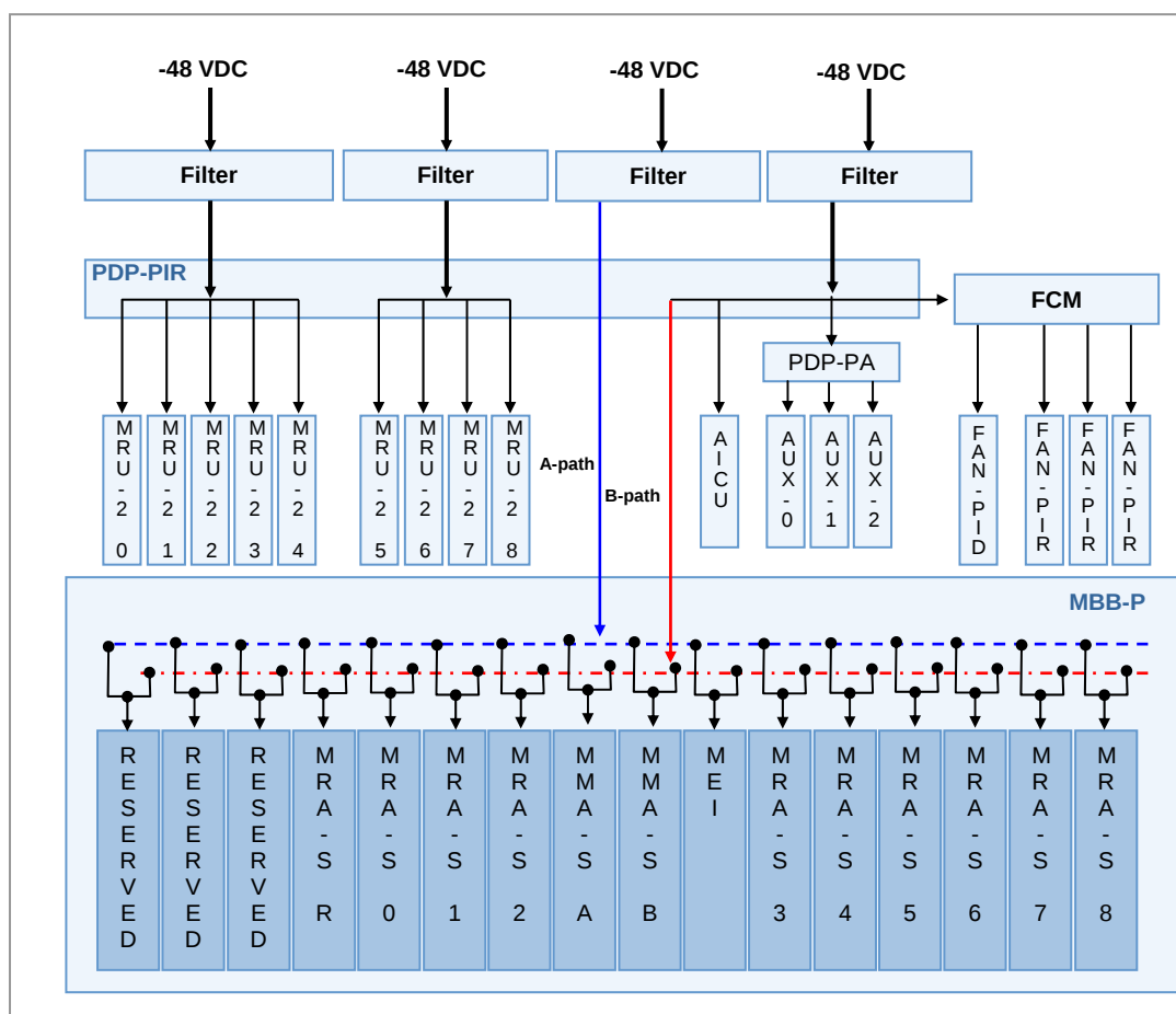
Figure 3.5 Power Structure
