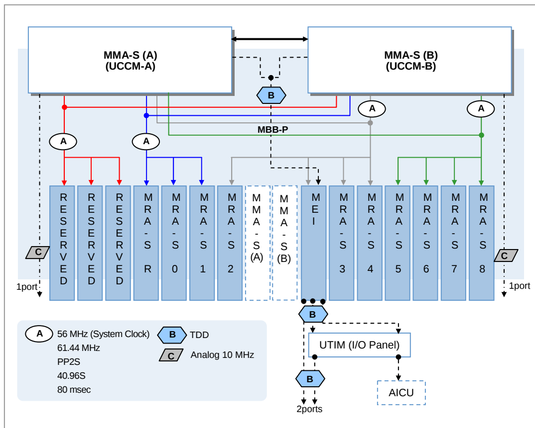
Figure 4.16 Network Synchronization Flow of Indoor SPI-2210
