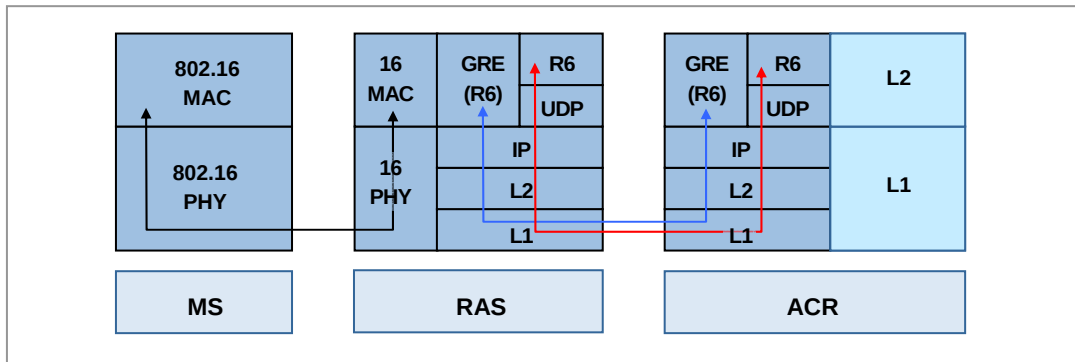
Figure 2.5 Protocol Stack between NEs
