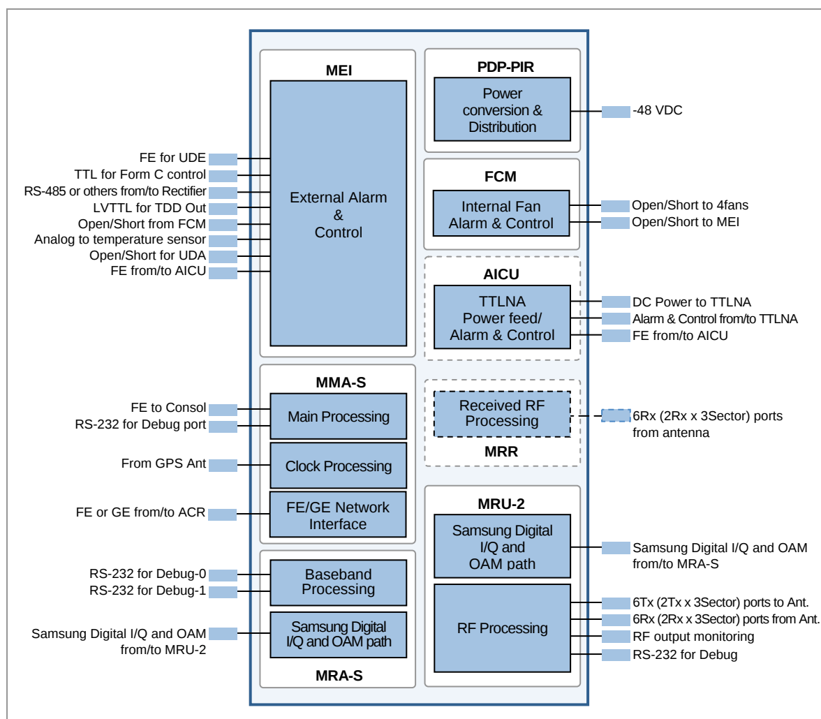
Figure 3.9 External Interfaces of Indoor SPI-2210
