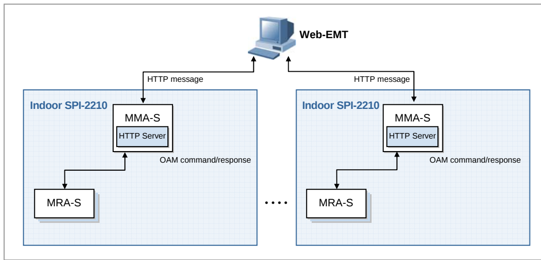
Figure 5.2 Web-EMT Interface
