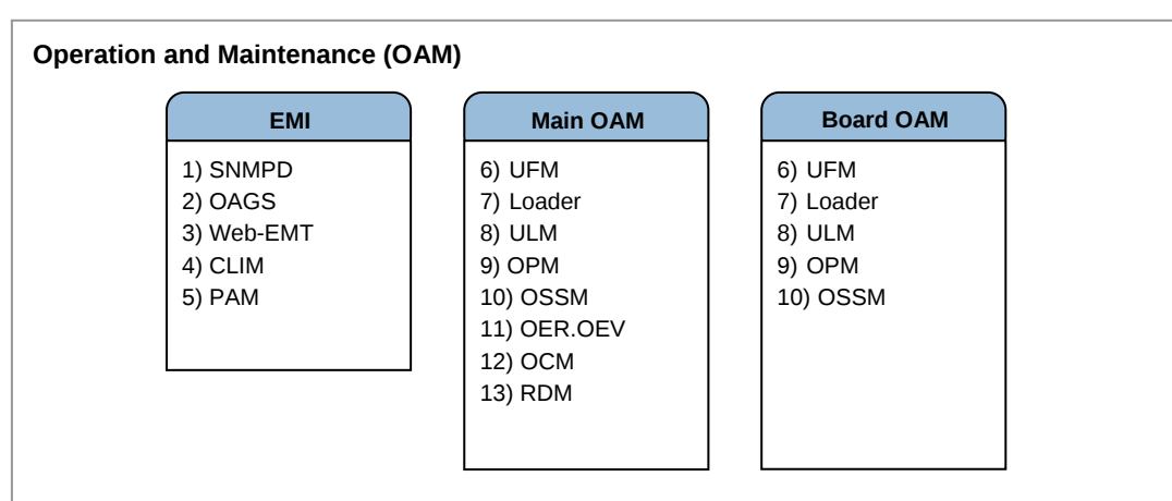
Figure 3.12 OAM Software Structure
