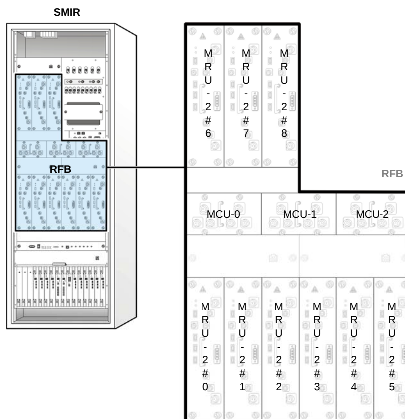
Figure 3.3 RFB Configuration
