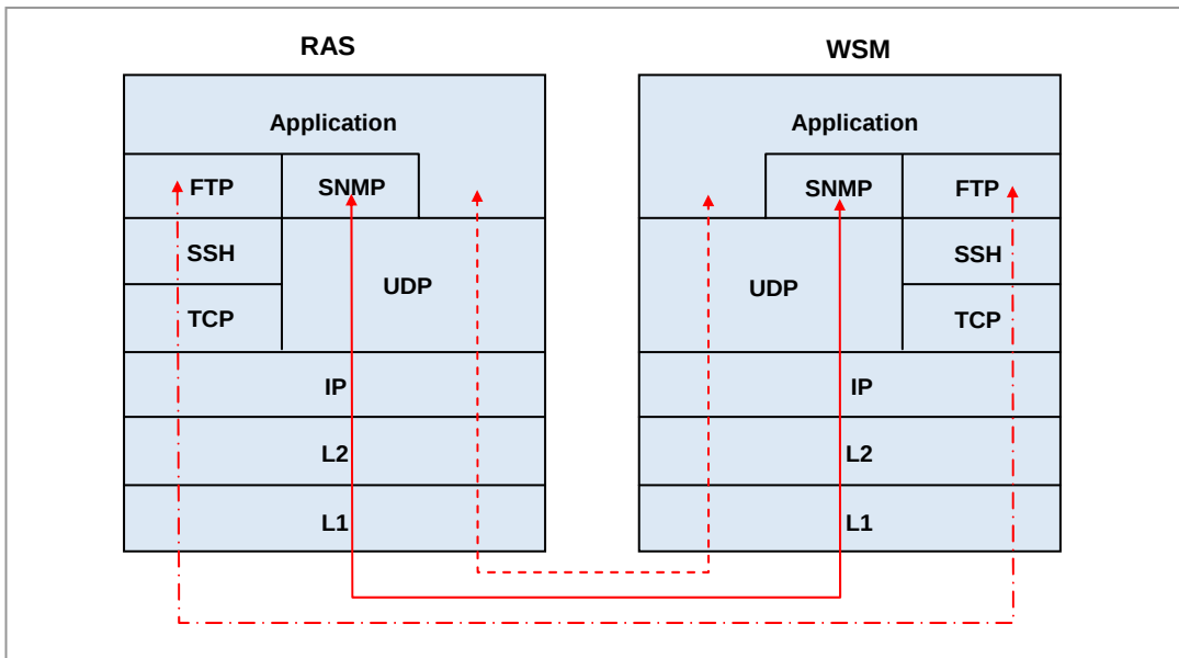
Figure 2.6 Protocol Stack between Indoor SPI-2210 and WSM
