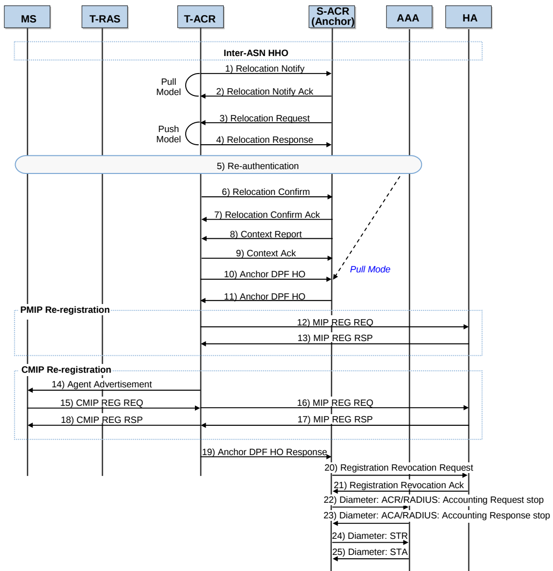
Figure 4.13 Inter-ASN Handover (CSN-Anchored Mobility)
