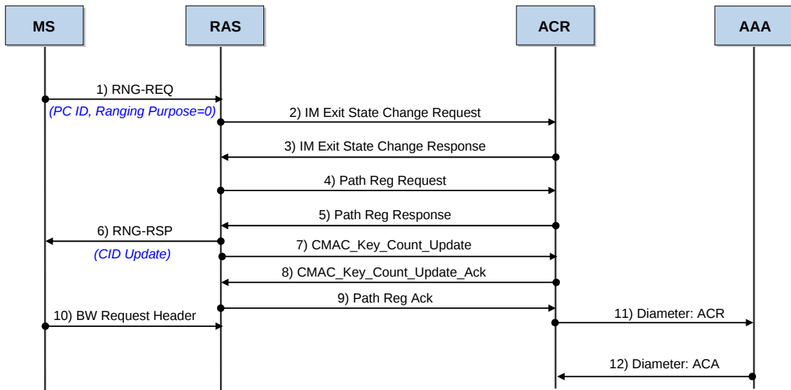
Figure 4.6 Idle Mode → Awake Mode (QCS) Procedure
