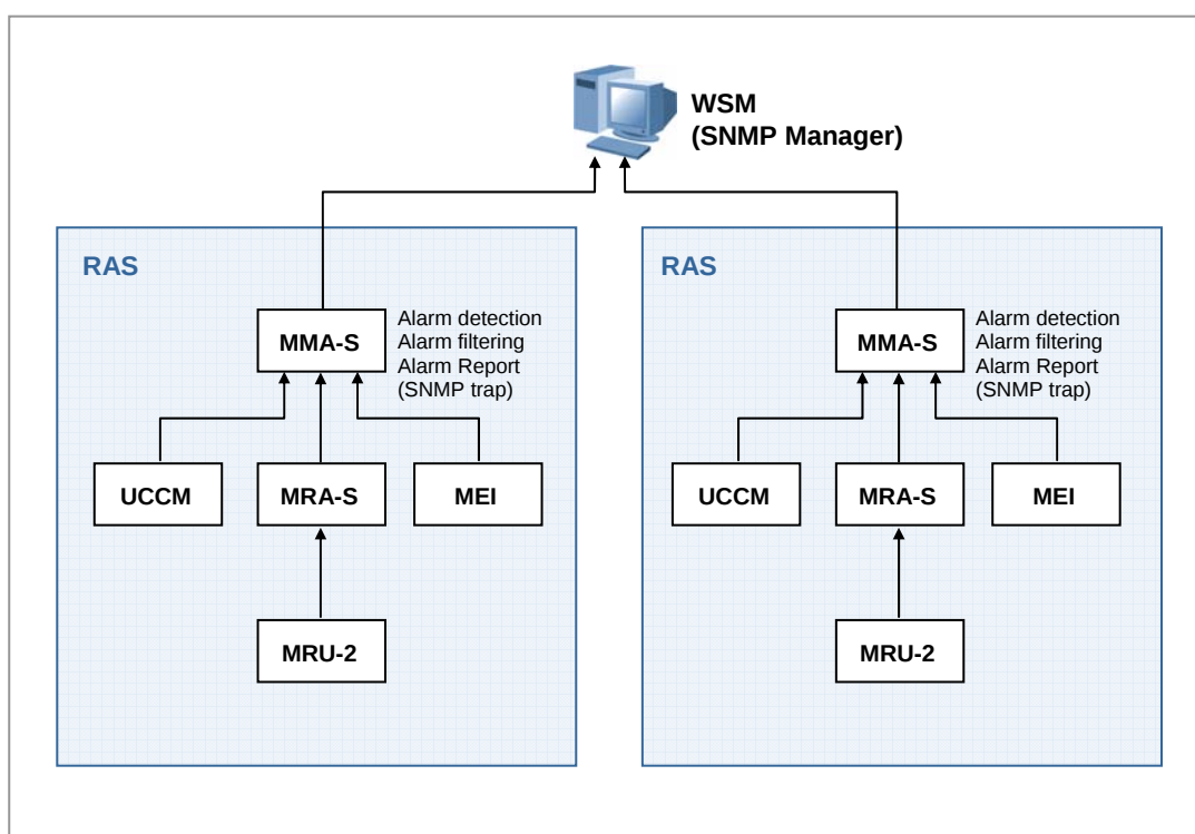
Figure 4.17 Alarm Signal Flow of Indoor SPI-2210
