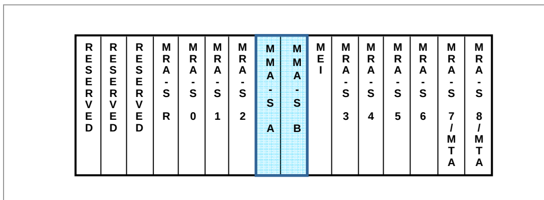
Figure 3.26 RDM Block
