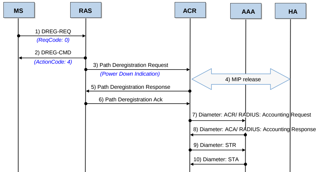
Figure 4.14 Access Termination (Awake Mode)
