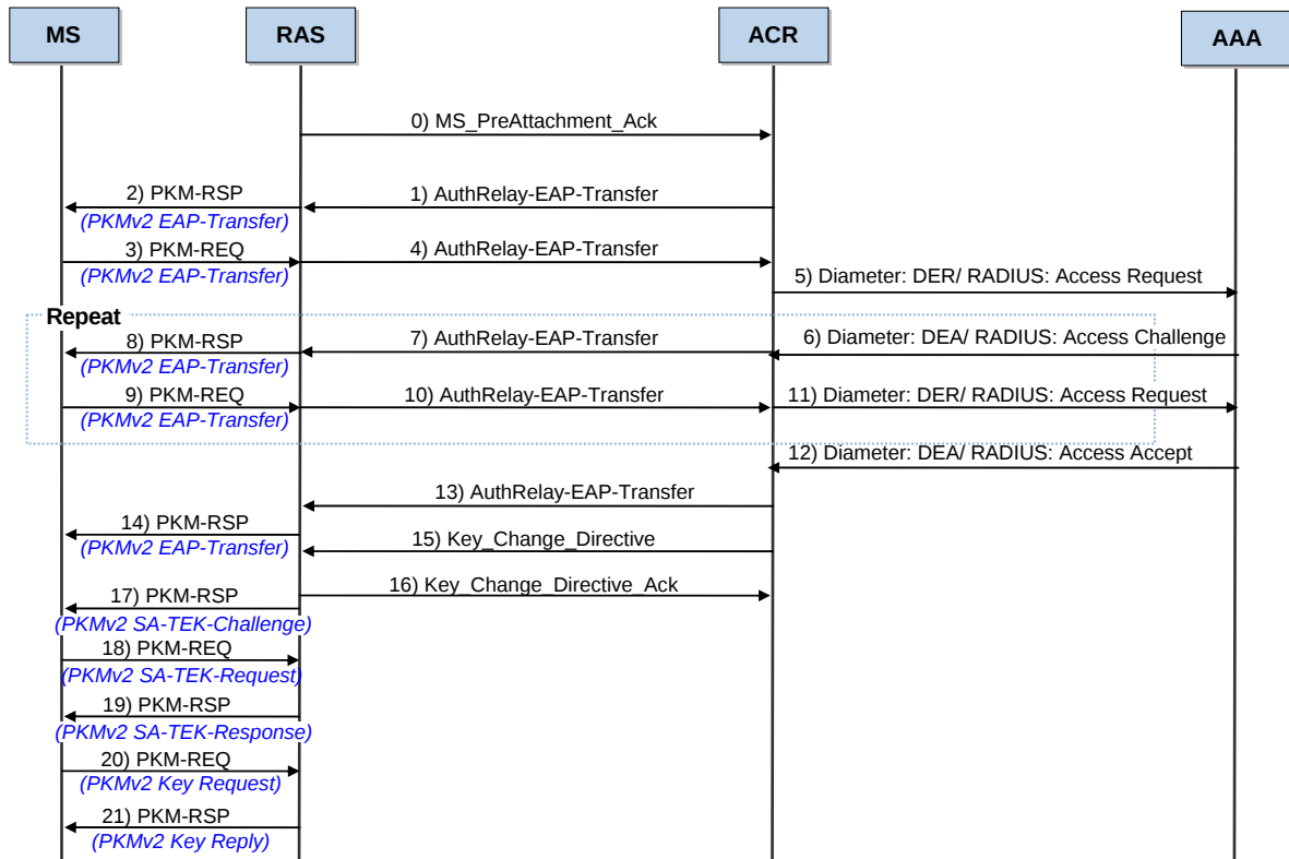
Figure 4.2 Authentication Procedure (At the time of initial access)
