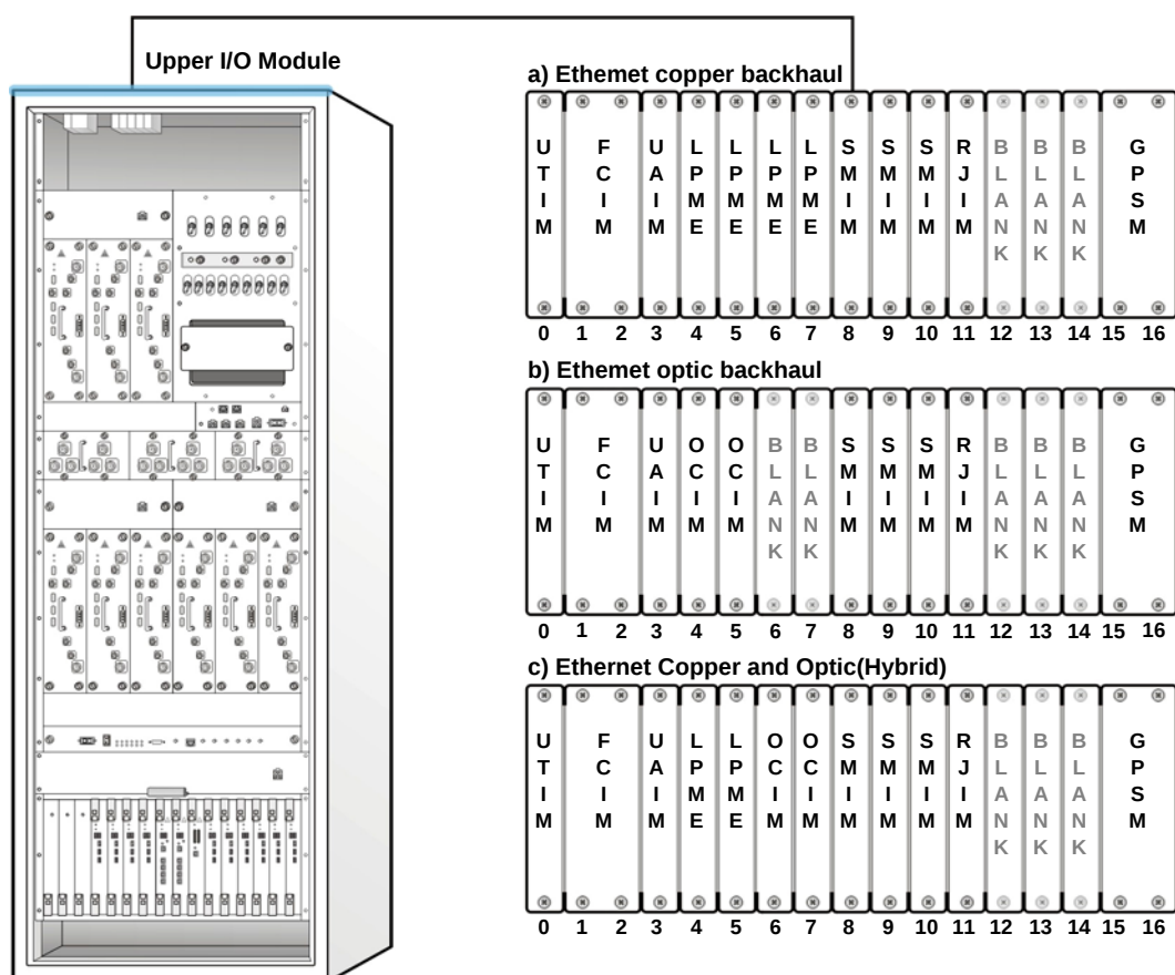
Figure 3.8 I/O Module Configuration
