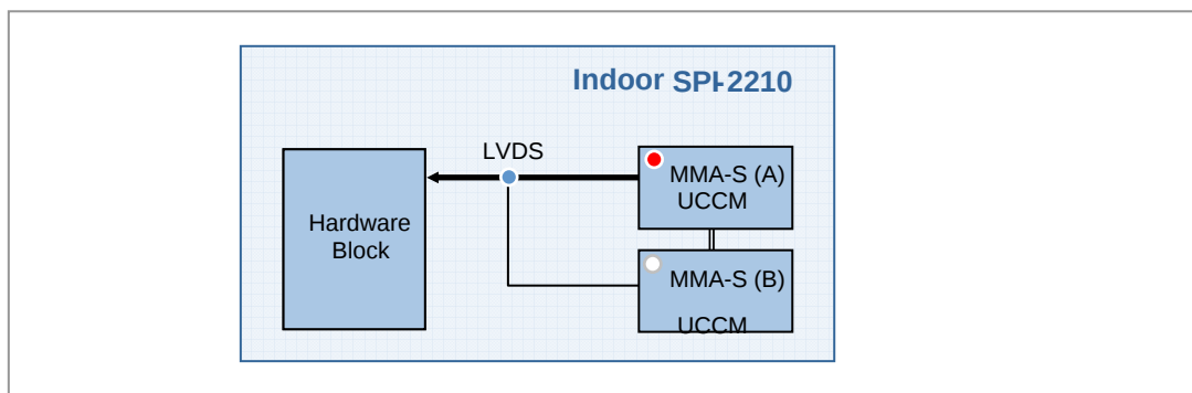
Figure 3.28 Redundancy Structure of UCCM (MMA-S)
