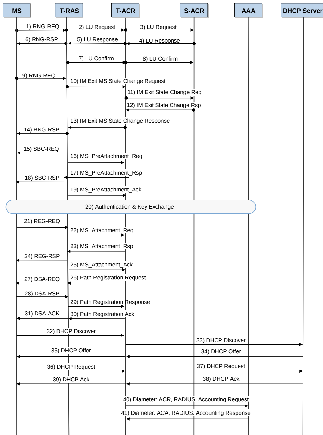
Figure 4.9 Inter-ACR Location Update Procedure (Simple IP Case)
