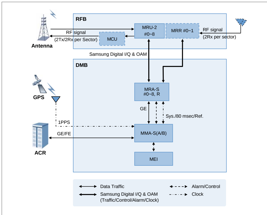
Figure 3.1 Internal Configuration of Indoor SPI-2210
