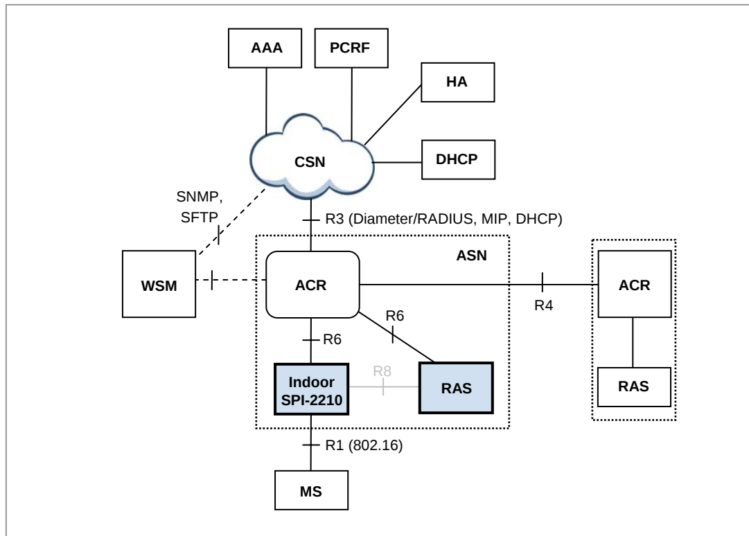
Figure 2.4 Structure of Indoor SPI-2210 Interface
