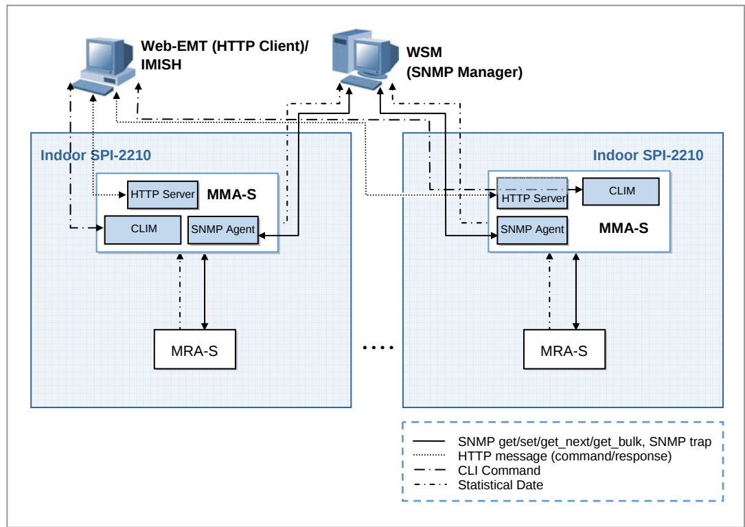
Figure 4.20 Operation and Maintenance Signal Flow
