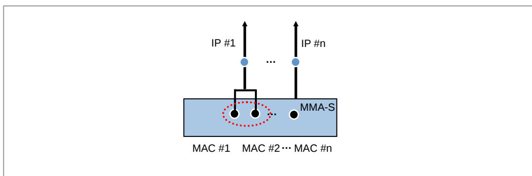
Figure 3.30 Load Sharing Structure of Backhaul
