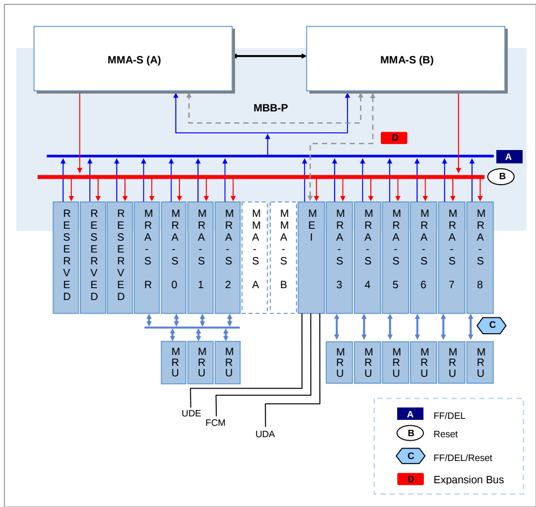
Figure 4.18 Alarm and Control Structure of Indoor SPI-2210
