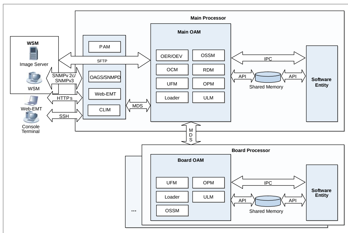
Figure 3.13 Interface between OAM Blocks
