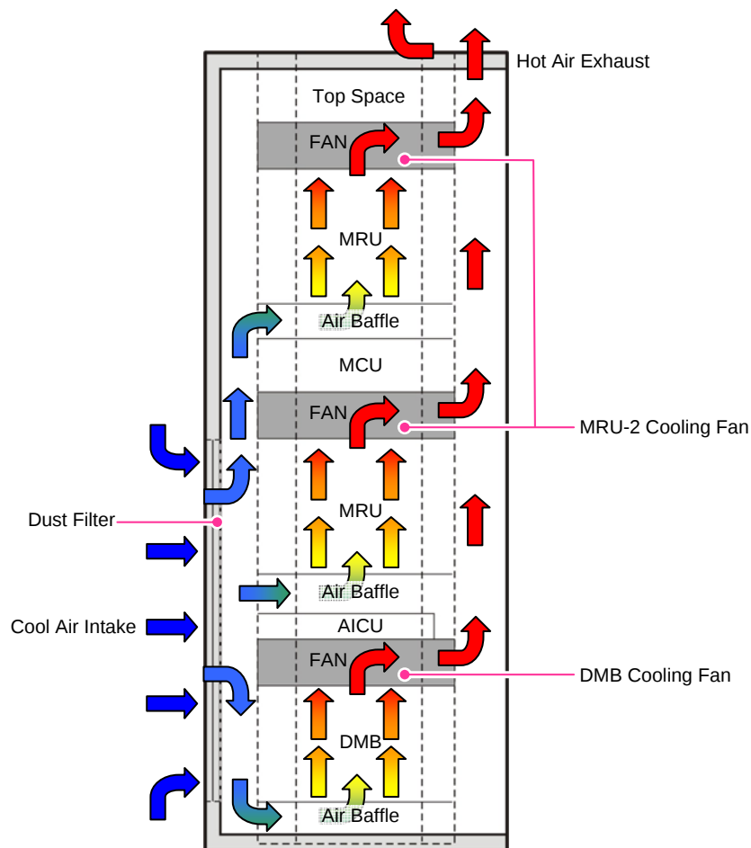
Figure 3.7 Radiation Structure of Indoor SPI-2210
