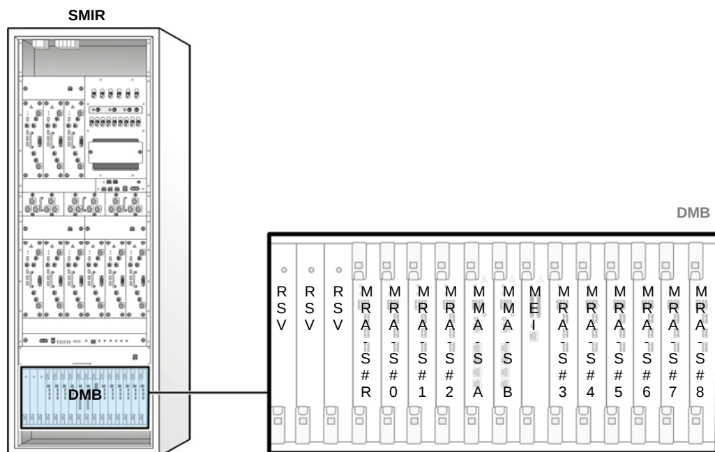
Figure 3.2 DMB Configuration
