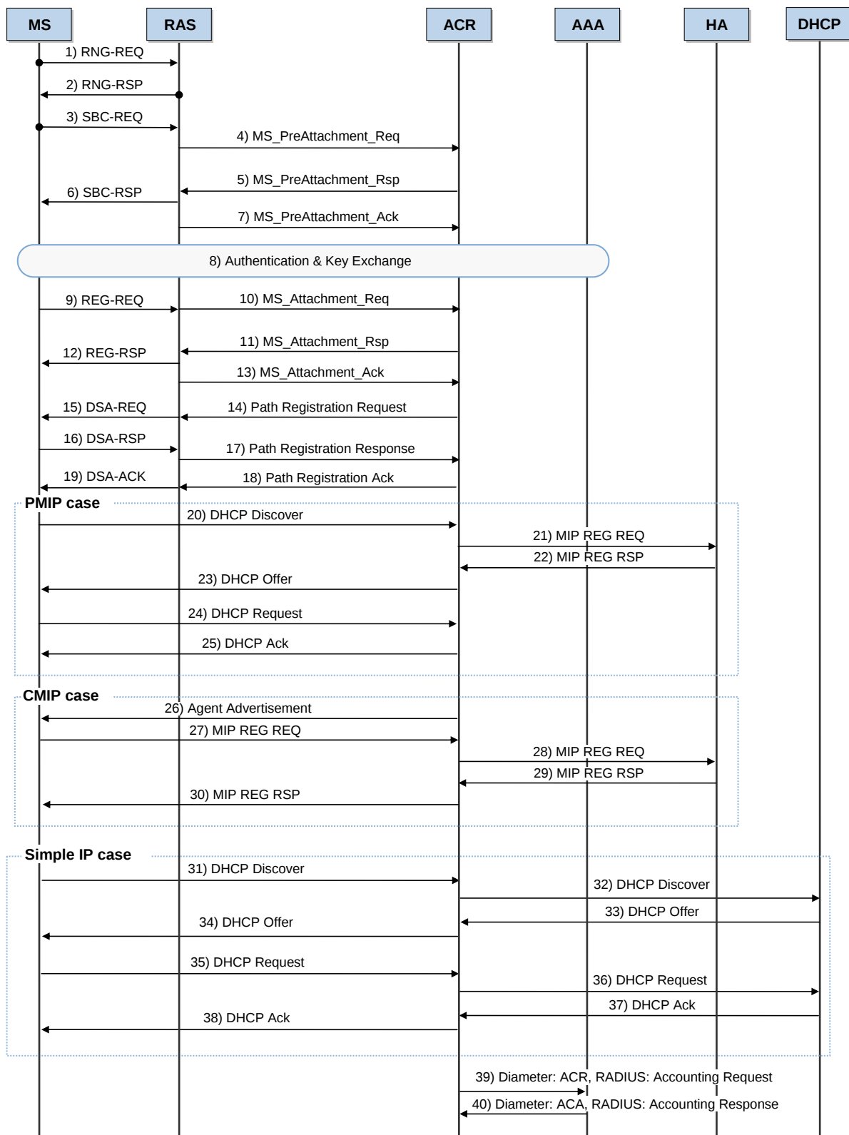
Figure 4.1 Initial Access Process
