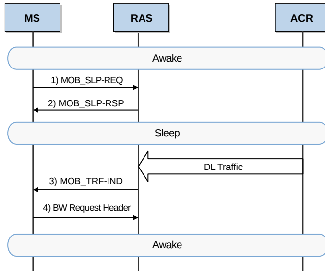
Figure 4.5 Awake Mode ↔ Sleep Mode Status Change Procedure
