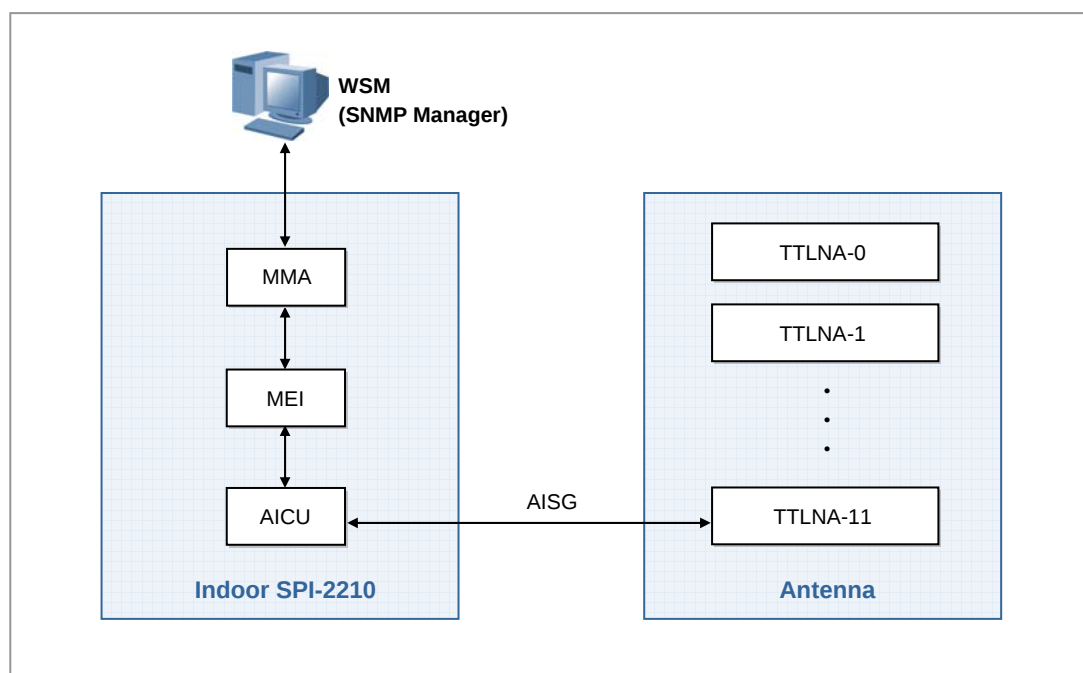
Figure 5.1 TTLNA/RET Interface
