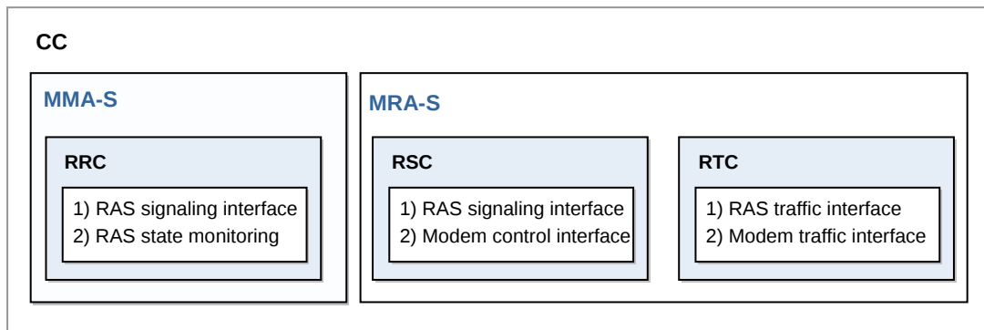
Figure 3.11 CC Block Structure
