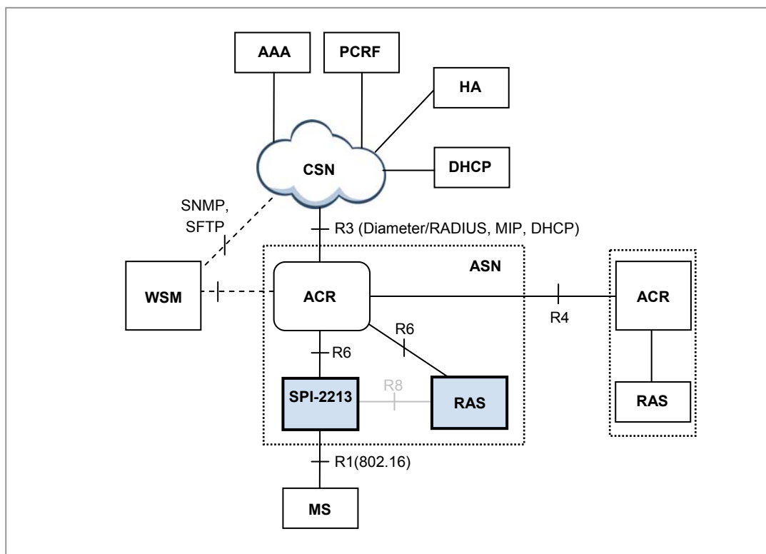
Figure 2.5 Structure of SPI-2213 Interface
