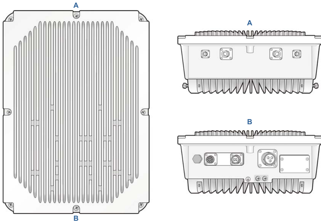
Figure 2.3 RRH Configuration
