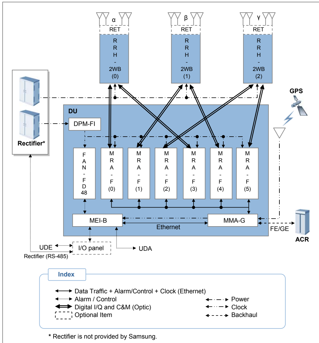
Figure 3.2 Internal Configuration of the System (4T4R with CDD)
