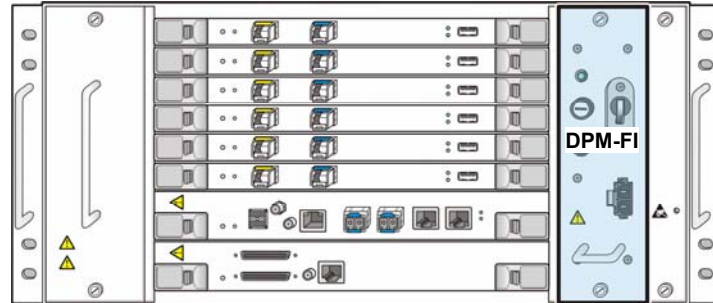
Figure 3.6 DPM-FI Configuration
