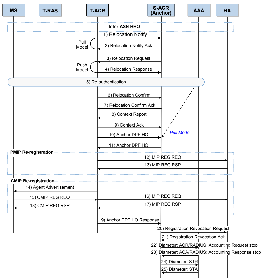
Figure 4.13 Inter-ASN Handover (CSN-Anchored Mobility)
