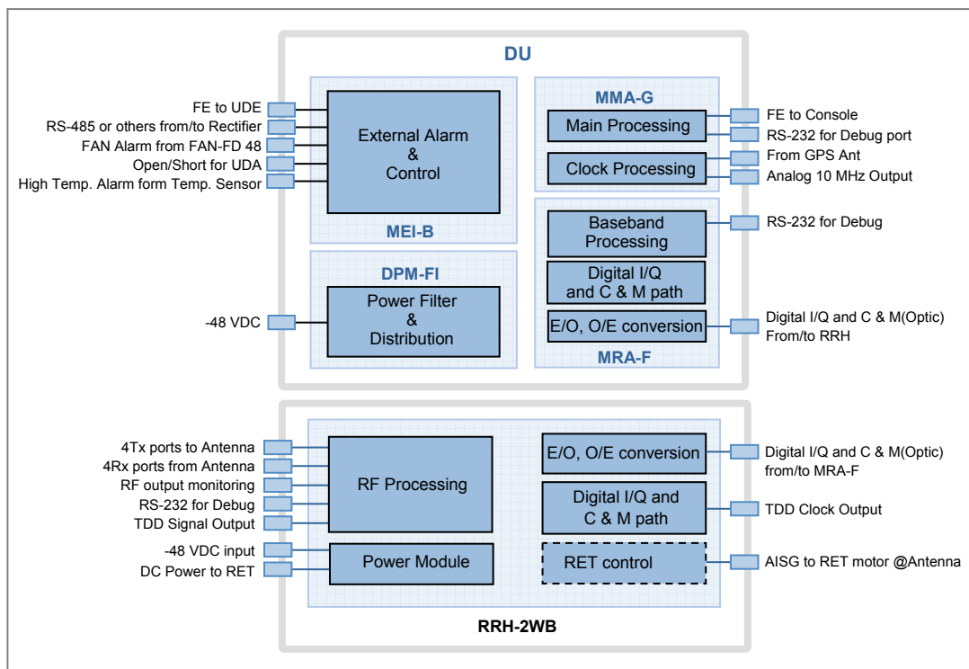
Figure 3.11 Interfaces of SPI-2213 (4T4R with CDD)
