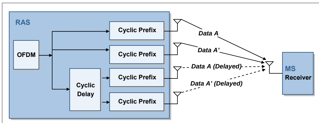
Figure 1.4 4T4R with CDD (Matrix A + CDD mode)
