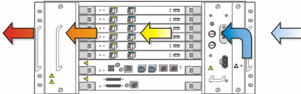
Figure 3.9 Cooling Structure of the DU
