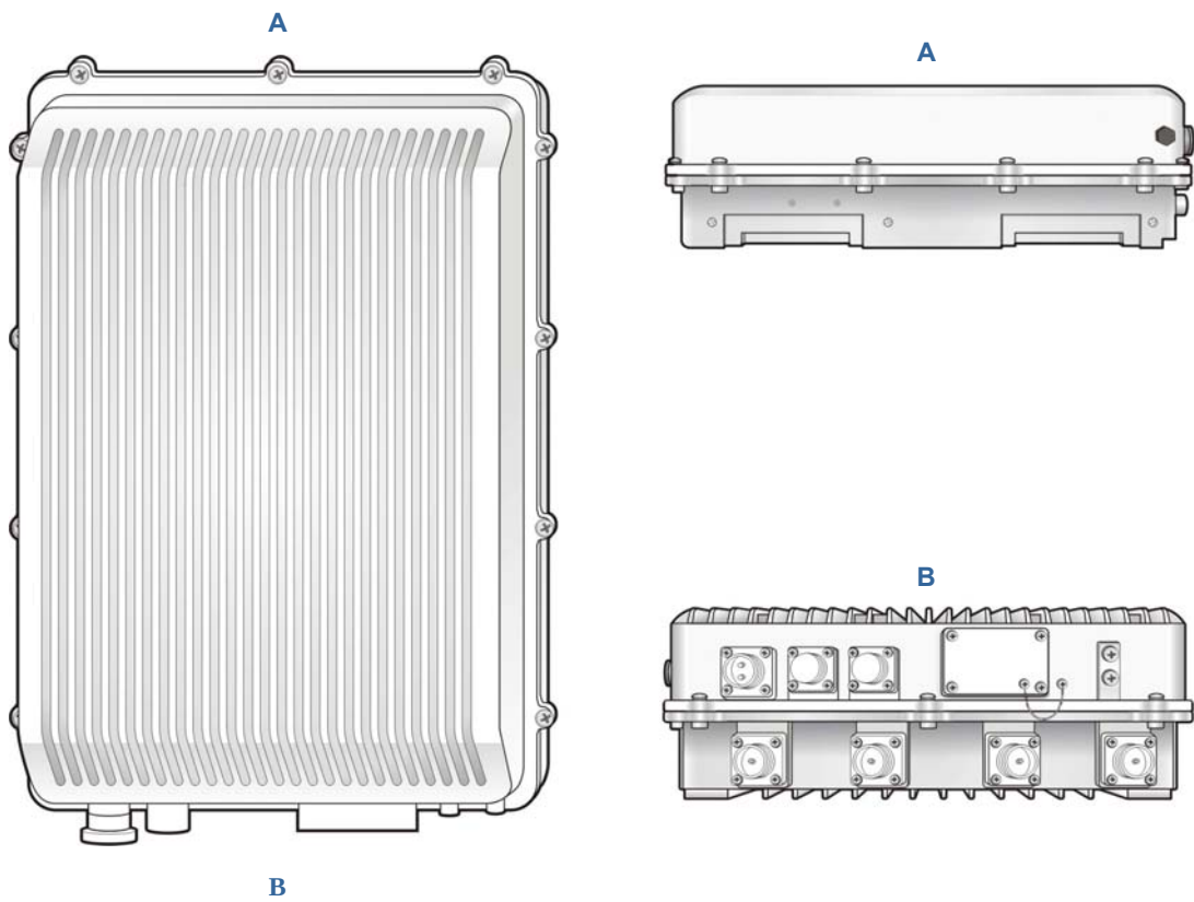
Figure 2.4 RRH-2WB Configuration
