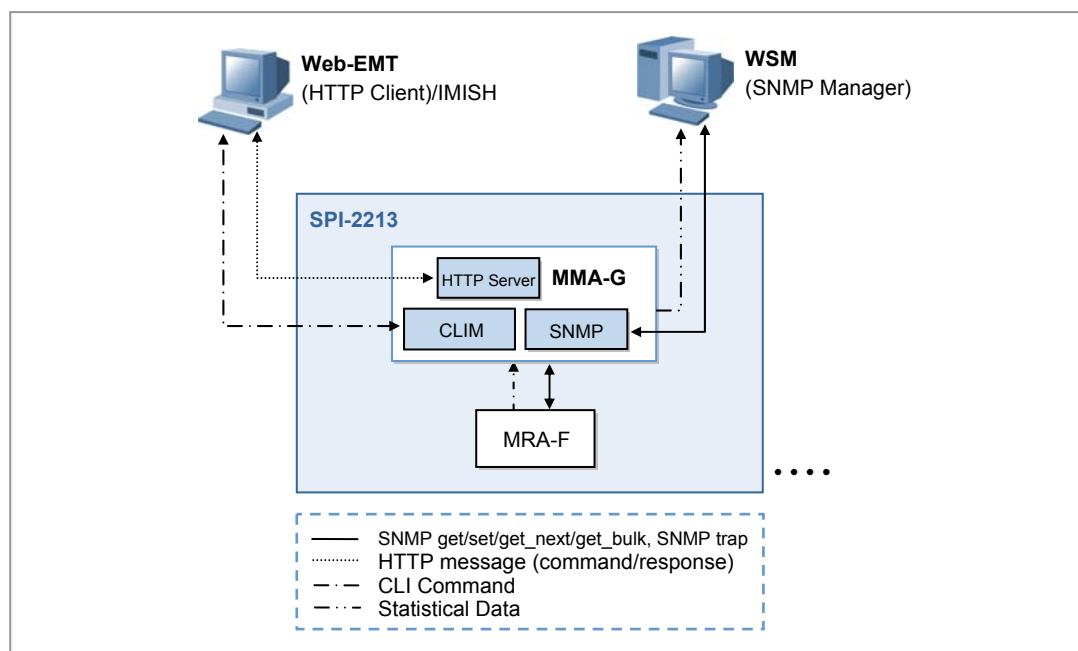
Figure 4.20 Operation and Maintenance Signal Flow
