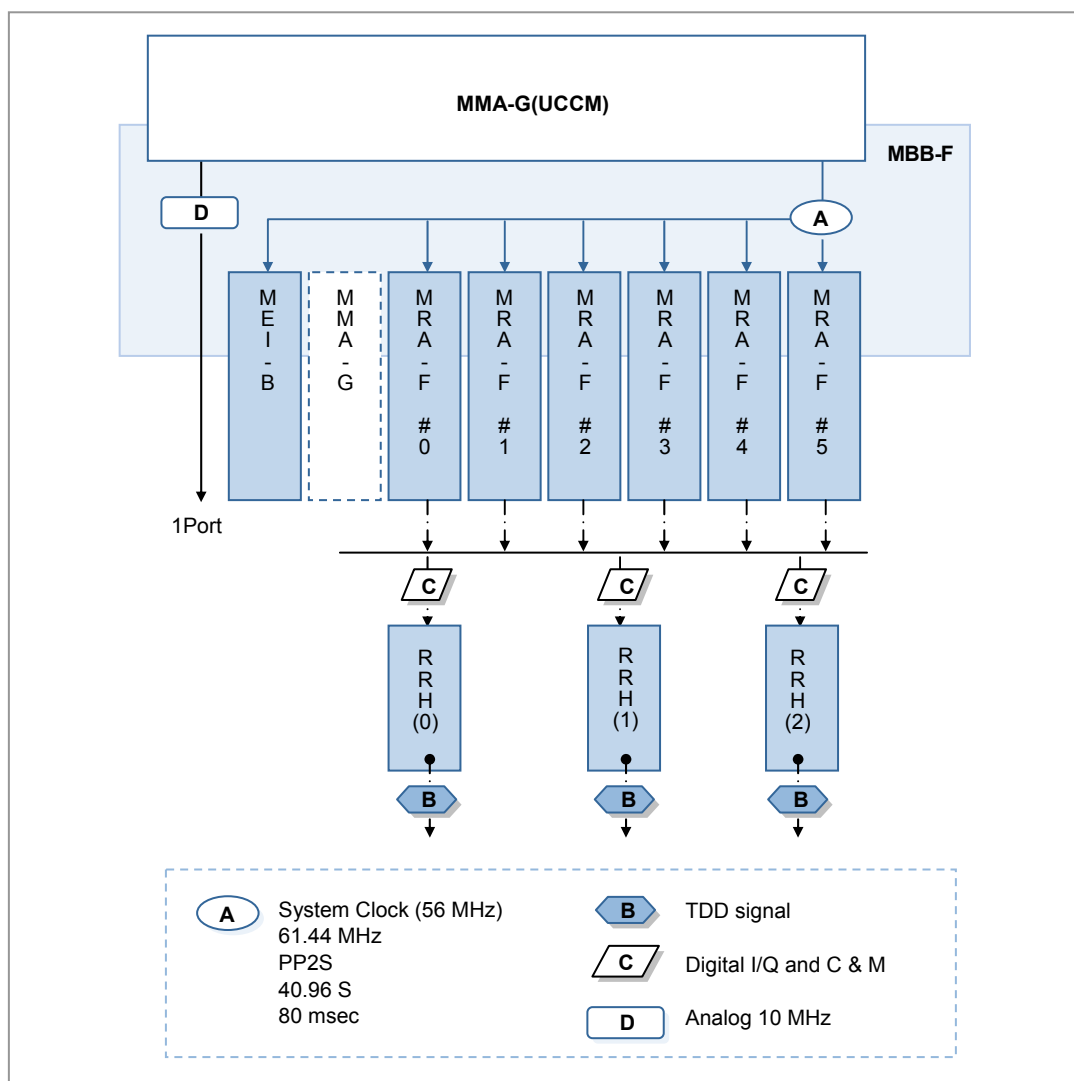
Figure 4.16 Network Synchronization Flow of SPI-2213
