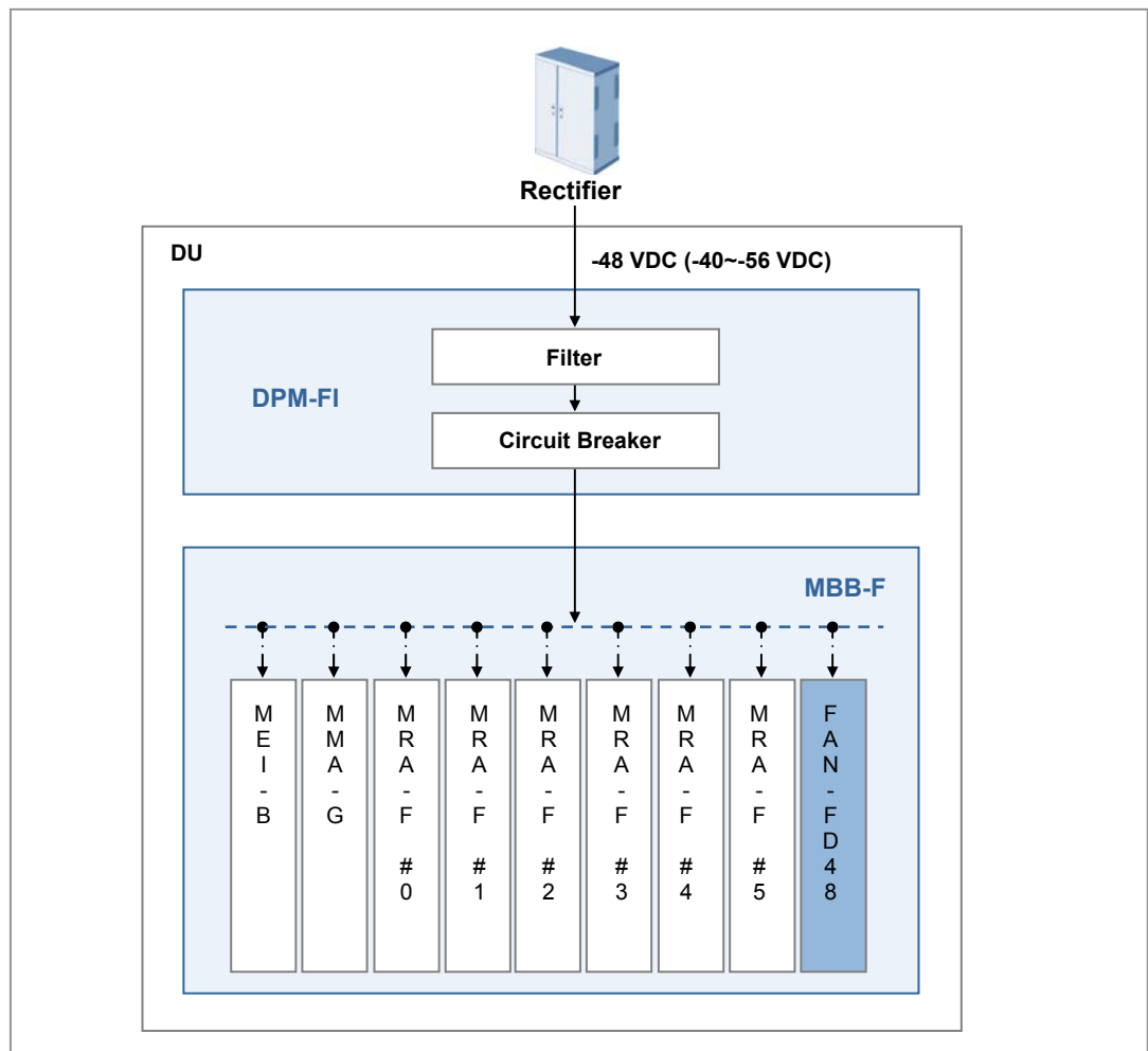
Figure 3.7 Power Structure of SPI-2213
