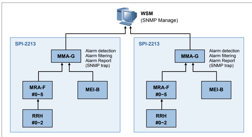
Figure 4.17 Alarm Signal Flow of SPI-2213
