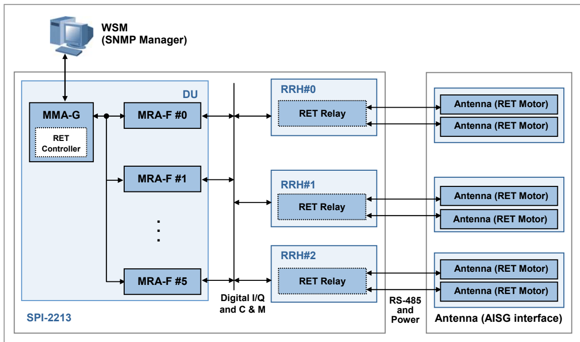
Figure 5.1 RET Interface
