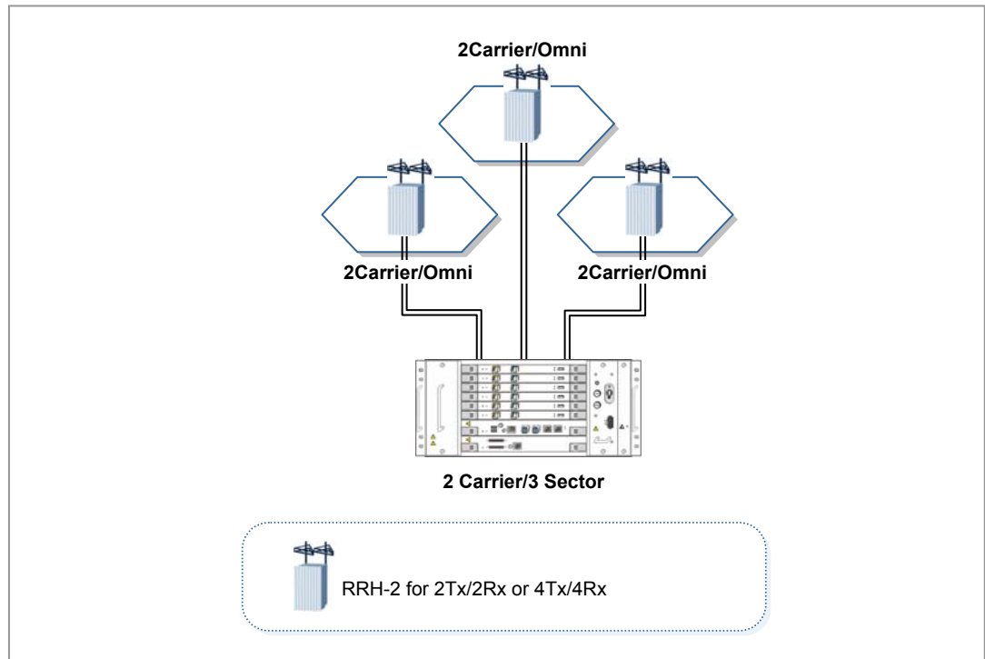
Figure 3.5 Omni Configuration Example Using RRH-2
