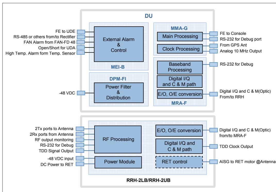
Figure 3.10 Interfaces of SPI-2213 (MIMO)
