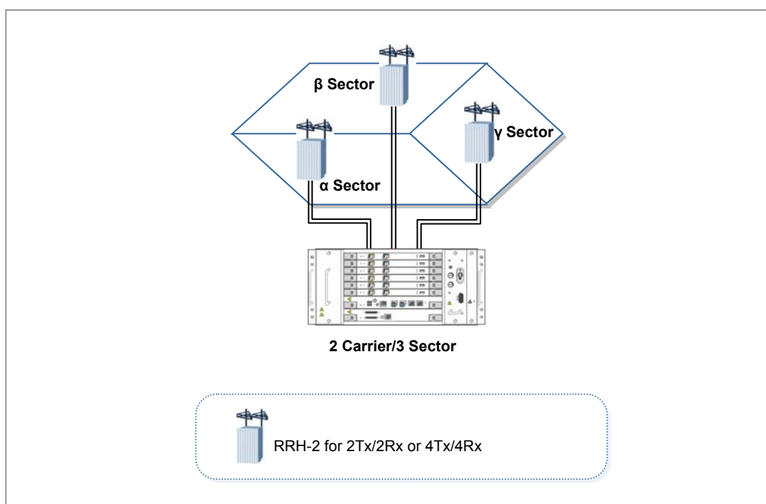
Figure 3.4 Sector Configuration Example Using RRH-2
