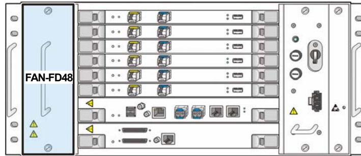
Figure 3.8 Fan Configuration
