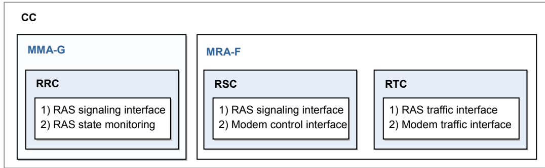
Figure 3.13 CC Block Structure
