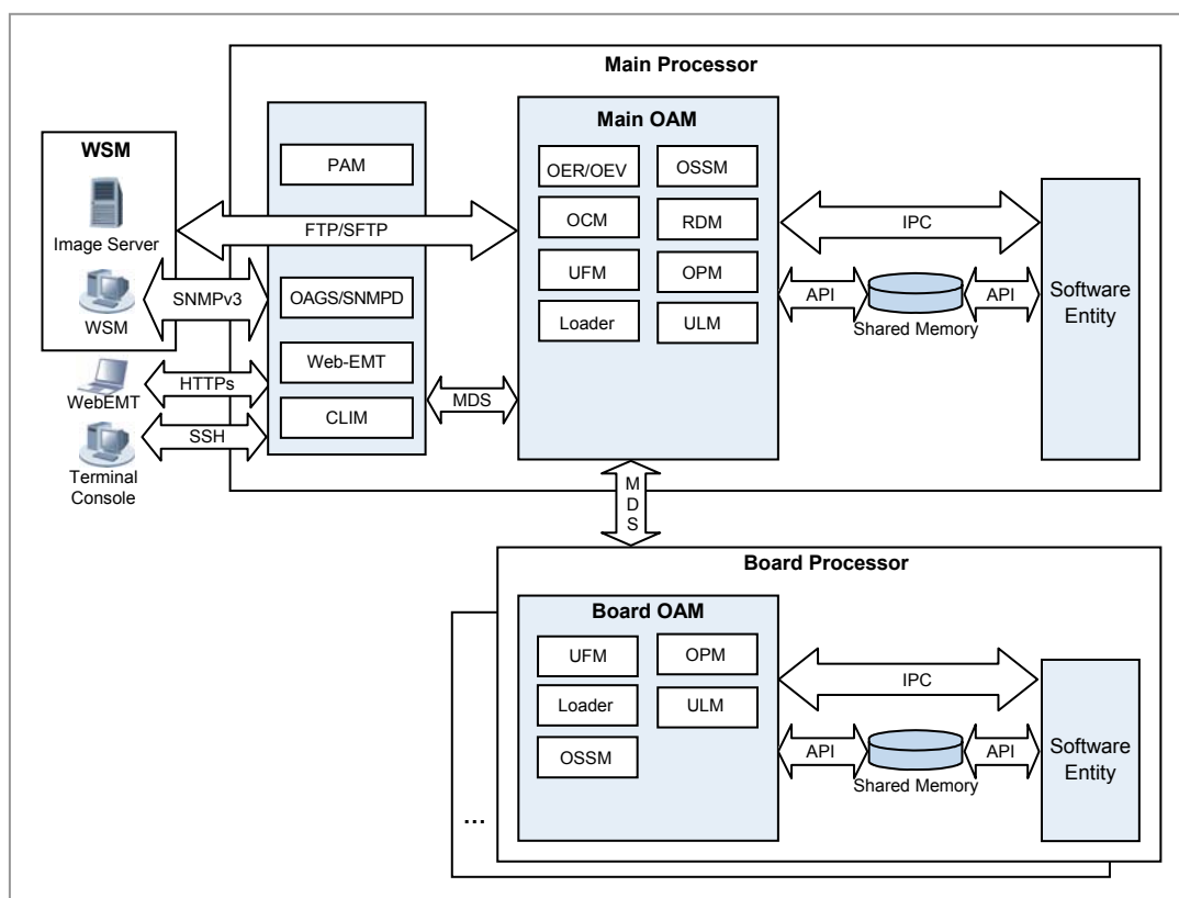
Figure 3.15 Interface between OAM Blocks
