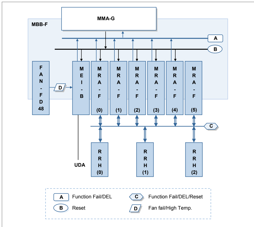
Figure 4.18 Alarm and Control Structure of SPI-2213
