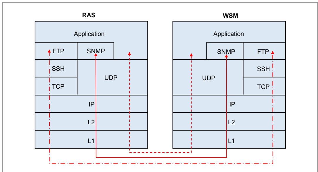
Figure 2.7 Protocol Stack between SPI-2213 and WSM
