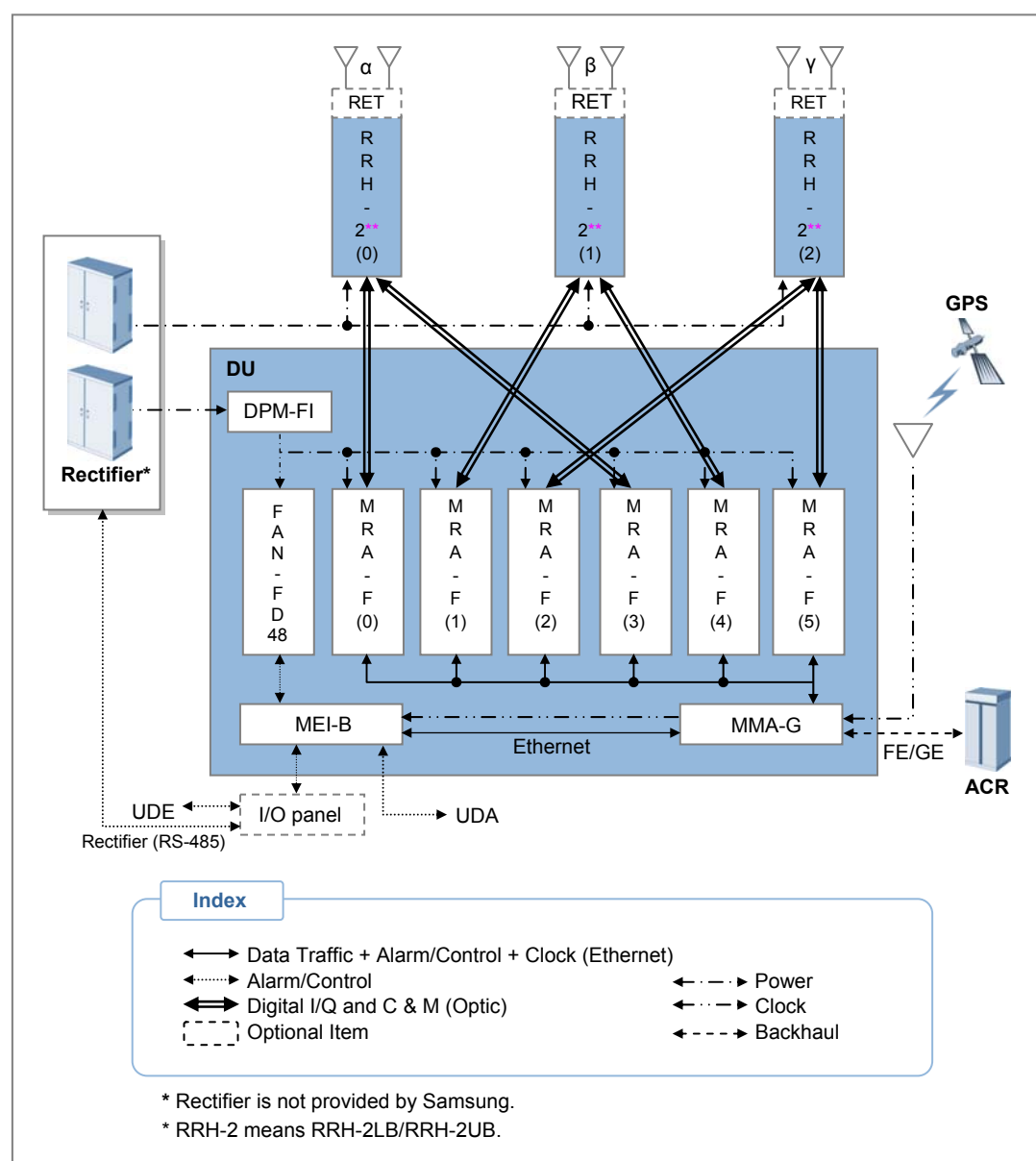
Figure 3.1 Internal Configuration of the System (MIMO)
