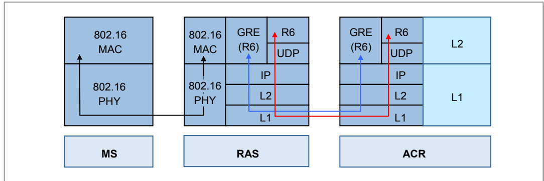
Figure 2.6 Protocol Stack between NEs
