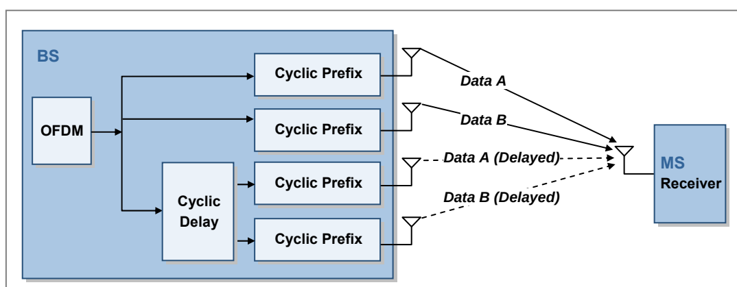
Figure 1.5 4T4R with CDD (Matrix B + CDD mode)
