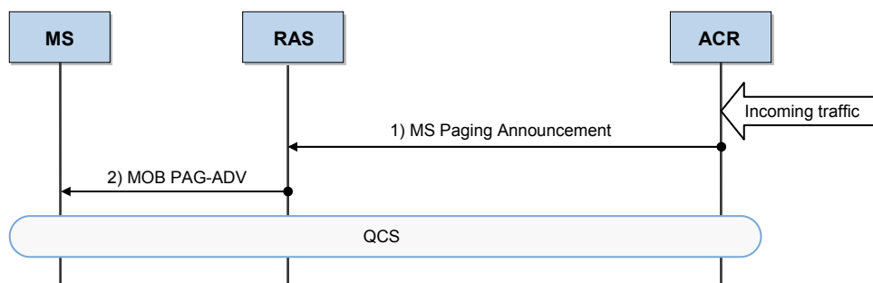
Figure 4.10 Paging Procedure
