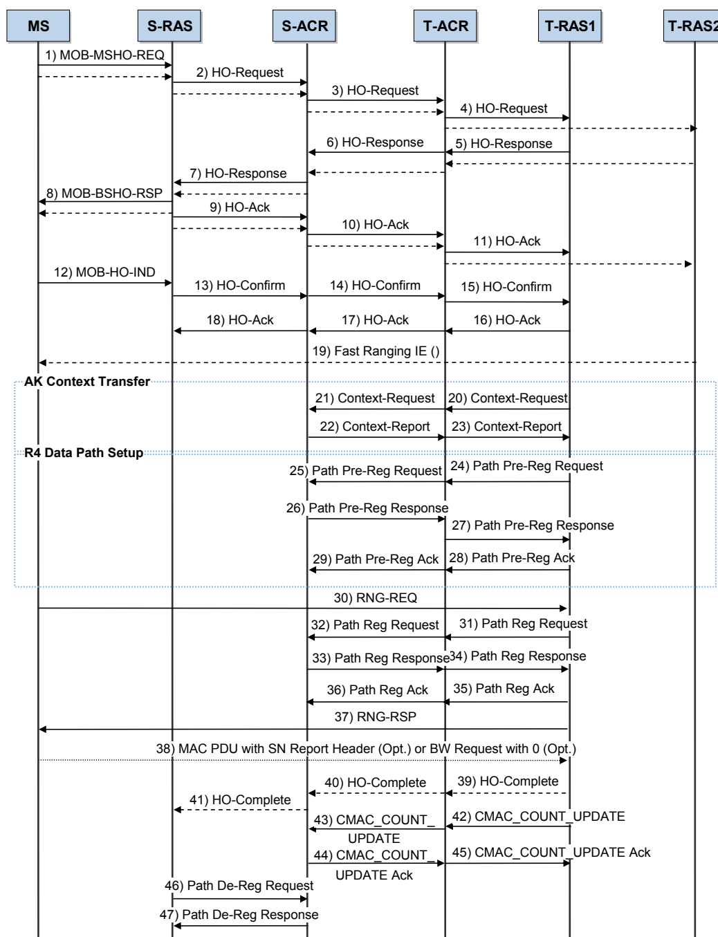
Figure 4.12 Inter-ASN Handover (ASN-Anchored Mobility)
