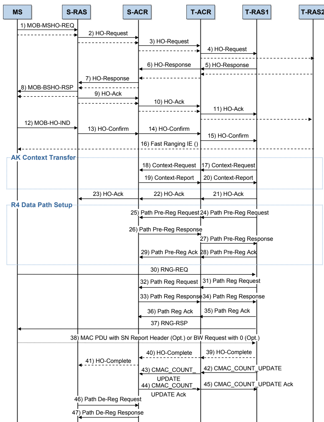
Figure 4.11 Inter-ASN Handover (ASN-Anchored Mobility)
