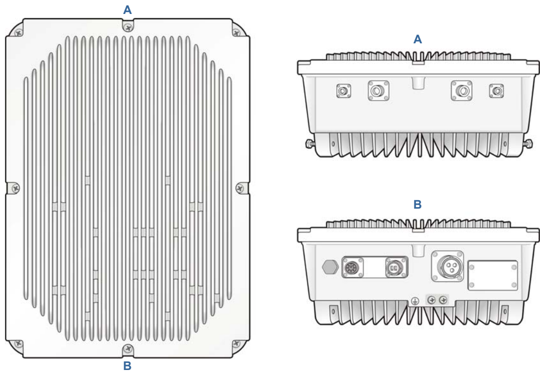
Figure 2.3 RRH Configuration
