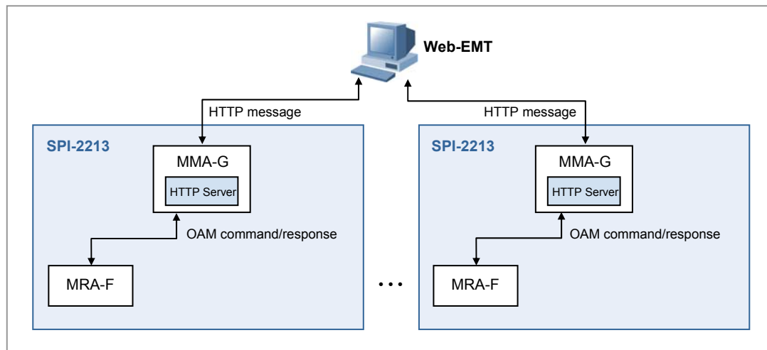
Figure 5.2 Web-EMT Interface
