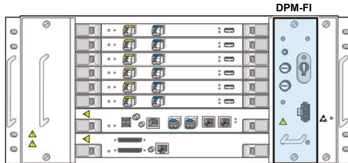
Figure 3.5 DPM-FI Configuration
