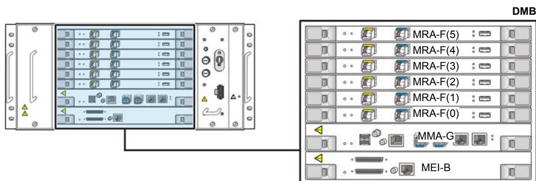
Figure 3.2 DMB Configuration
