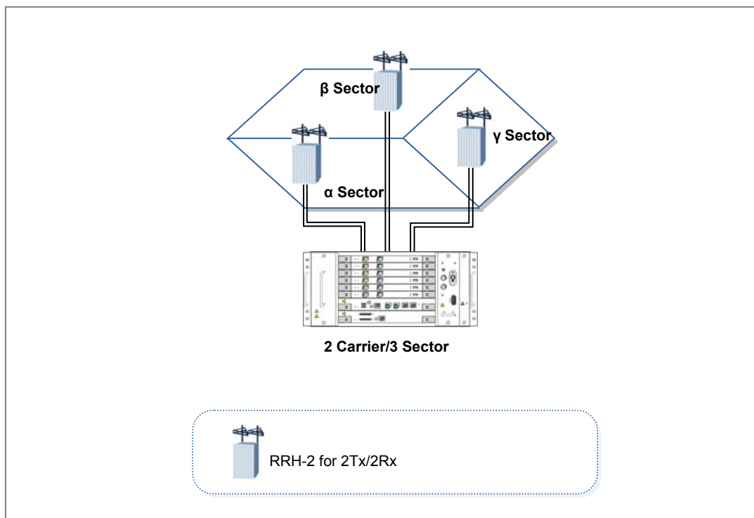
Figure 3.3 Sector Configuration Example Using RRH-2
