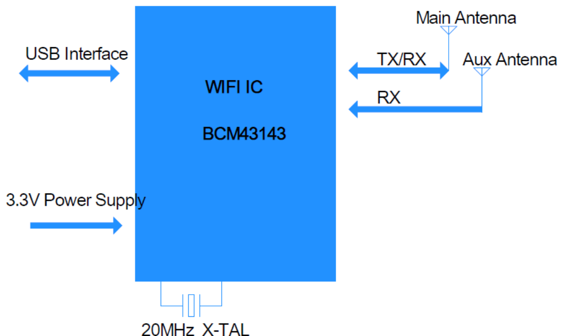
Figure 1-1 SPW-B43143U block diagram and System Interface
