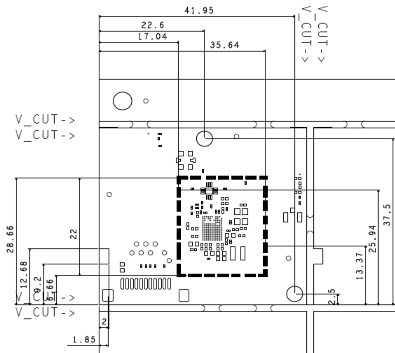
Figure 1-2 SPW-B4319U
