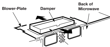
For Front-to-Back Adjustment, Slide the Exhaust Adaptor as Needed
