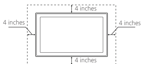
Installation with a wall-mount.
