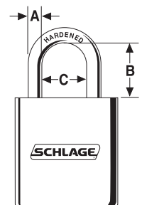
Shackle Dimensions
