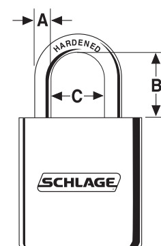
Shackle Dimensions
