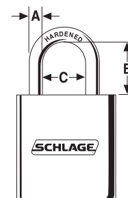
Shackle Dimensions
