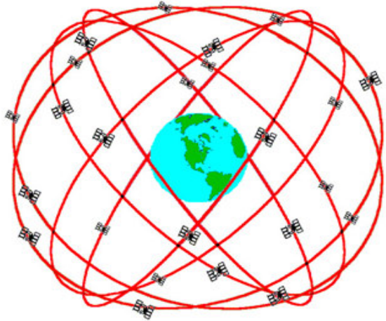
GPS satellite orbital planes
