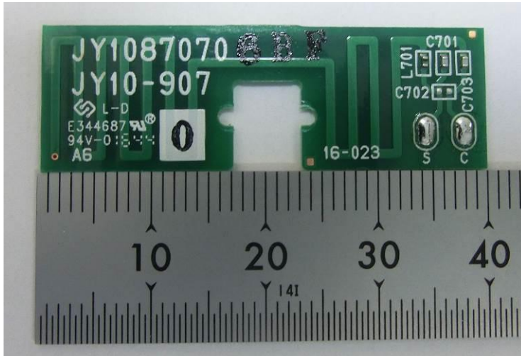
Antenna PCB Bottom View
