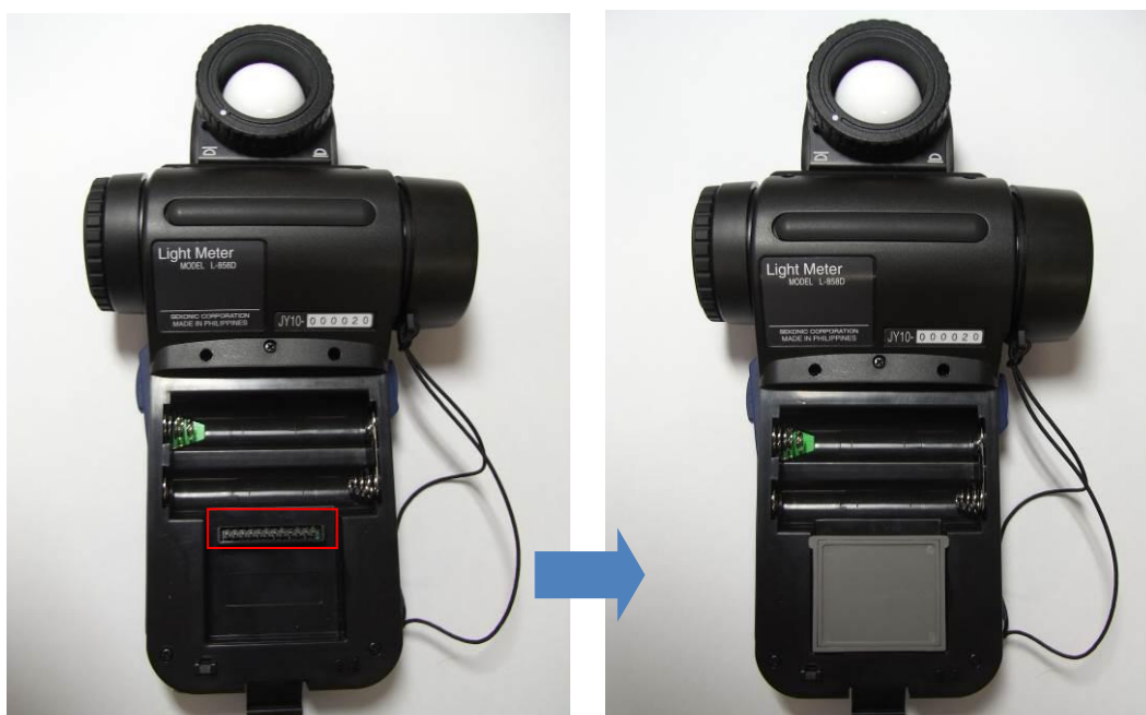
Transmitter module installation
