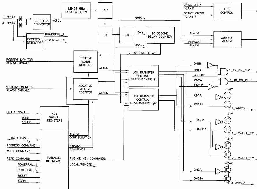
Figure 1-17 LCU Block Diagram
