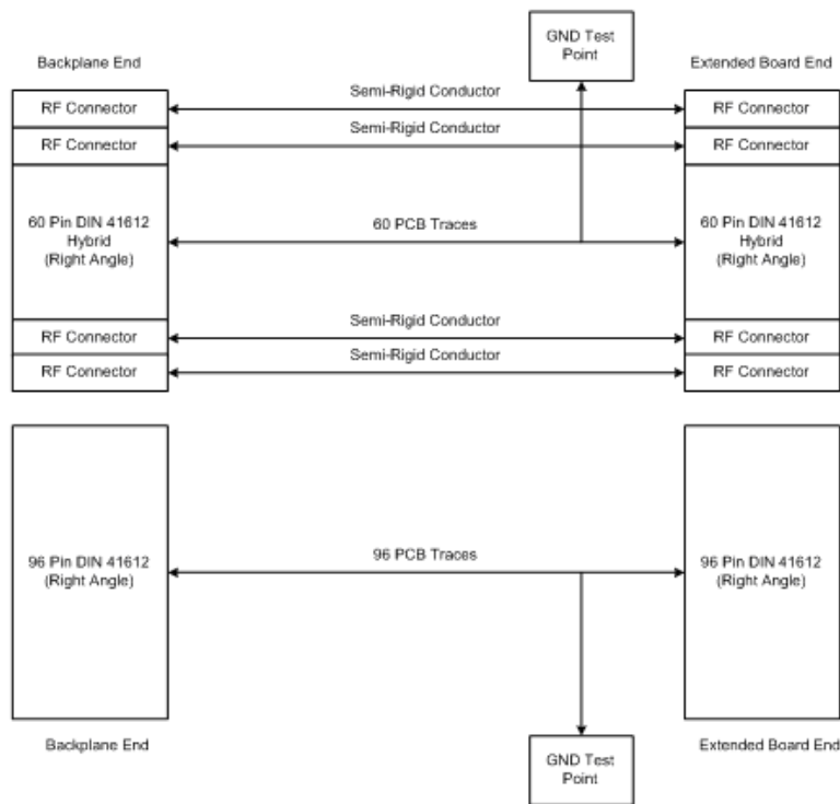
Figure 1-21 Extender Board
