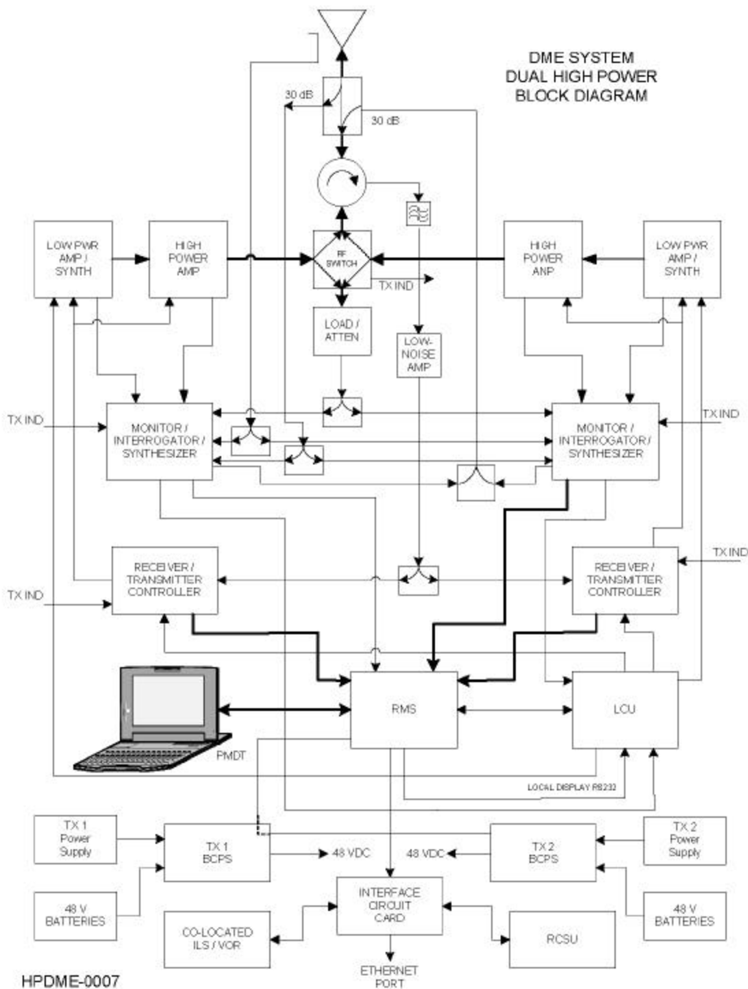
Figure 1-4 DME Simplified Block Diagram
