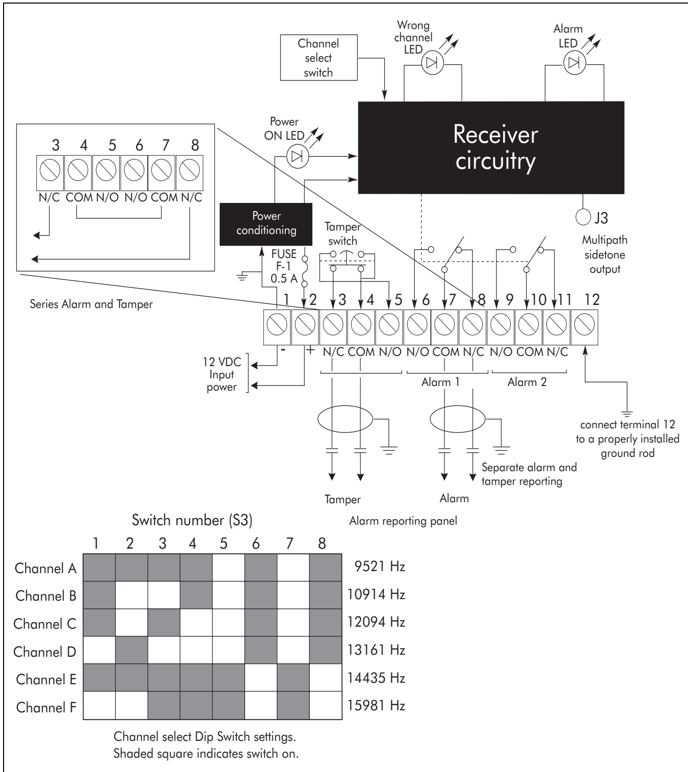
Figure 3-6: Receiver wiring
