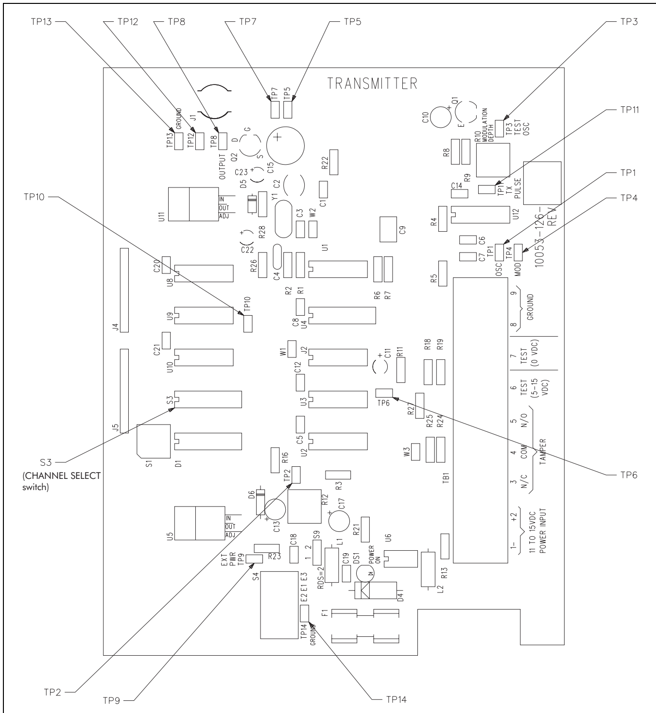
Figure 5-2: Transmitter PCB
