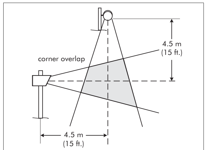
Figure 3: Corner overlap
