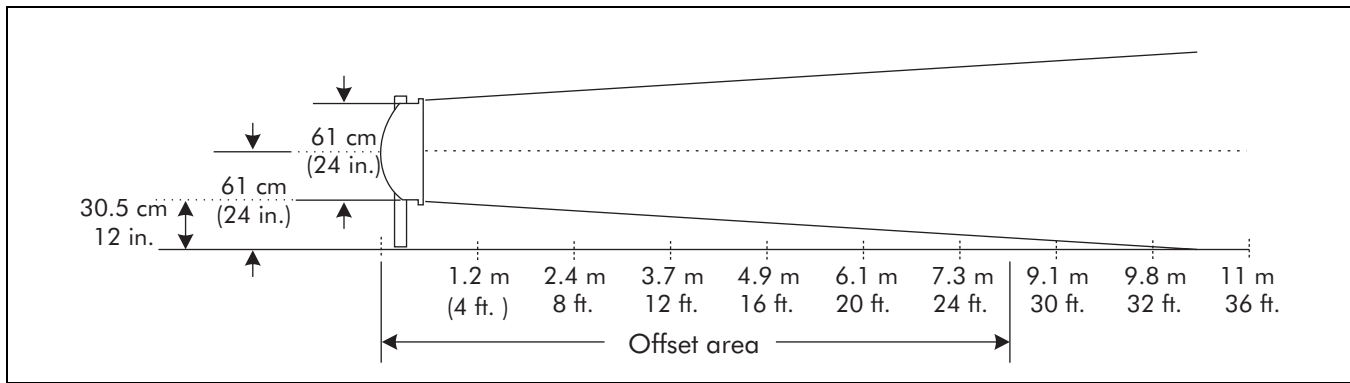
Figure 2-1: Offset area
