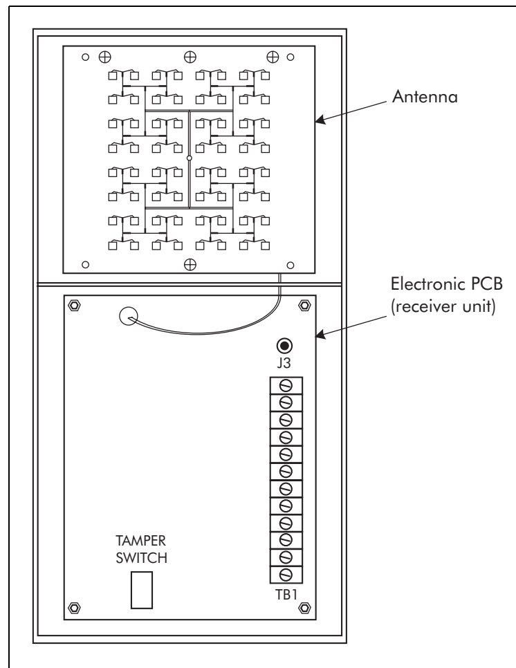
Figure 3-1: Series 24000 microwave unit (receiver)
