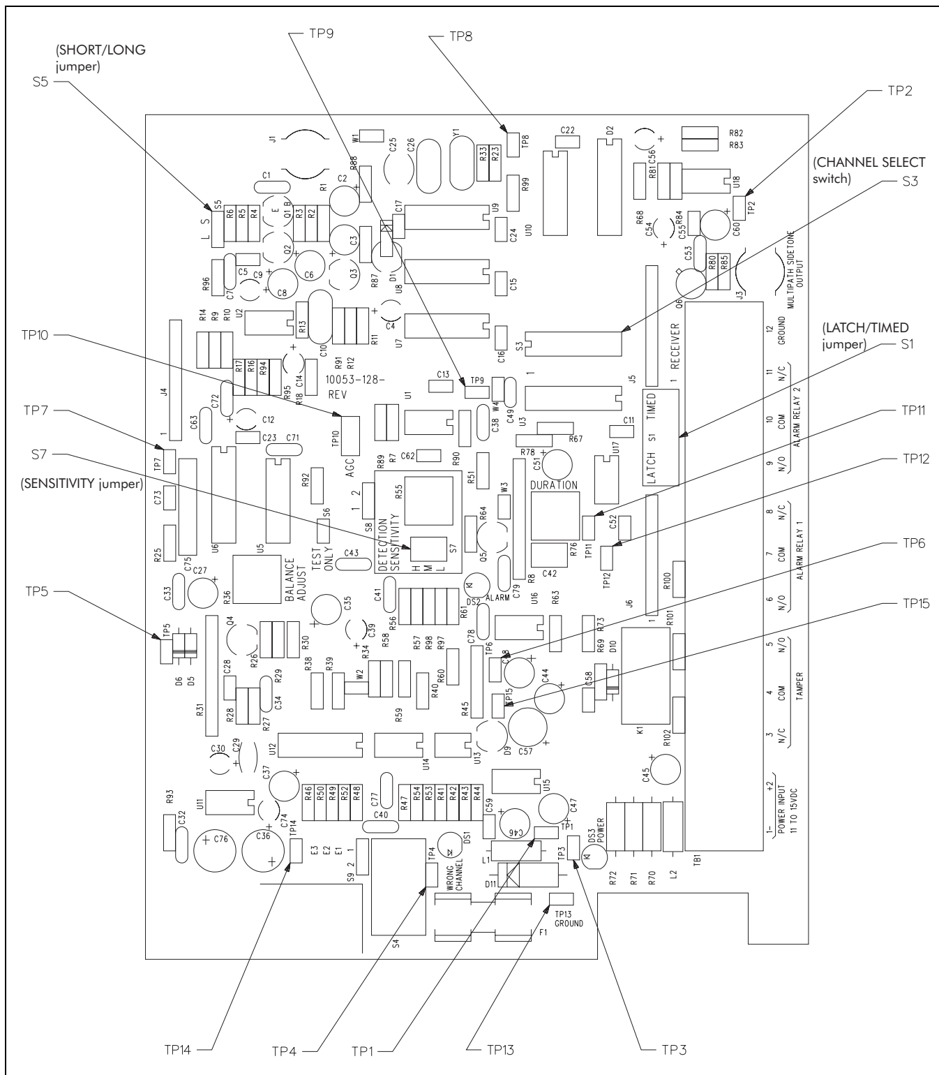
Figure 5-1: Receiver PCB
