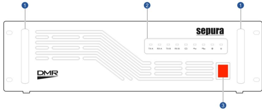
Front Panel
