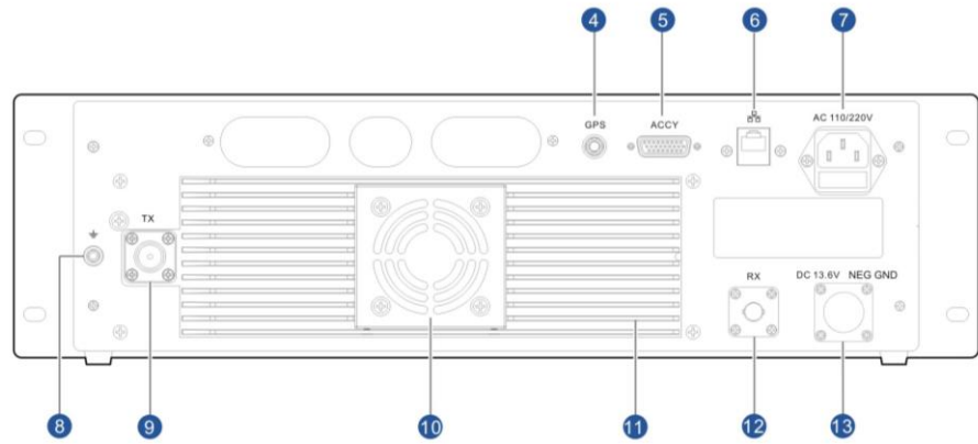
Rear Panel
