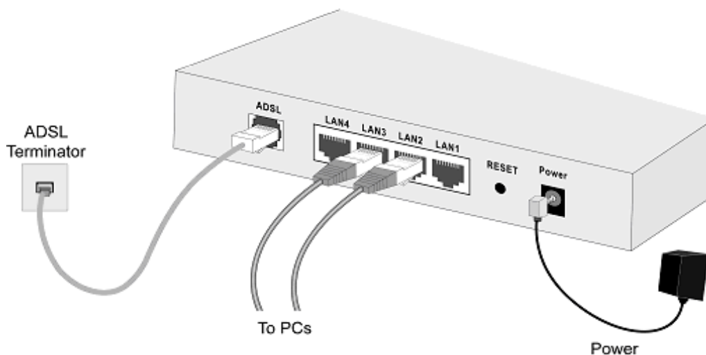
Figure 4: Installation Diagram
