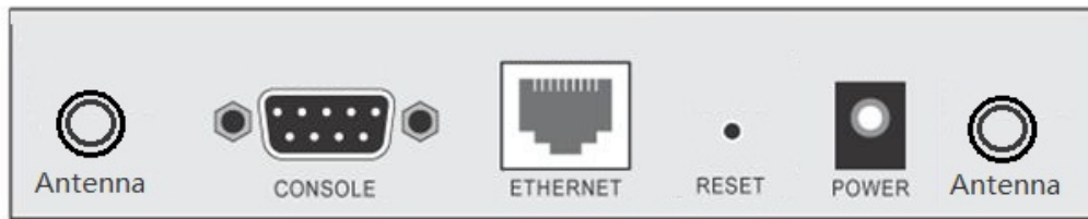
Figure 3: Rear Panel
