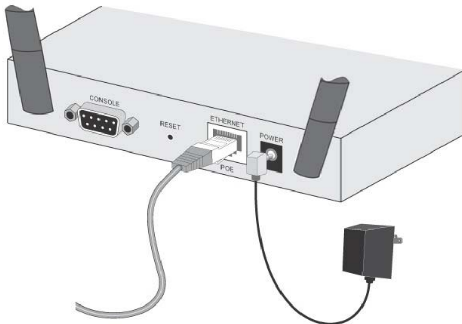
Figure 4: Installation Diagram
