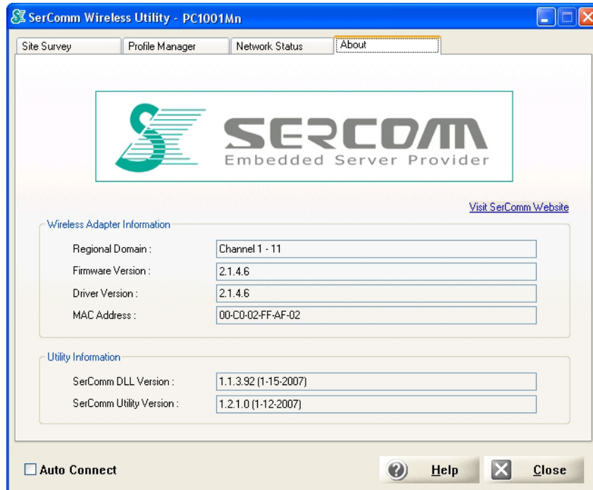
Figure 10: About Screen
