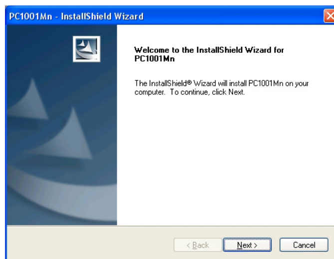
Figure 1: Start Installation
