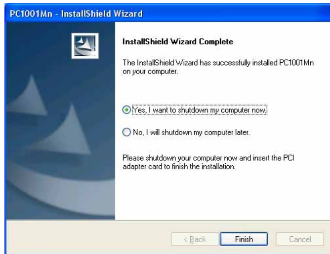
Figure 2: Installation Screen
