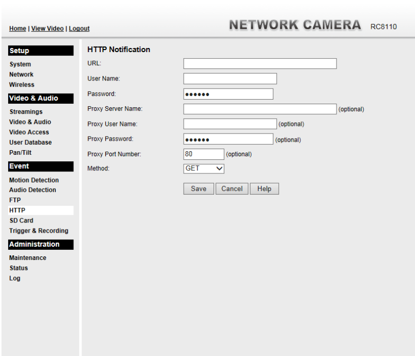
Figure 26: HTTP Screen
