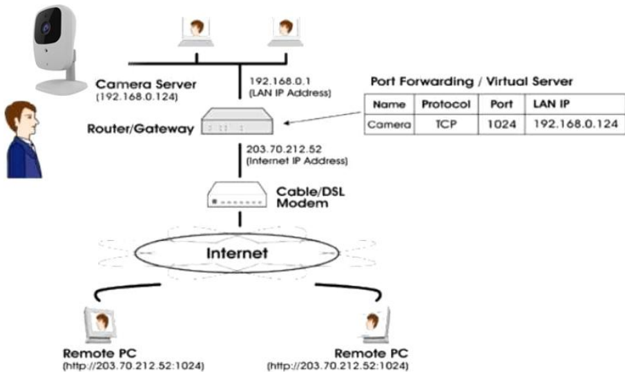
Figure 10: Connecting via the Internet
