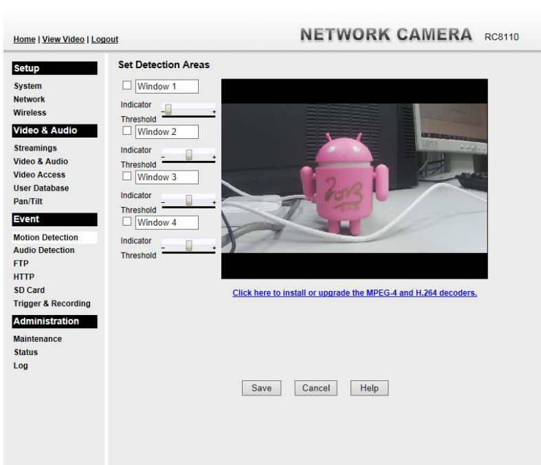
Figure 12: Motion Detection
