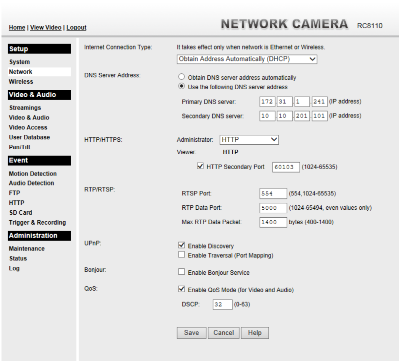
Figure 15: Network Screen
