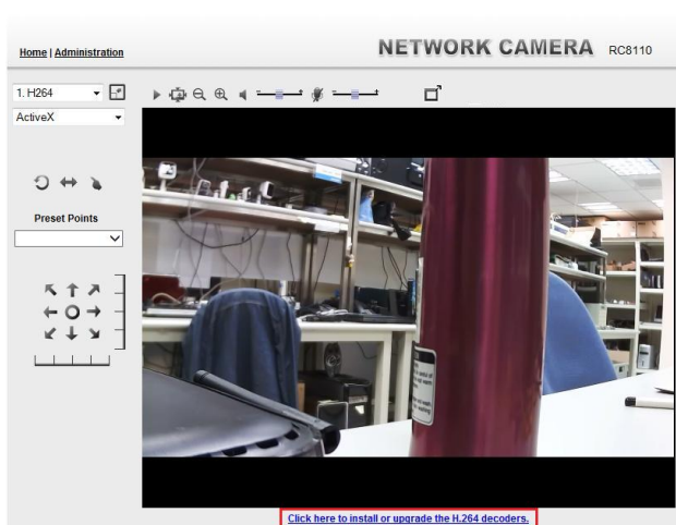
Figure 7: Install Decoders
