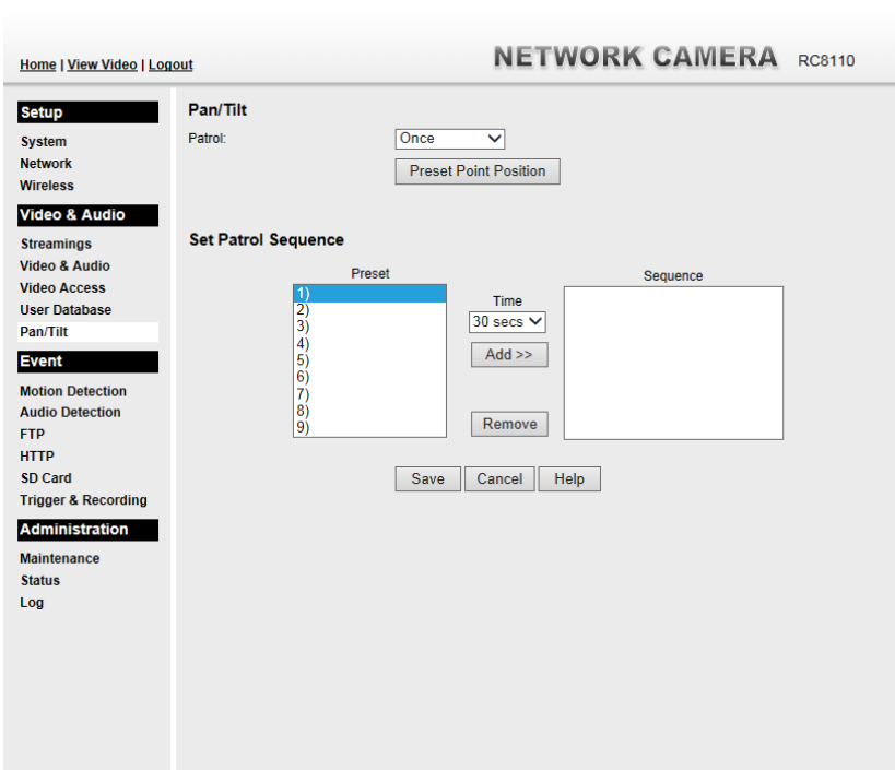
Figure 21: Pan/Tilt Screen
