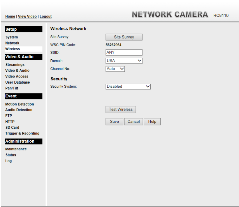
Figure 16: Wireless Screen
