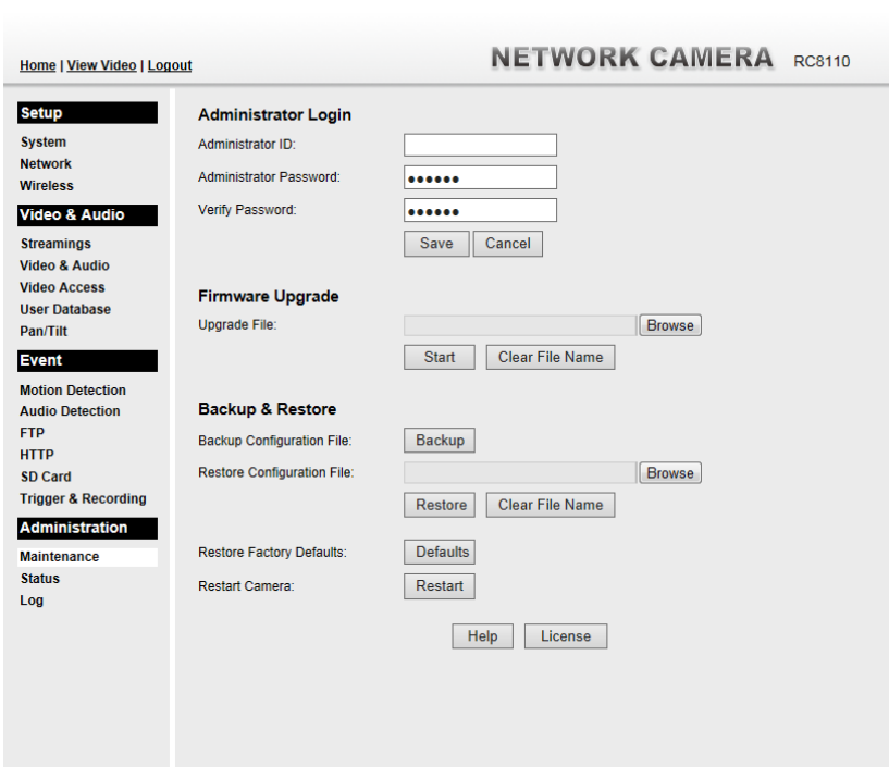
Figure 29: Maintenance Screen
