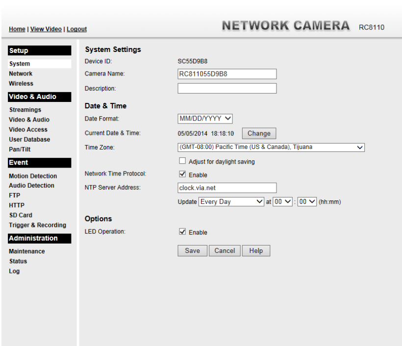
Figure 14: System Screen
