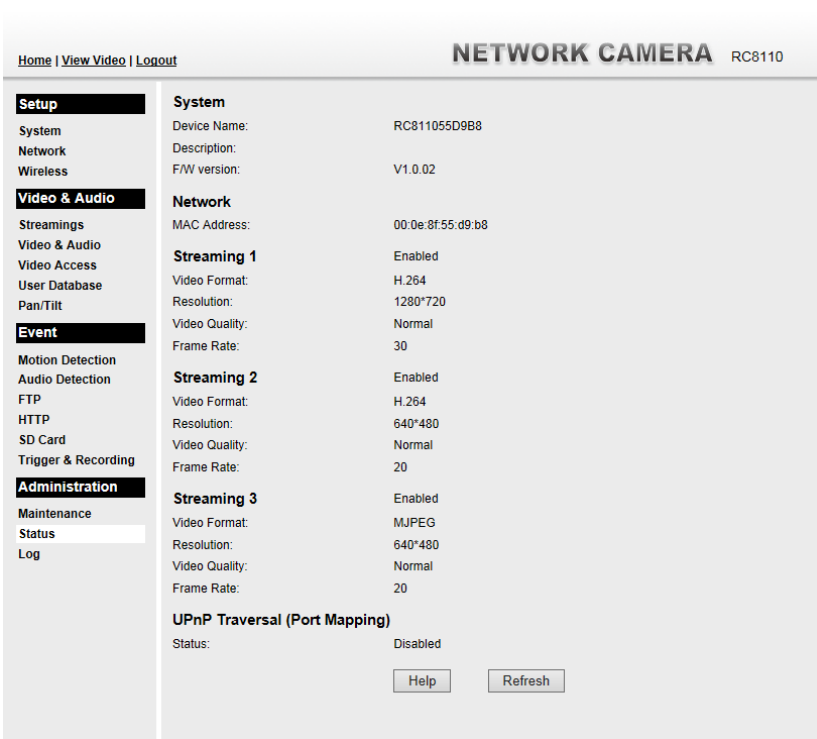
Figure 30: Status Screen
