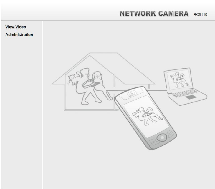
Figure 13: Welcome Screen
