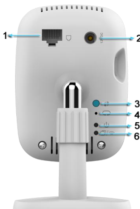
Figure 3: Rear Panel
