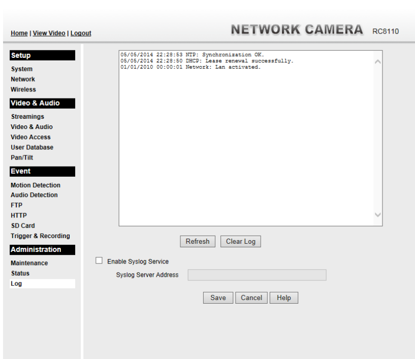
Figure 31: Log Screen
