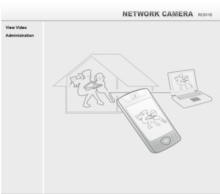
Figure 4: Home Screen
