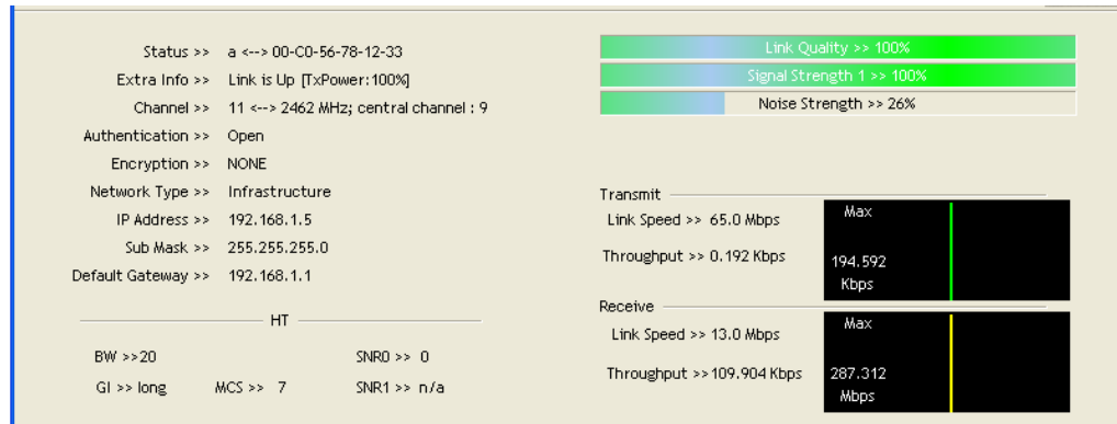
Figure 10: Link Status
