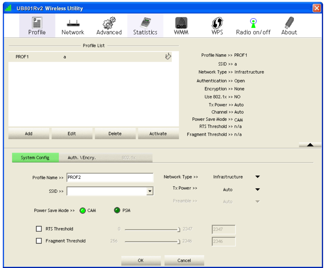
Figure 10: Profile Screen
