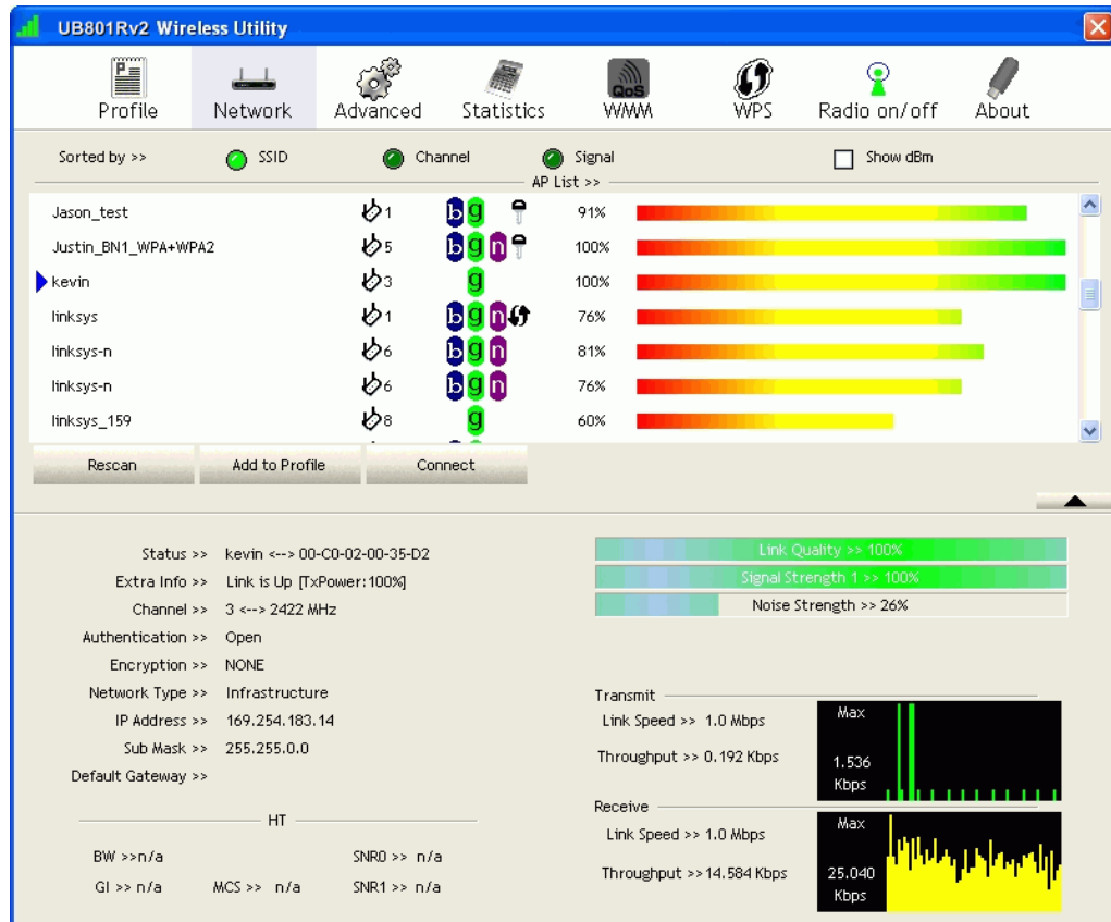
Figure 7: Network Screen
