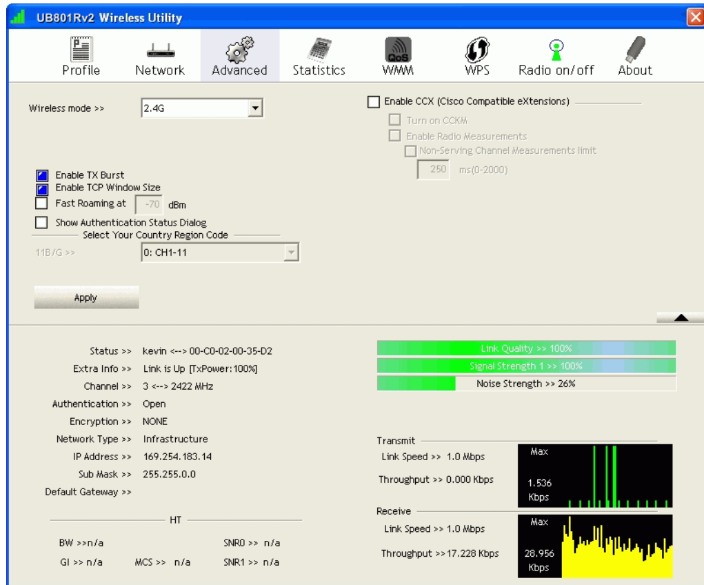
Figure 9: Advanced Screen
