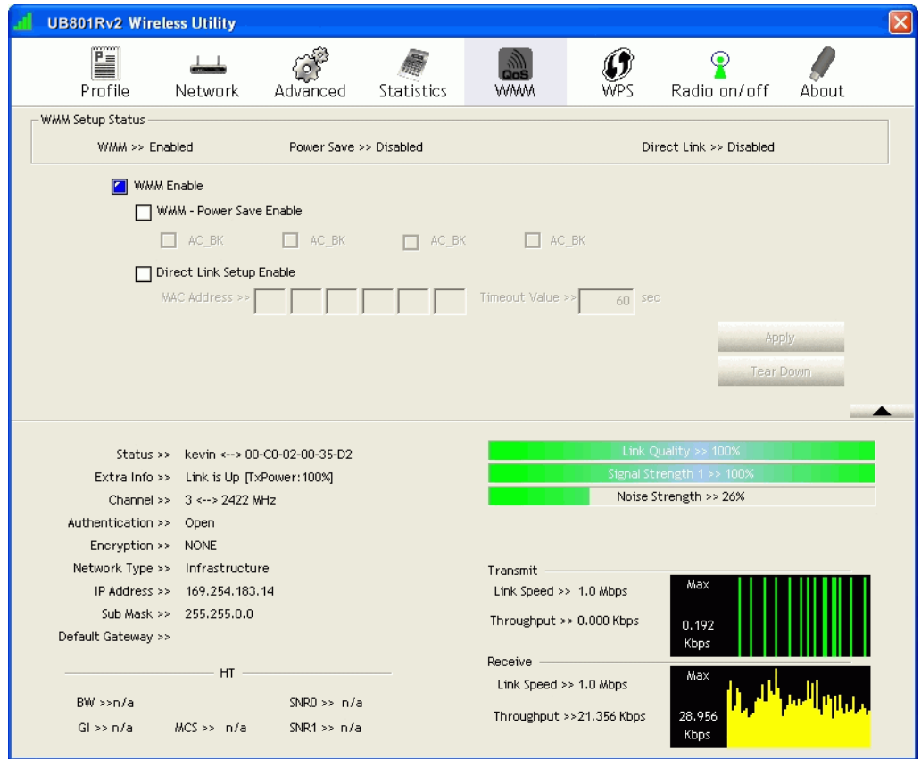
Figure 11: WMM Screen
