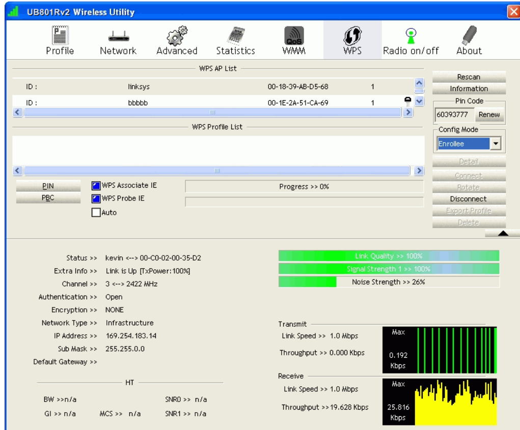
Figure 12: WPS Screen
