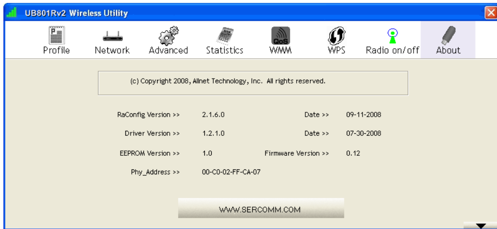
Figure 14: About Screen
