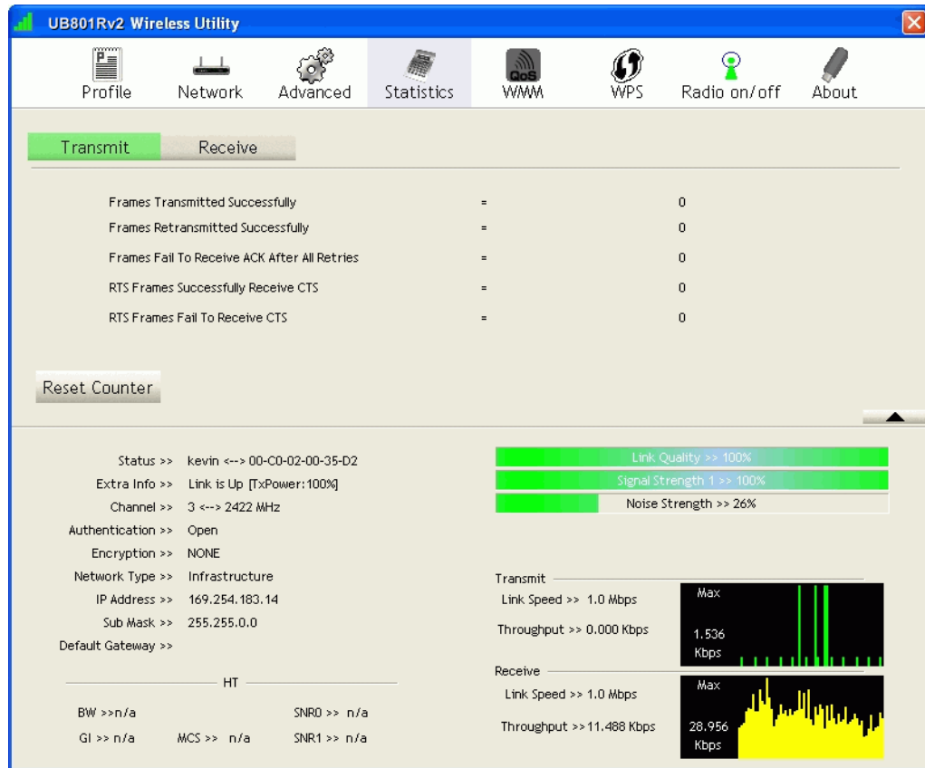
Figure 10: Statistics Screen
