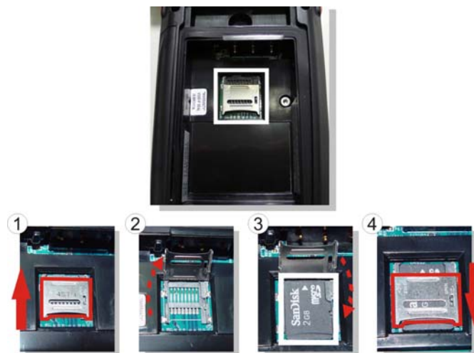
Figure 2-19 Detach the SD Holder from Device
