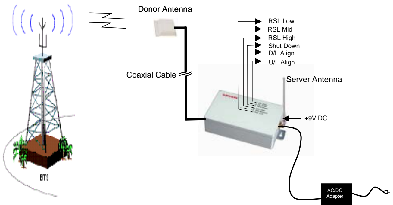
Figure 4.0 : Installation Diagram of Home Booster
