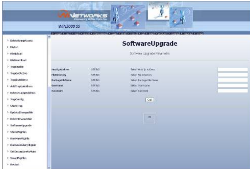
Figure 6-1: SoftwareUpgrade Screen
