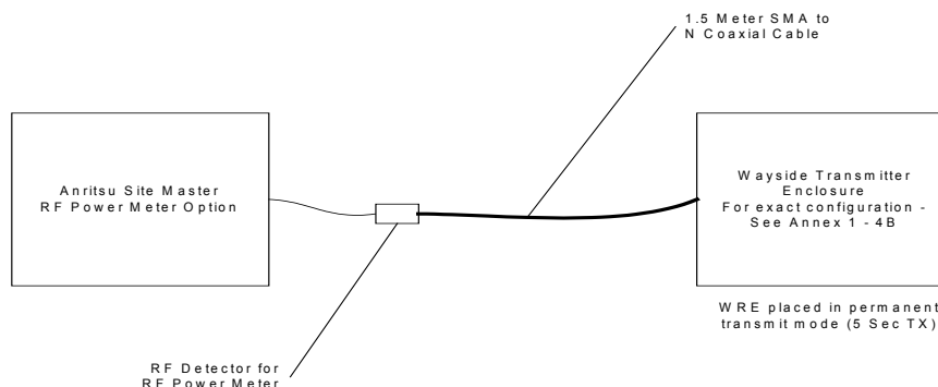
Figure 5.3 - RF Measurement of WRE
