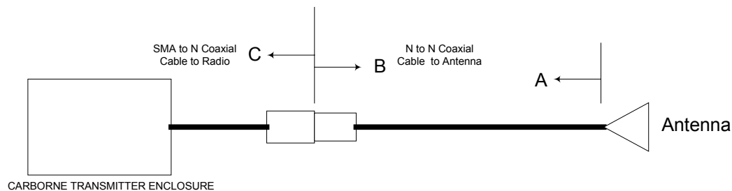
Figure 6-1 - Carborne Power Measurements
